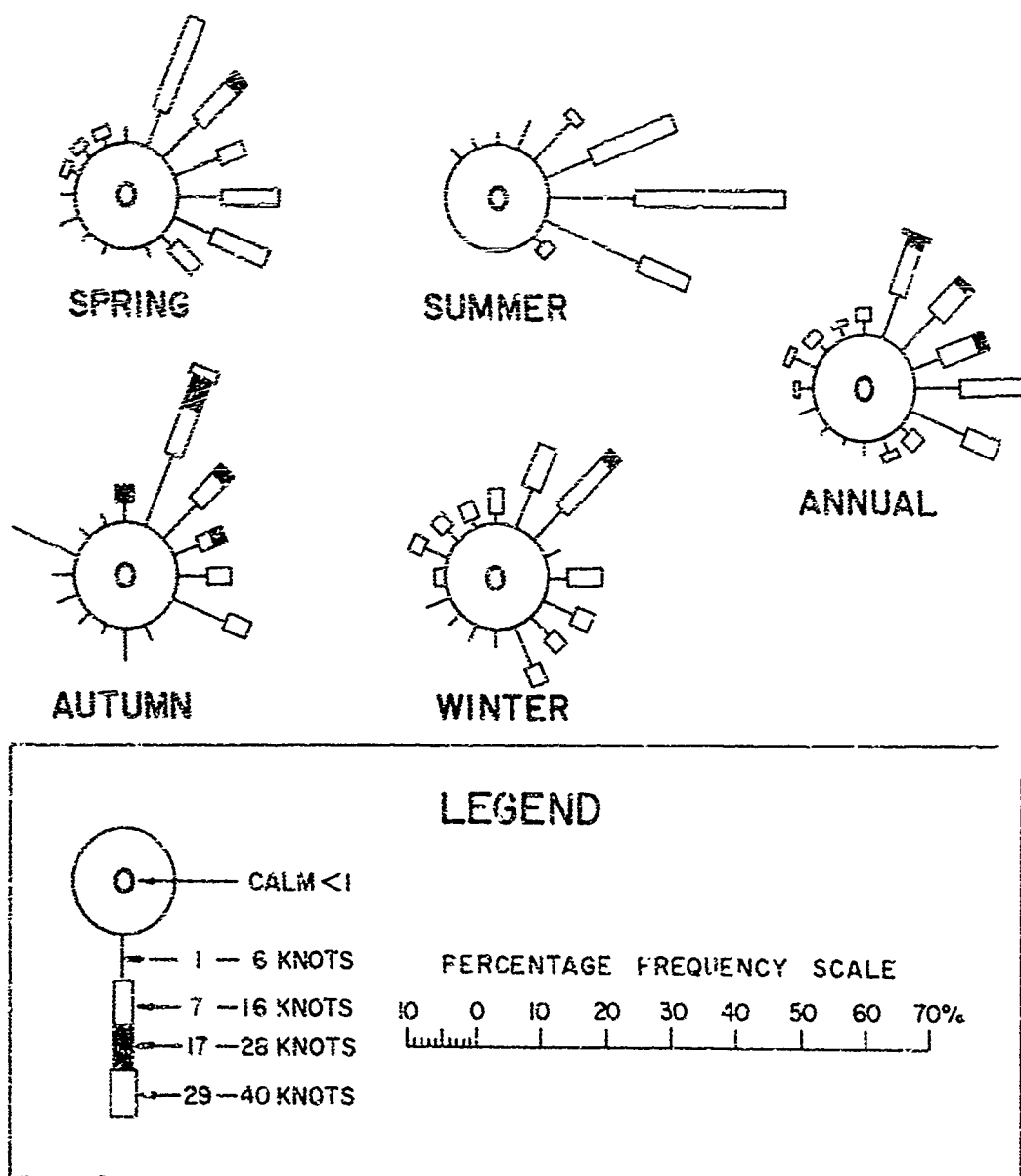
FIGURE 3. SEASONAL AND ANNUAL WIND ROSE AT MANGROVE CAY, ANDROS ISLAND, NOV. 1962 THROUGH OCT. 1964.
