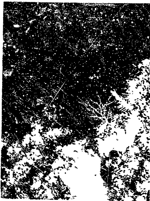
PLATE 3. FRESH CREEK (A) ONE OF THE BLIND CHANNELS IN THE ZONE OF LUXURIANT CORAL GROWTH BETWEEN 40 TO 60 FEET DEPTH, (B) OUTER PLATFORM, DEPTH 110 TO 130 FEET, (C) DETAILED VIEW OF OUTER PLATFORM SHOWING HARD BOTTOM AND THIN SAND VENEER, (D) VERTICAL DOWNWARD VIEW OF EDGE OF OUTER PLATFORM AT 130 FEET. NOTE TERRACE TO RIGHT OF PHOTOGRAPH APPROXIMATELY 15 FEET DEEPER.
