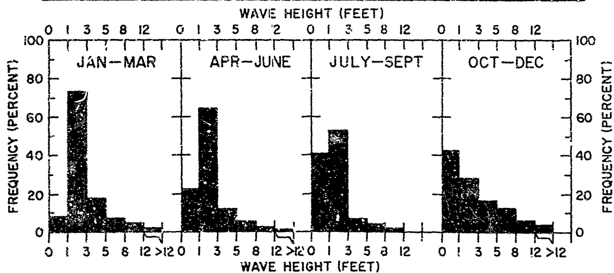
FIGURE 4. OBSERVED SEASONAL WAVE HEIGHTS, DIRECTION AND FREQUENCY IN THE TONGUE OF THE OCEAN.
