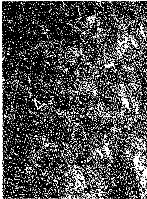
PLATE 9. BIG WOOD CAY (A) LAGOON BOTTOM BETWEEN BUOYS 1 TO 4, DEPTH 4 FEET (LOW TIDE), (C) & (D) LAGOON BOTTOM AT BUOY 5, DEPTH 5 FEET. ROUNDED CORAL (DIPLORIA CLIVOSA) IS 1 FOOT ACROSS.
