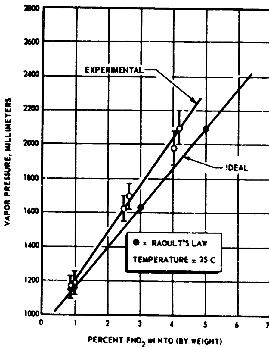
Figure 5. Vapor Pressures of NTO- \text{FNO}_2 Solutions. 25 \pm 0.5^\circ\text{C}
