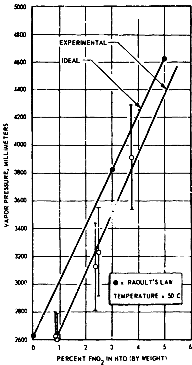
Figure 6. Vapor Pressures of \text{NTO-FNO}_2 Solutions, 50°C
