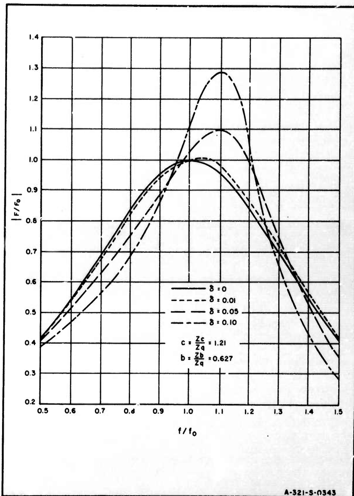
FIG. 16a MECHANICAL RESPONSE OF Y-CUT TRANSDUCER WITH INDIUM BOND TO FUSED-SILICA DELAY MEDIUM
