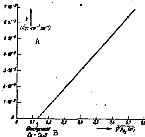
Fig. 5. Tarnishing constant k for the oxidation of copper to copper protoxide at 1000°C as a function of the seventh root of the oxygen pressure ( P_{O_2} in atm). A) Equilibrium.
