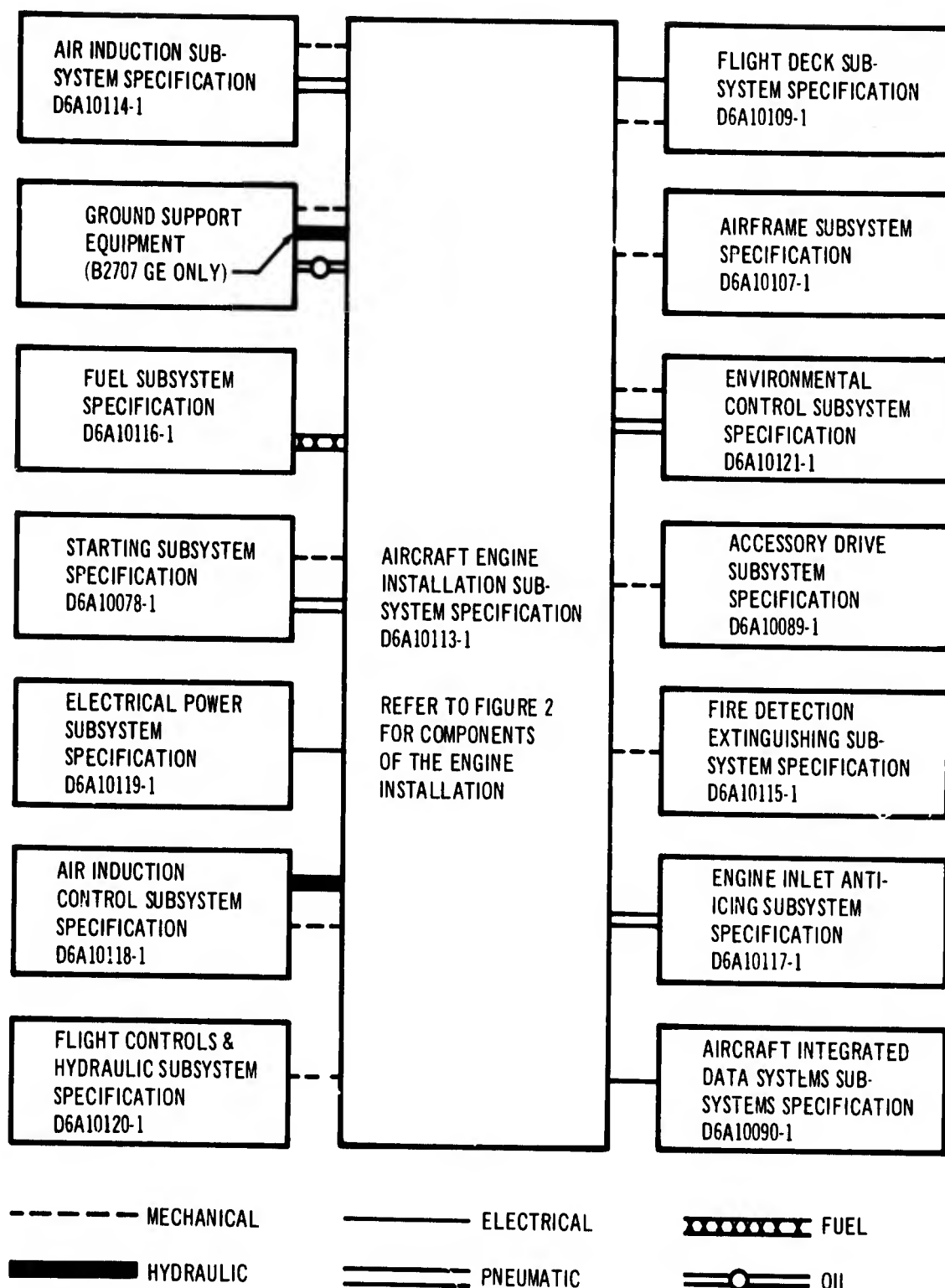
Figure 1. Interface Diagram
