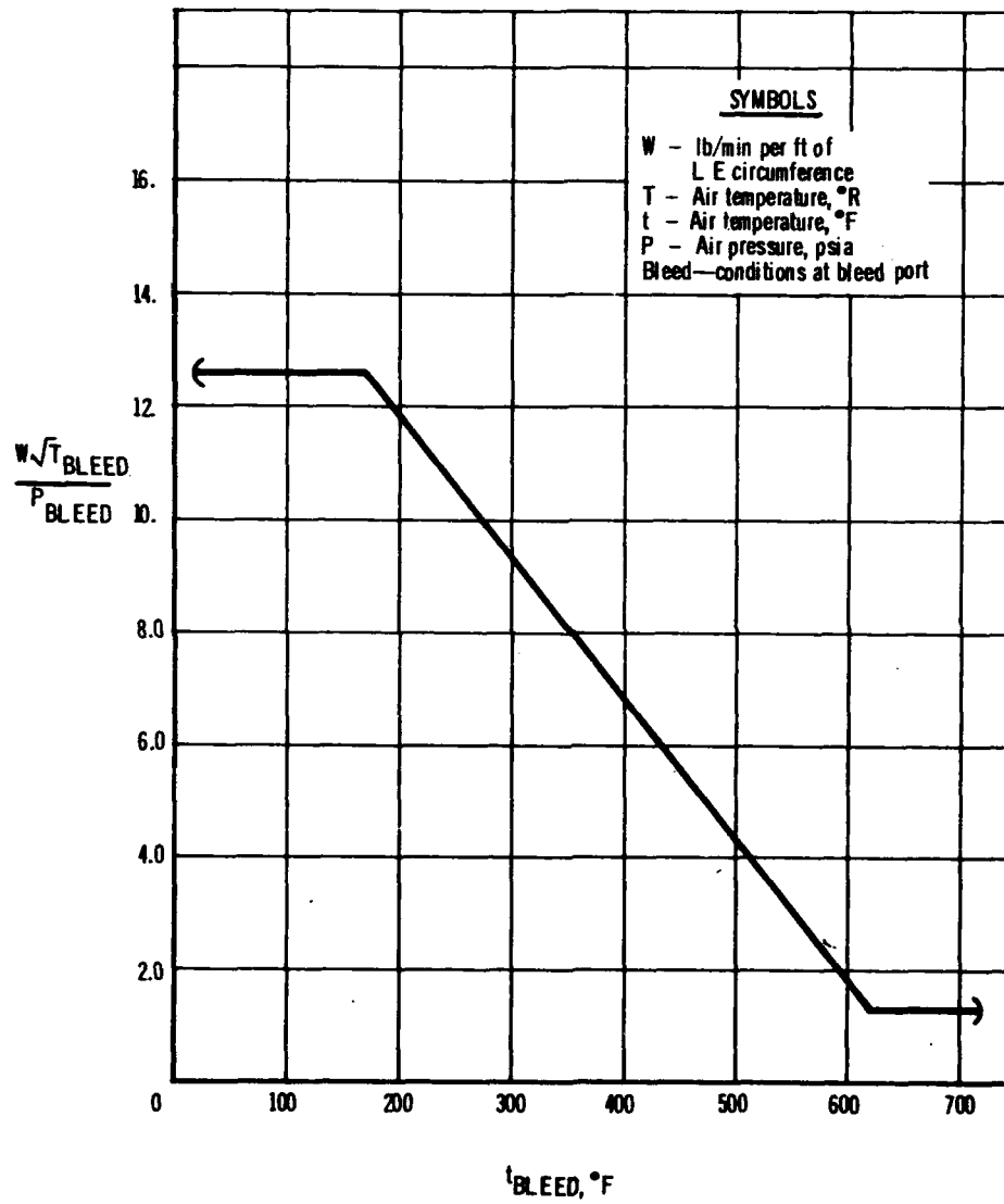
Figure 4. IAIS Total Airflow Requirements for B-2707 (G.E.)
