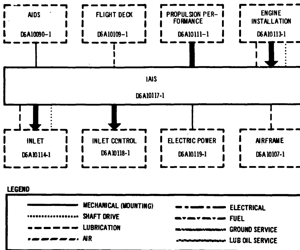
Figure 3. Interface Schematic Diagram—B-2707 (P&WA)
