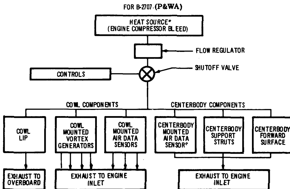
Figure 6. IAIS Design Features
