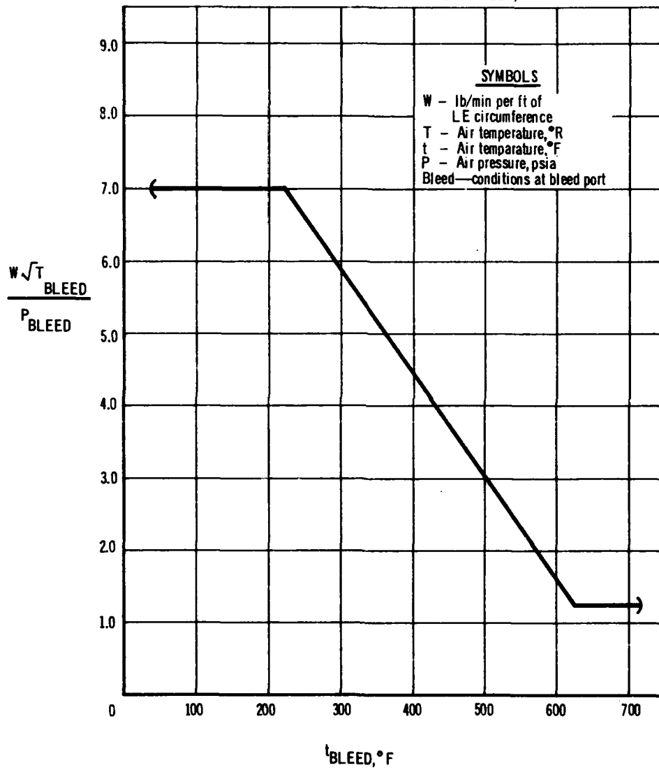
Figure 5. IAS Total Airflow Requirements for B-2707 (P&WA)
