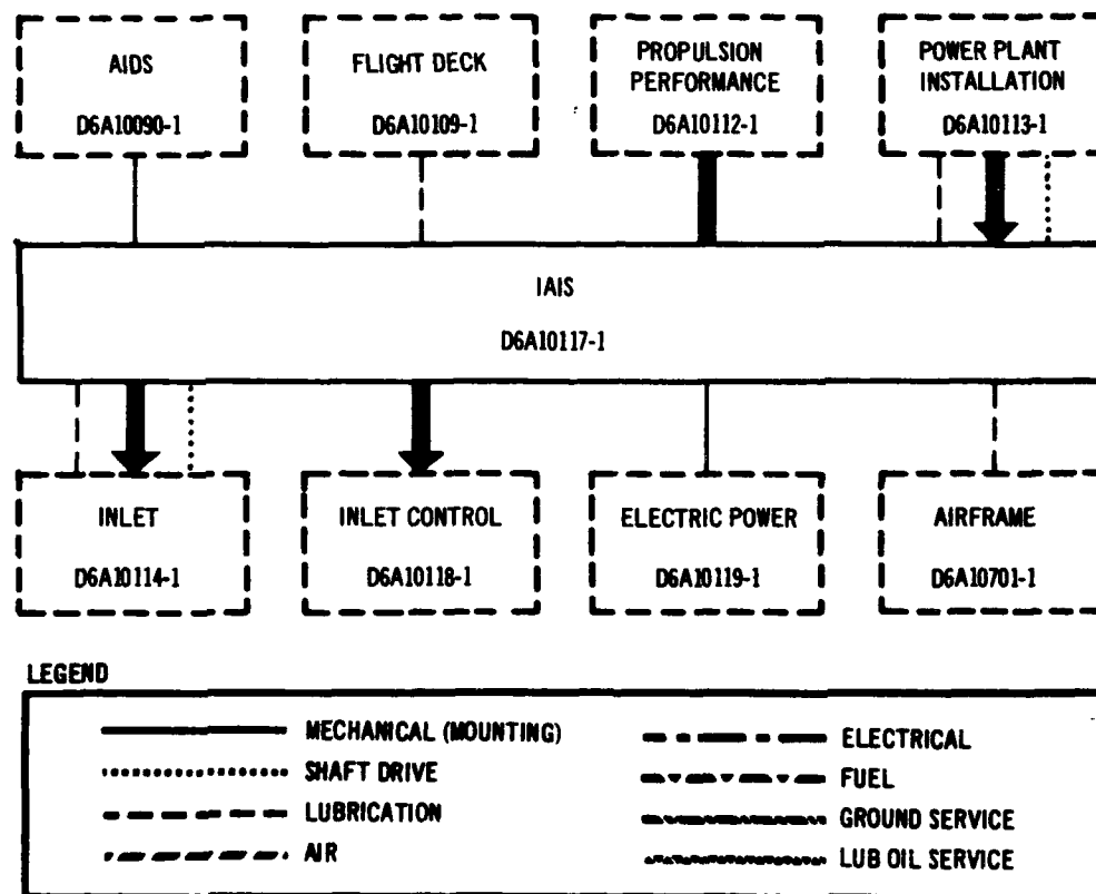
Figure 2. Interface Schematic Diagram—B-2707 (G.E.)
