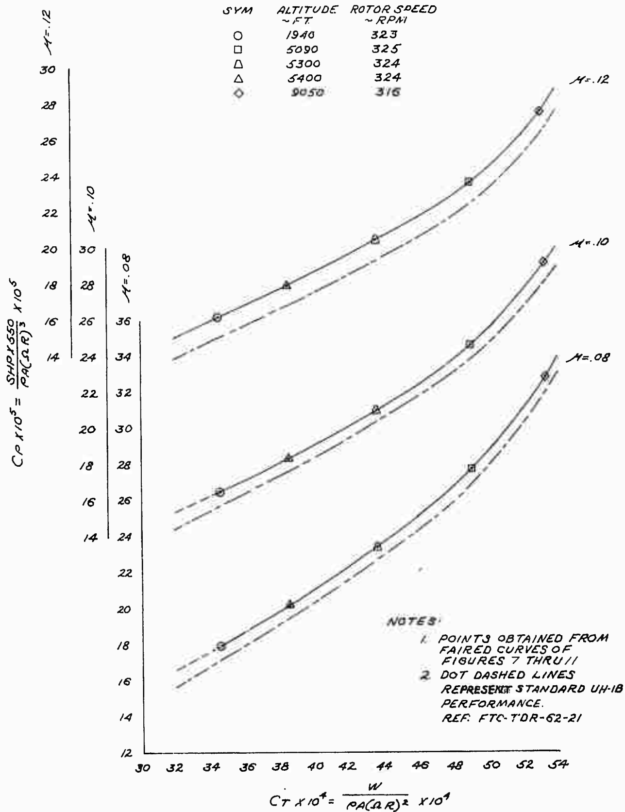
FIGURE No. 4 NON-DIMENSIONAL LEVEL FLIGHT PERFORMANCE UH-1B USA 5/160-3548 FLOAT KIT INSTALLED
