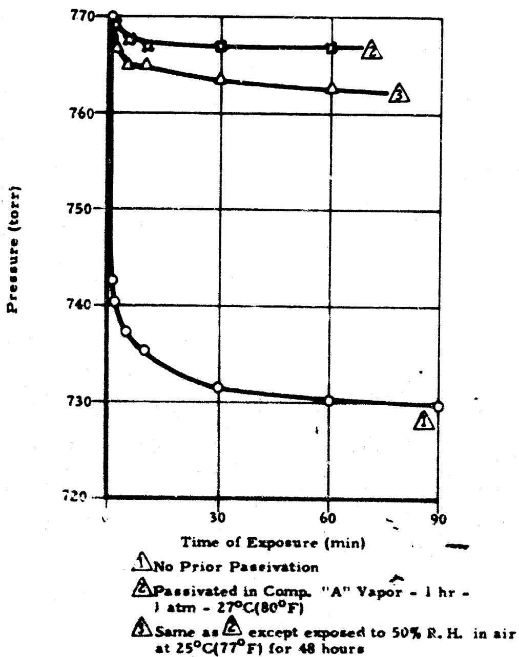
Figure 36. Exposure of Nickel 200 Powder (80g) to Fluorine at 27°C(80°F)
