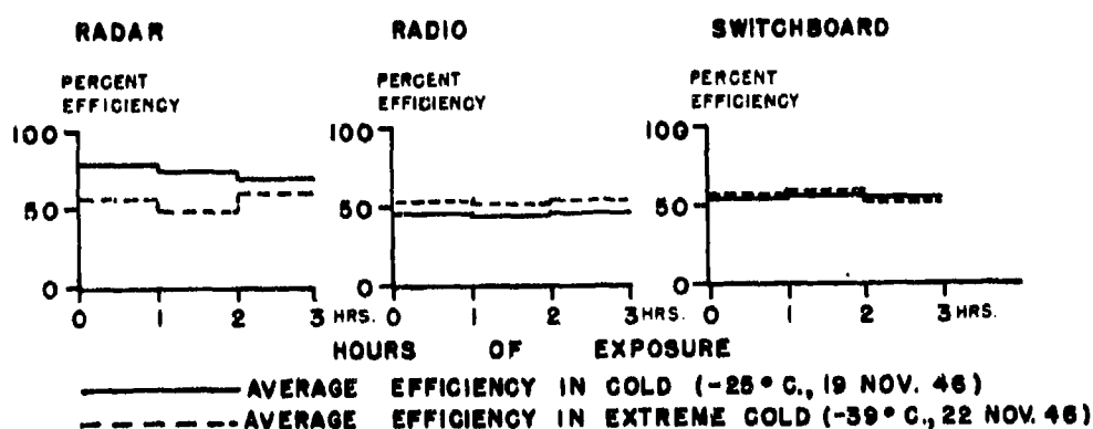
FIGURE 3 EFFECT OF AMBIENT TEMPERATURE ON EFFICIENCY
