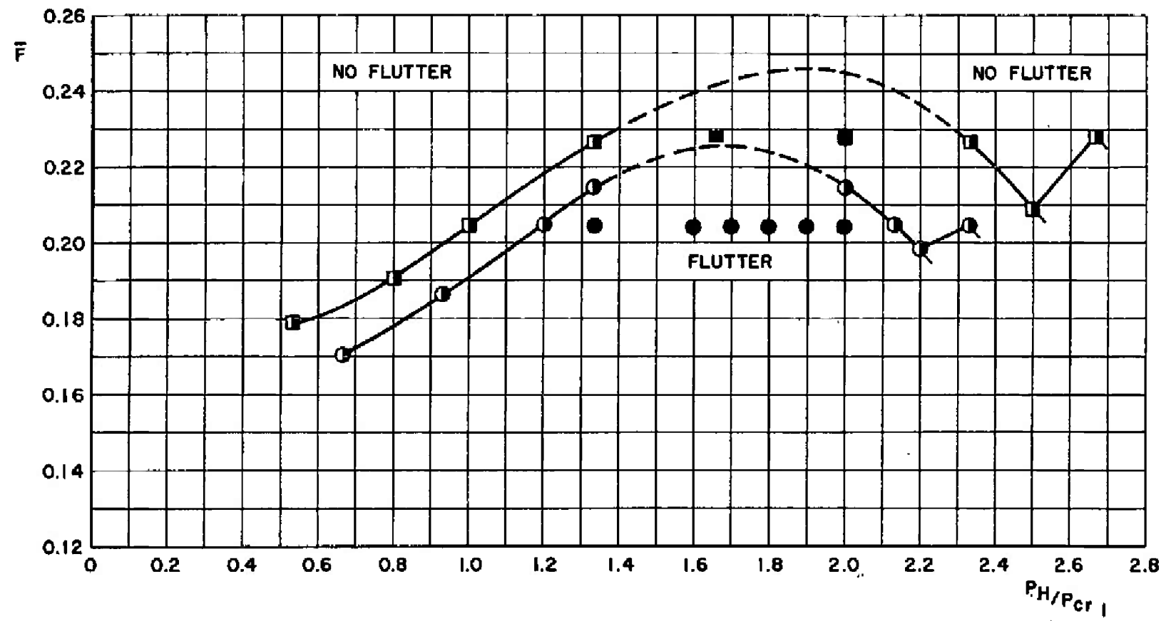
Fig. 16 Variation of the Flutter Parameter with Panel Buckling Load Ratio at M_{\infty} = 1.40
