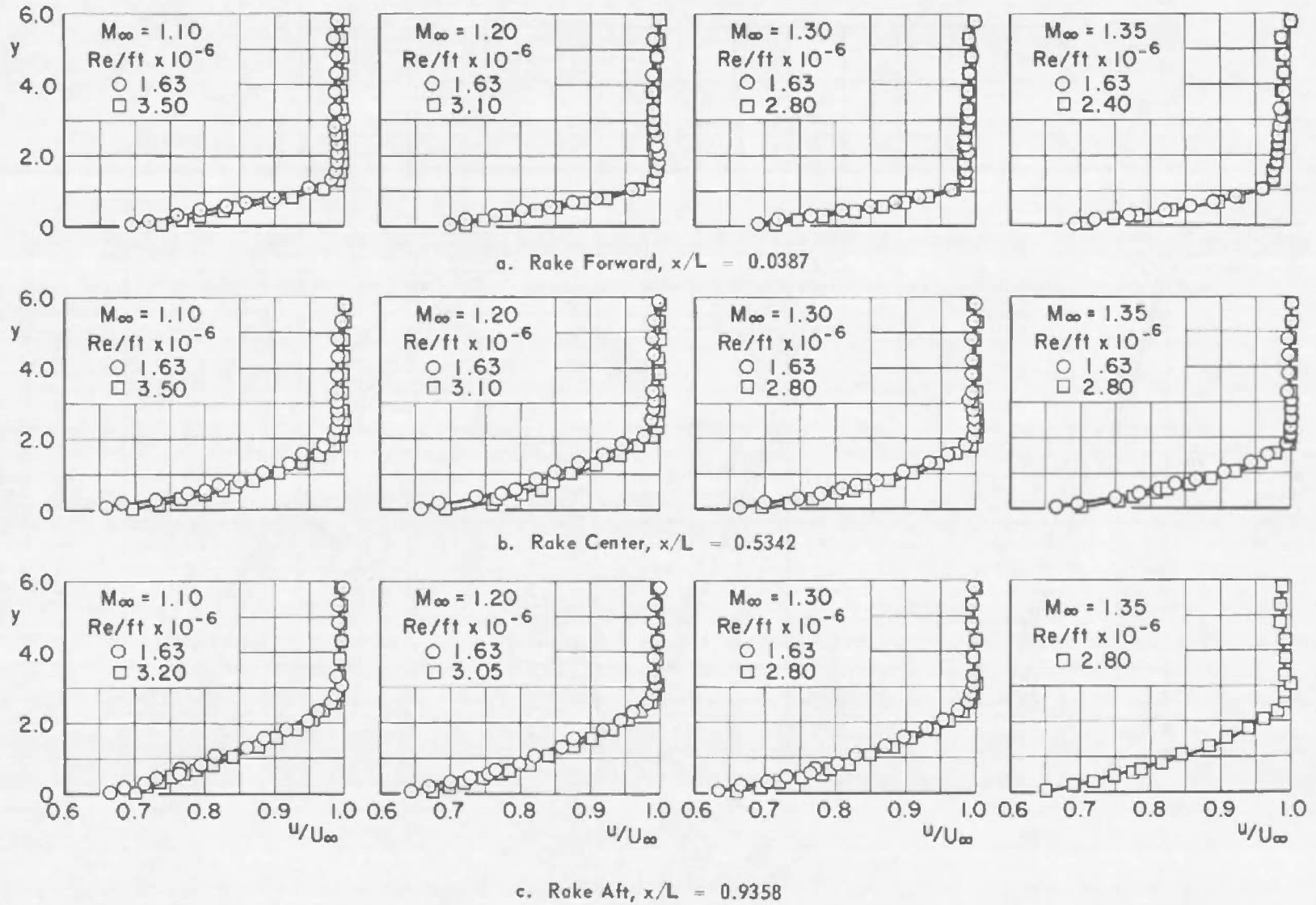
Fig. 10 Boundary-Layer Profiles
