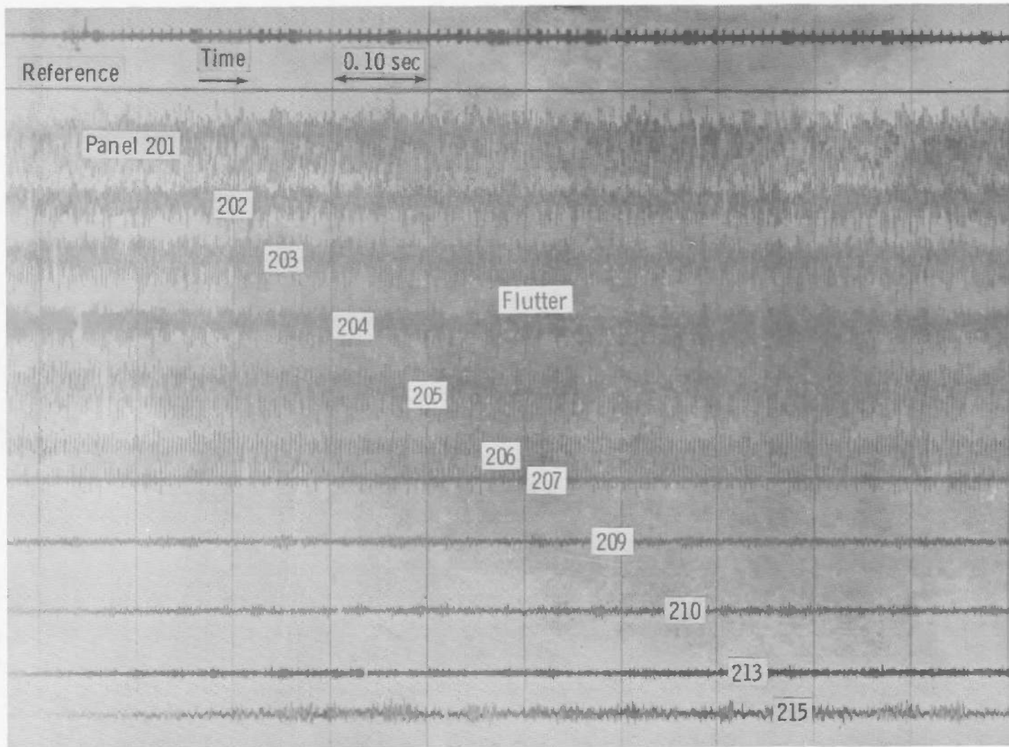
Fig. 15 Oscillograph Trace Showing Panel Flutter
