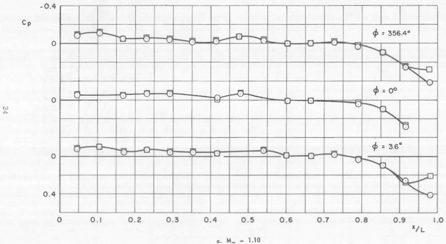
Fig. 12 Variation of Pressure Coefficients along the Pressure Panel
