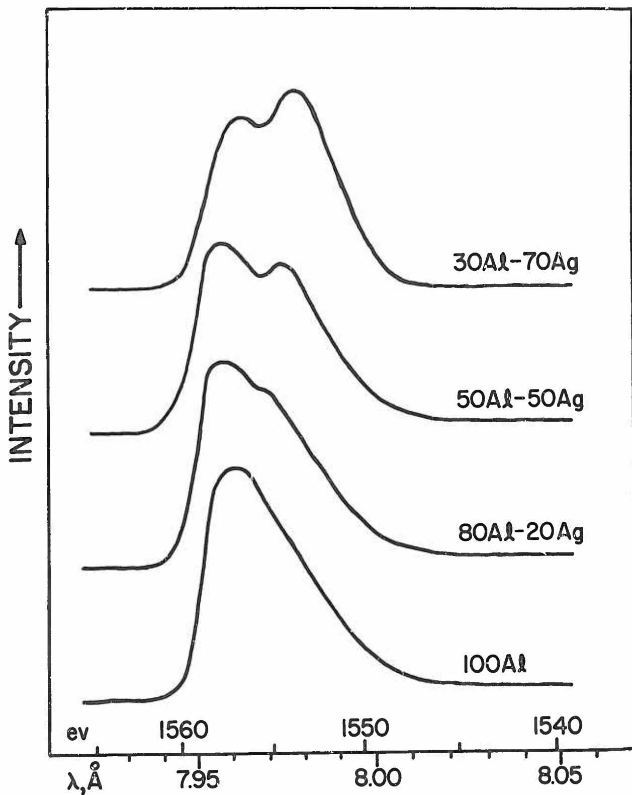
Figure 33. Aluminum K Emission Band from Some Al-Ag Alloys (EDDT Crystal)
