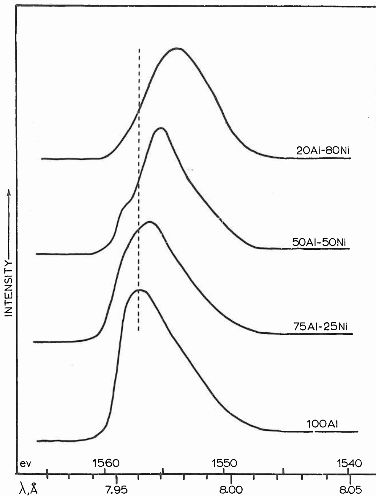
Figure 11. Aluminum K Emission Band from Some Al-Ni Alloys (EDDT Crystal)
