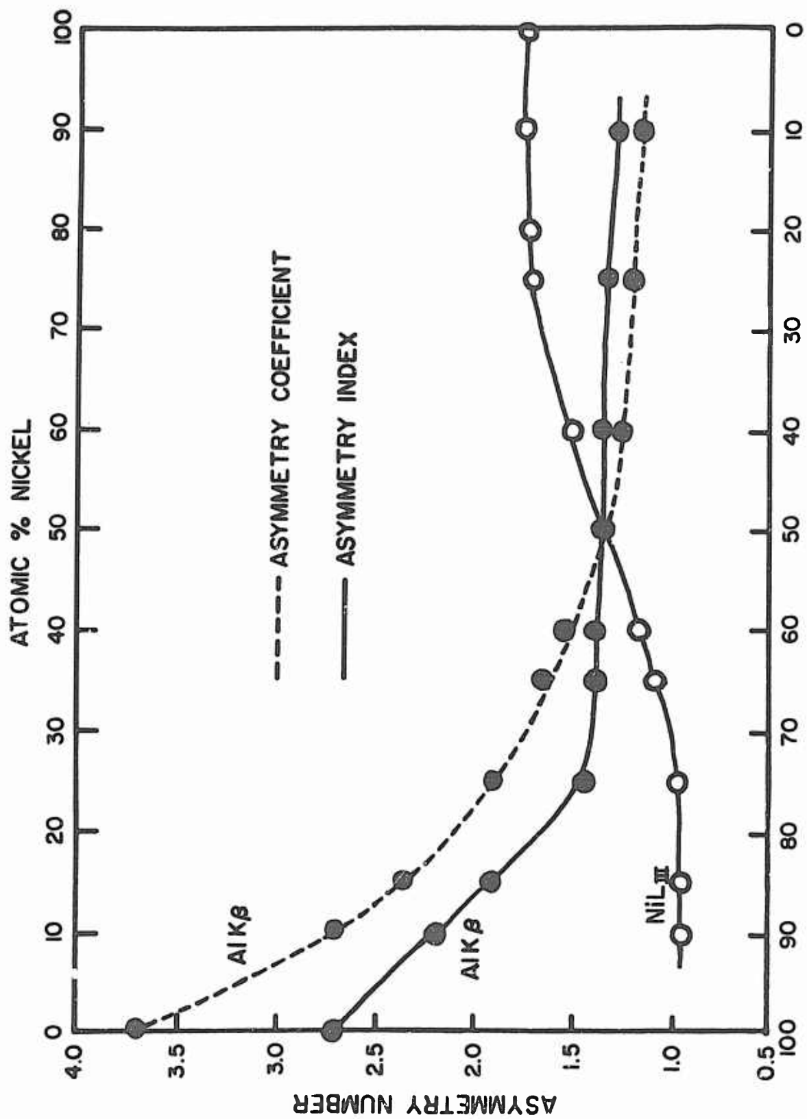
Figure 15. Change in Asymmetry Constants of Al K and NiL \beta Bands with Alloy Composition in Al-Ni System
