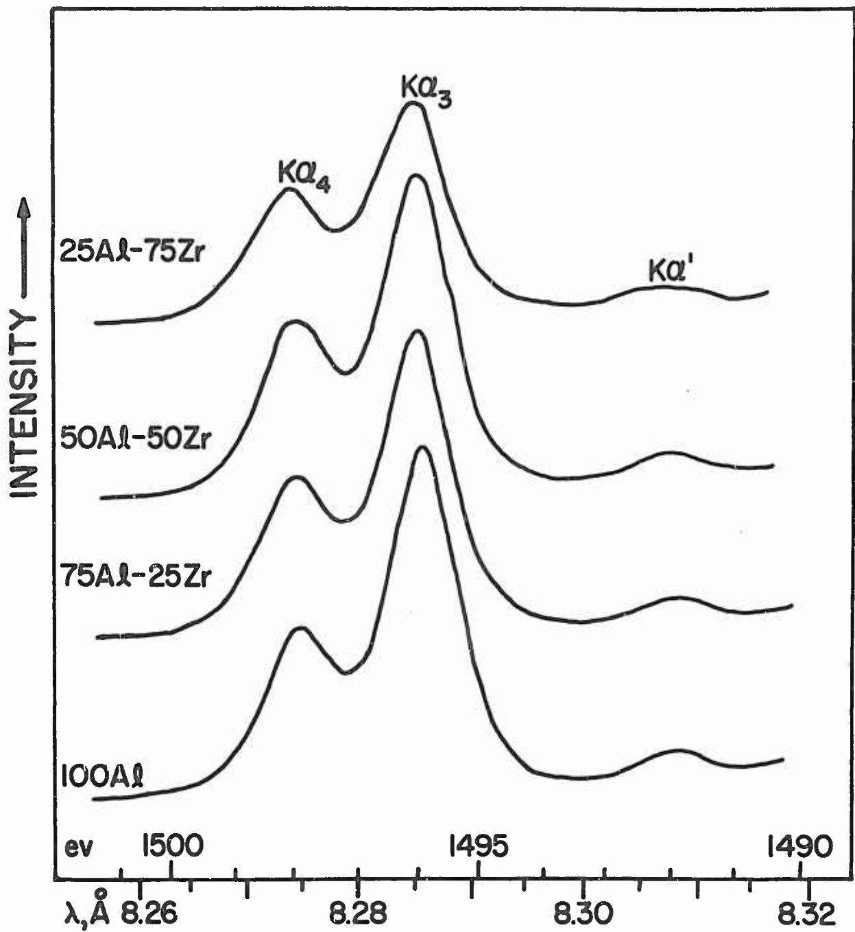
Figure 44. Aluminum K\alpha' , K\alpha_3 and K\alpha_4 Lines from Some Al-Zr Alloys (EDDT Crystal)
