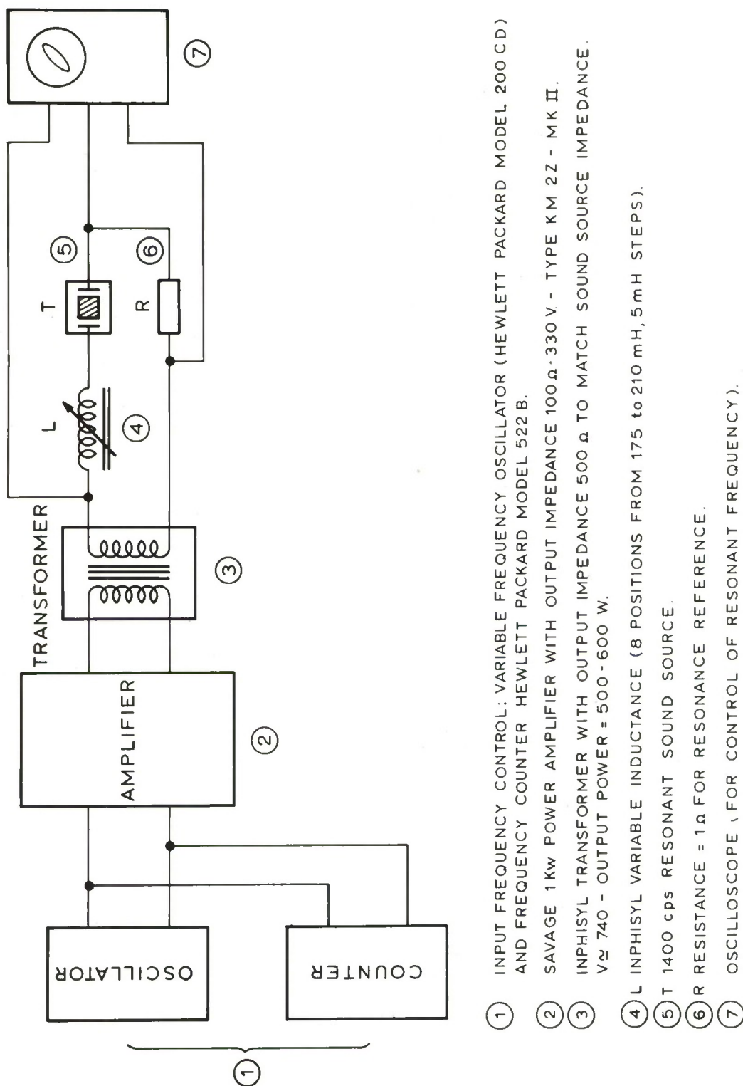
Fig. 5 Driving Unit for Shipborn Source
