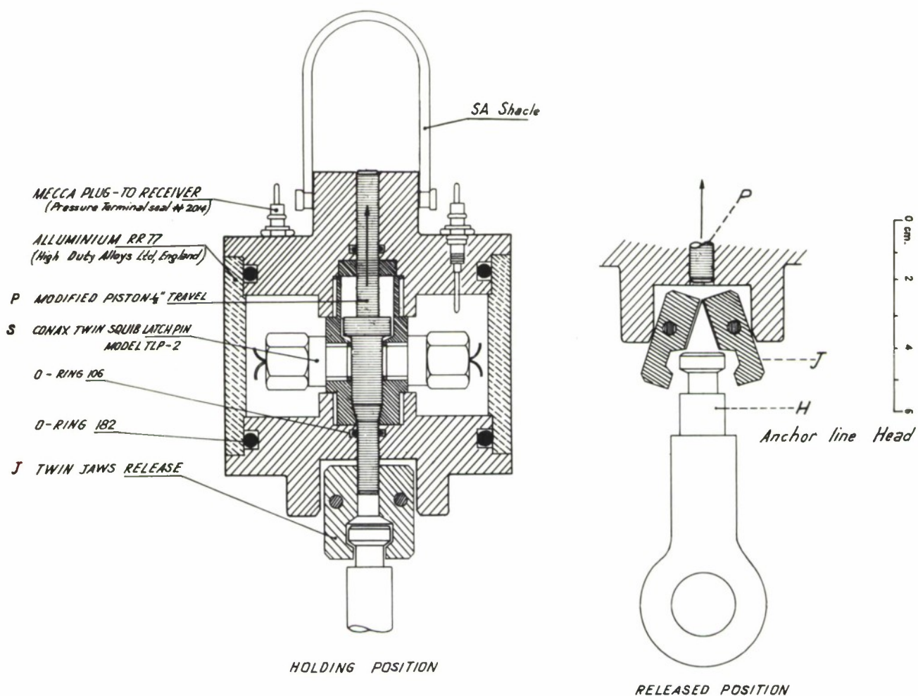
Fig. 9 Mechanical Releaser
