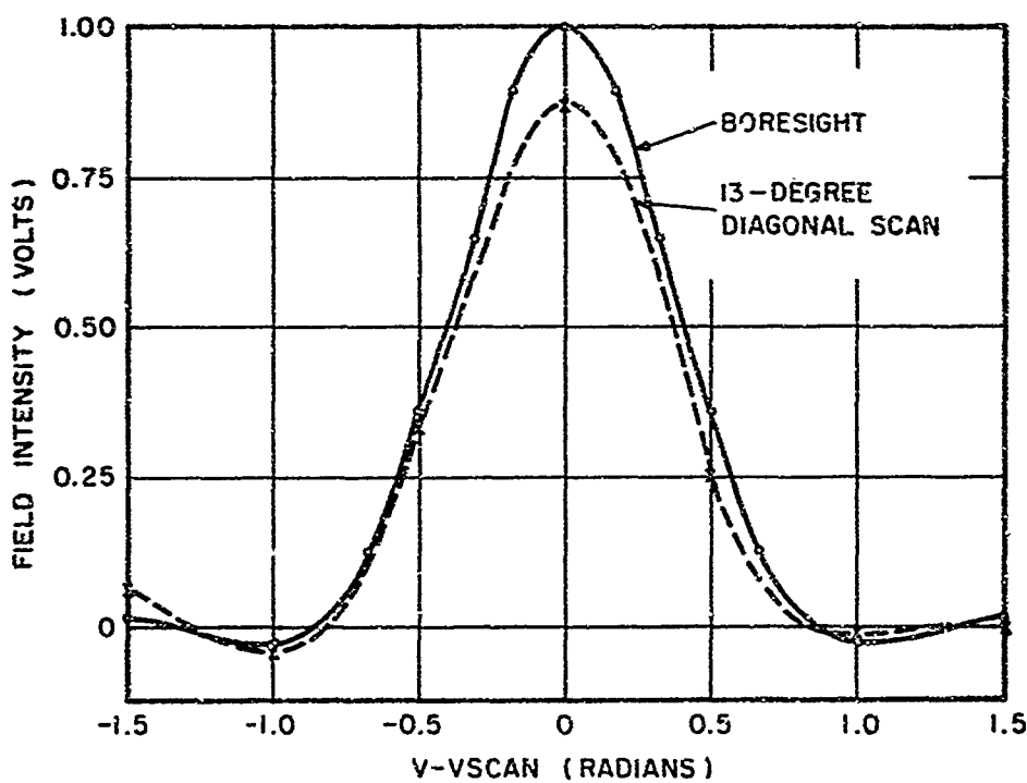
FIGURE 4. PRINCIPAL PLANE PATTERNS FOR 1.5-WAVELENGTH SPACING, APERTURE OF 15 \times 15 WAVELENGTH
