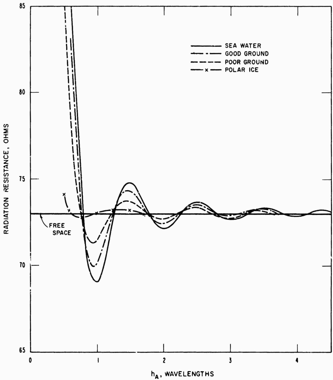
6. Radiation resistance of a vertical half-wave dipole over various types of ground as a function of height of the midpoint.
