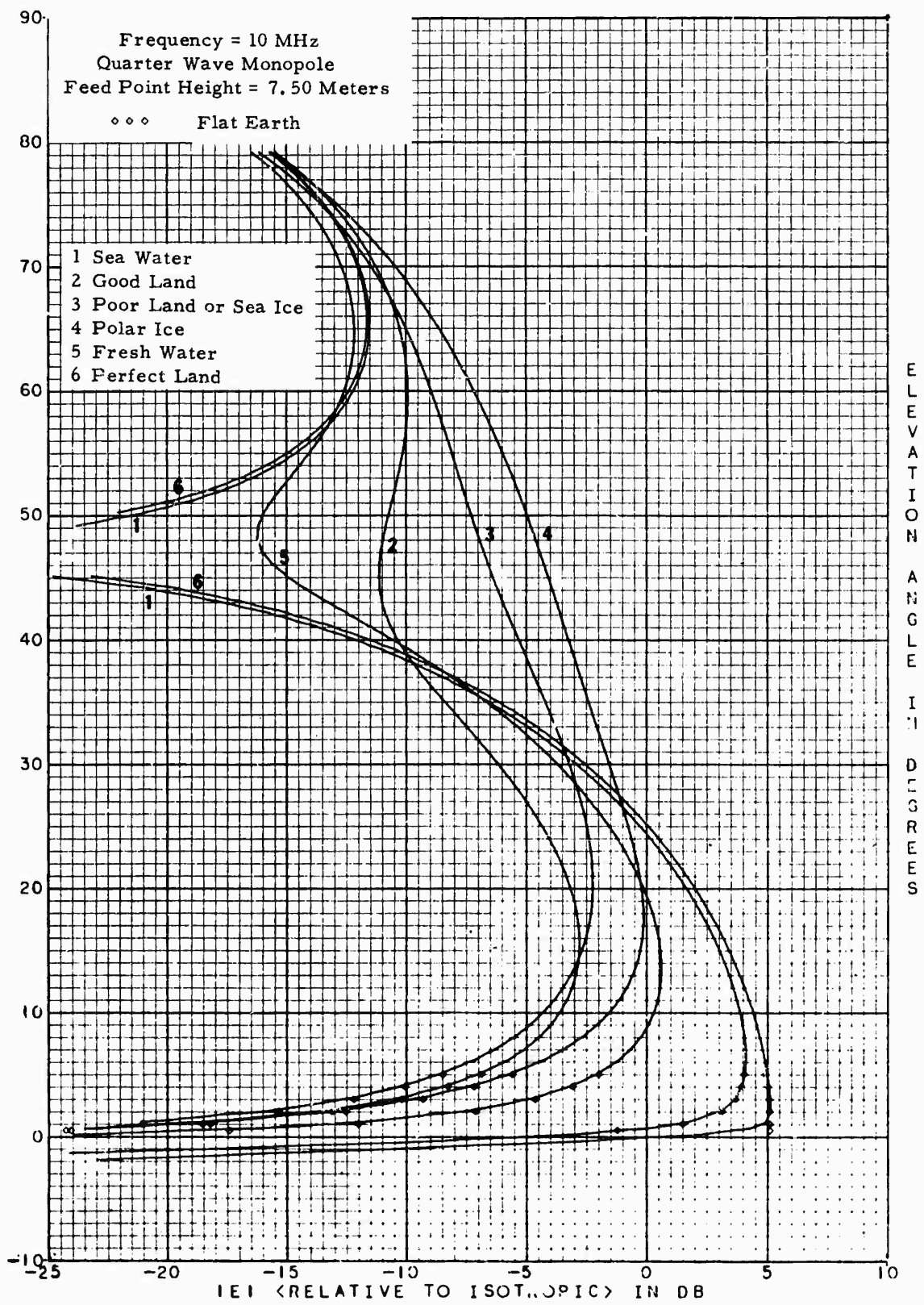
16. Vertical radiation pattern of a quarter-wave antenna with perfect counterpoise located \lambda/4 above various types of ground. The frequency is 10 MHz.
