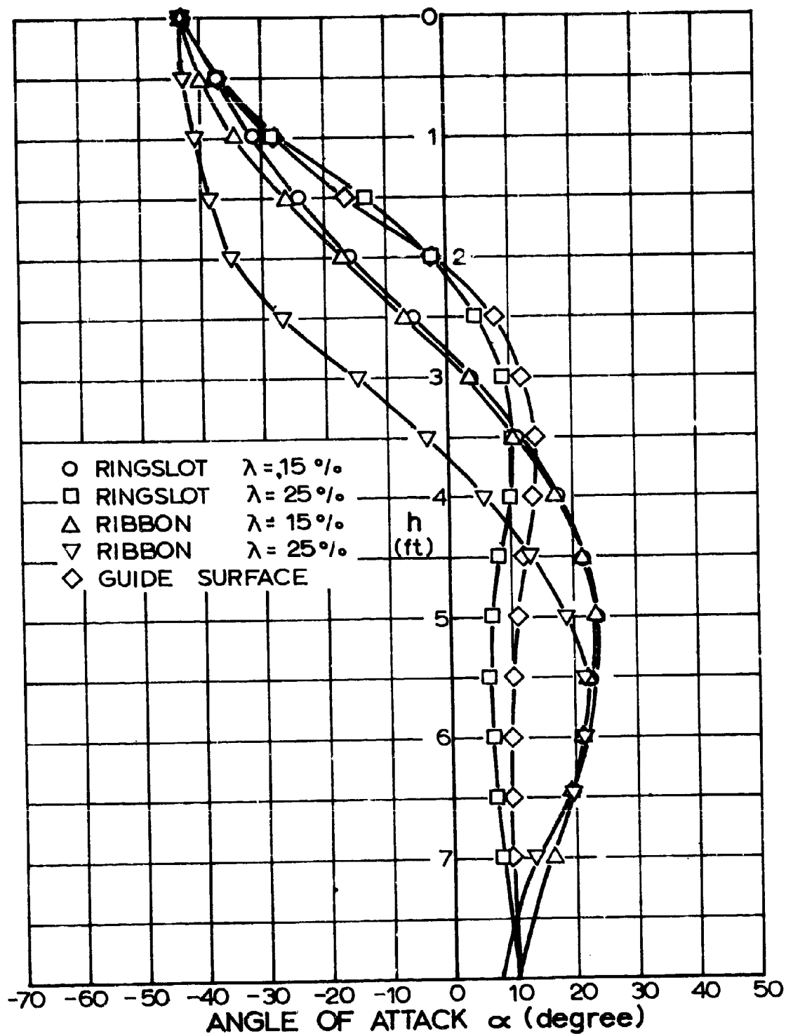
Fig 25. Angle of Attack as a Function of Altitude for Various Parachutes, Terminal Velocity ( V_{zp} ) = 40 ft/sec, Wind Velocity ( V_w ) = 37 ft/sec
