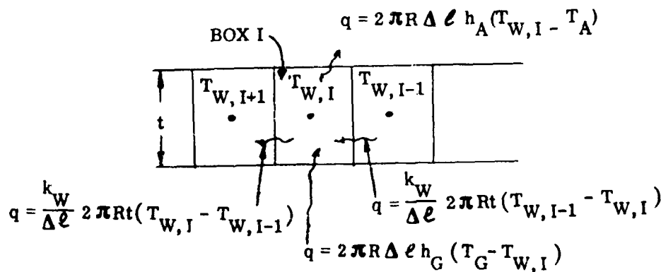
Figure 97. Tube Wall Section Showing Energy Flows.
