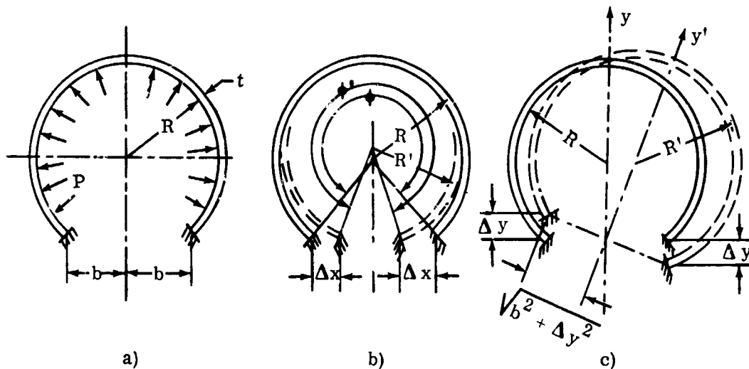
Figure 115. Suspension Stress Analysis Nomenclature Diagram.
