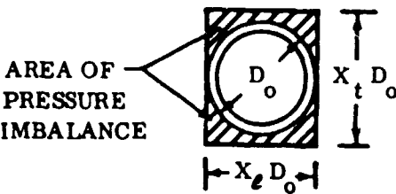
Figure 100. Sketch Showing Area of Differential Pressure.
