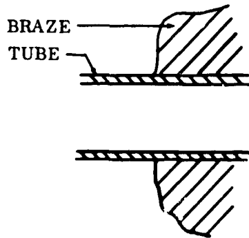
Figure 106. Brazing Alloy at Tube End.
