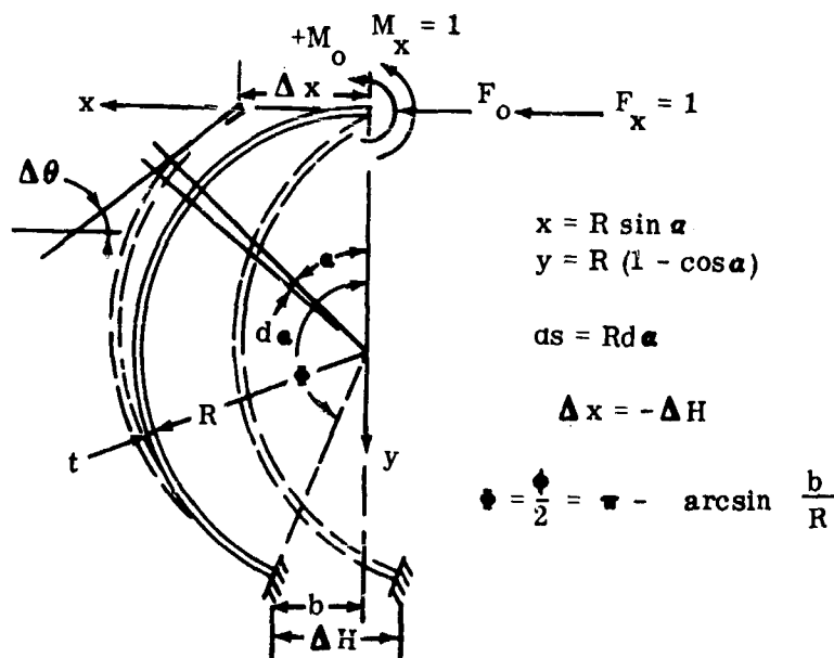
Figure 116. Suspension Stress Analysis Nomenclature Diagram.
