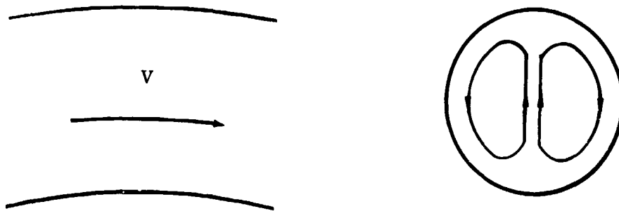
Figure 92. Secondary Flows in Curved Tube.
