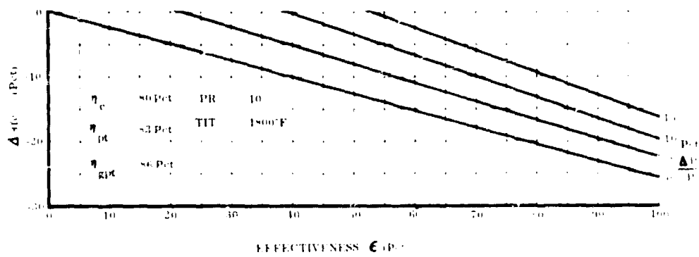
Figure 19. Fuel Flow Change by Adding Regenerator to Basic Gas Turbine Engine.
