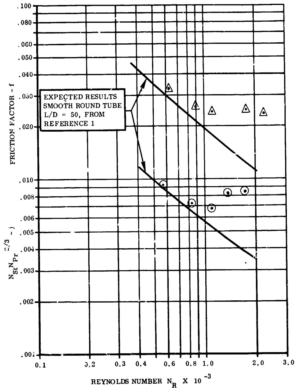
Figure 127. Heat Transfer and Pressure Drop Characteristics, Surface Roughened Tube, 0.042-Diameter Particles in 0.210 ID Tube.
