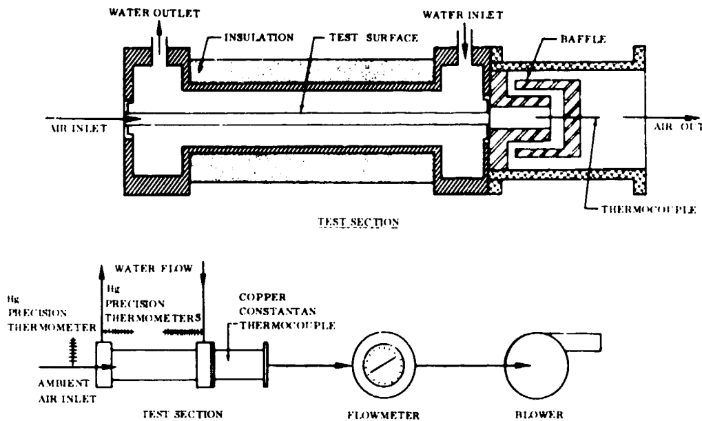
Figure 45. Steady-State Test Rig.
