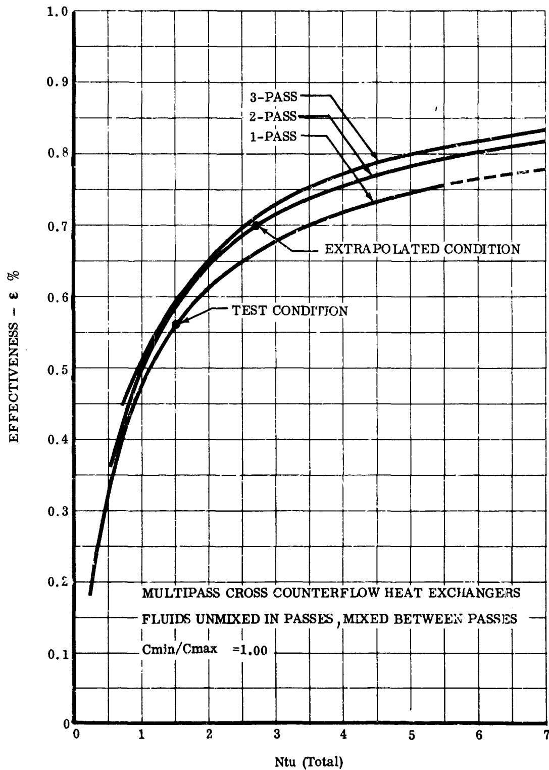
Figure 134. Effectiveness Versus Ntu.
