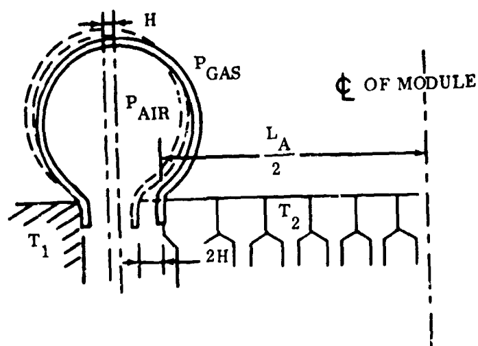
Figure 118. Displacement Due to Nonuniform Thermal Expansion.
