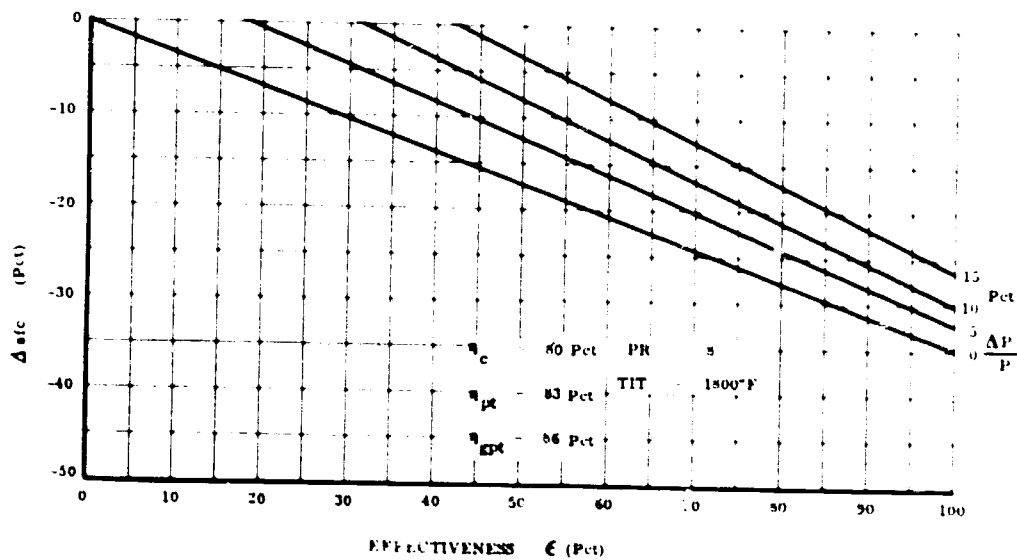
Figure 16. Fuel Flow Change by Adding Regenerator to Basic Gas Turbine Engine.
