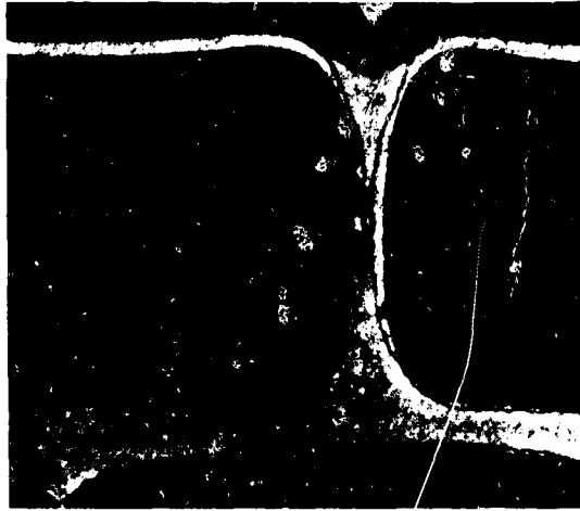
Figure 61b. Tube Wall Erosion by Palniro 1 (Similar for Palniro 7)
