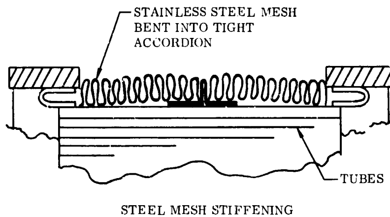
Figure 78. Other Suspension Stiffening Modifications.
