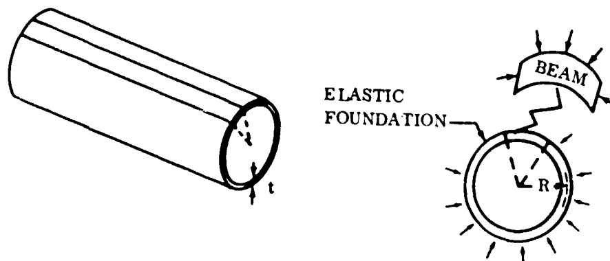
Figure 108. "Elastic Foundation" Method of Analysis.
