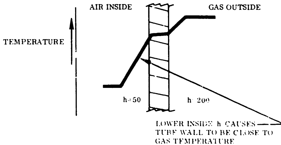
Figure 56. Effect of Gas Flowing Inside Tubes.
