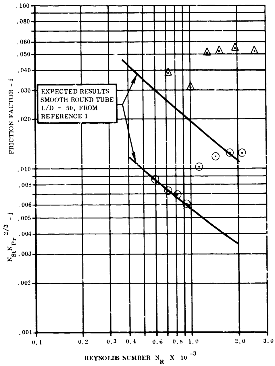
Figure 121. Heat Transfer and Pressure Drop Characteristics, Ring-Dimpled Tube.
