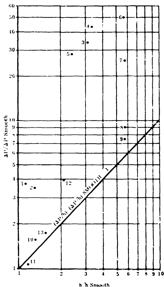
Figure 35. Summary Of The Effects Of Turbulence-Promoting Devices Inside Tubes.
