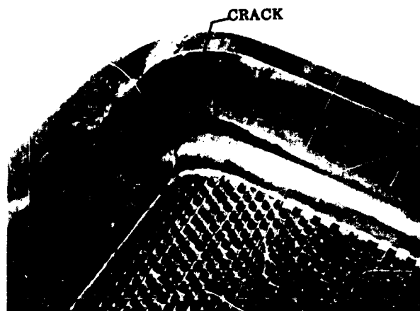
Figure 80. Crack in Modified Suspension.
