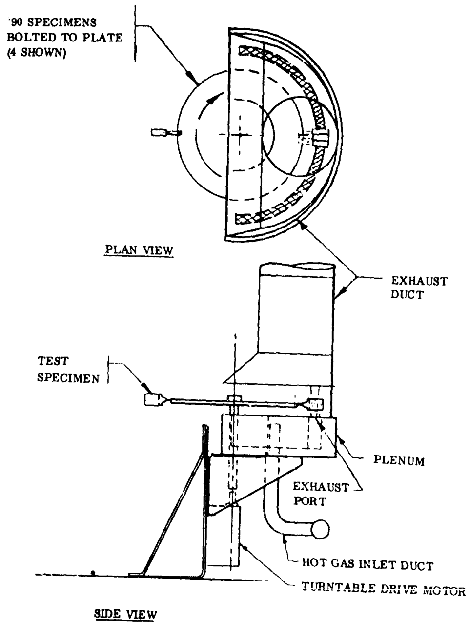
Figure 91. Oxidation and Corrosion Test Rig.
