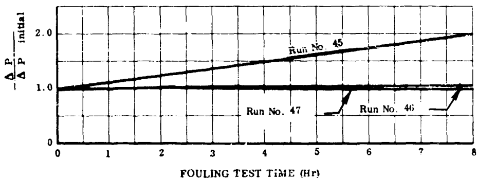
Figure 86. Gas in Tube Fouling Characteristics, Wavy-Tube Module.
