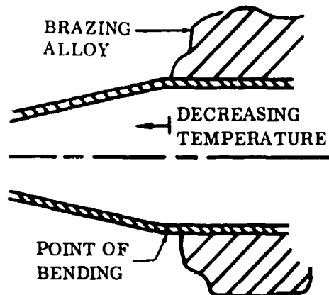
Figure 107. Bending of Wall at Tube End.
