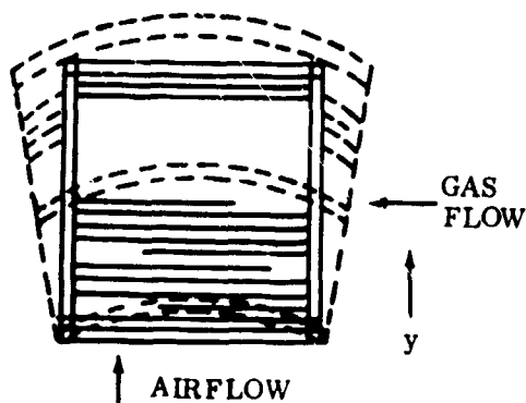
Figure 101. Exaggerated Bowing of Tubes due to Thermal Gradient. (Exaggerated for illustration)
