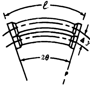
Figure 102. Bowing of Tubes.
