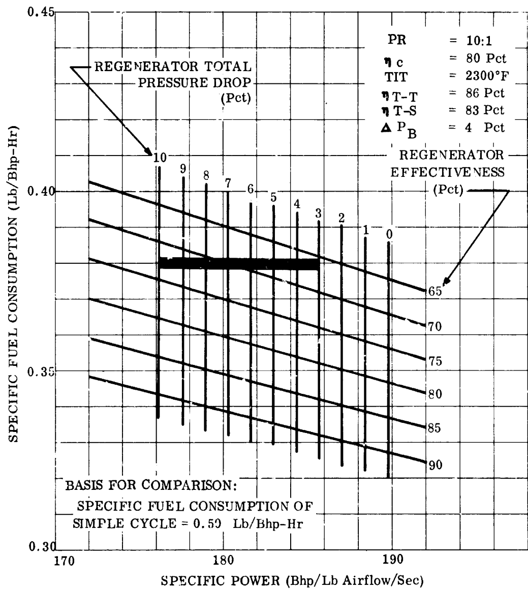
Figure 8. Specific Fuel Consumption and Specific Power as Function of Regenerator Performance.
