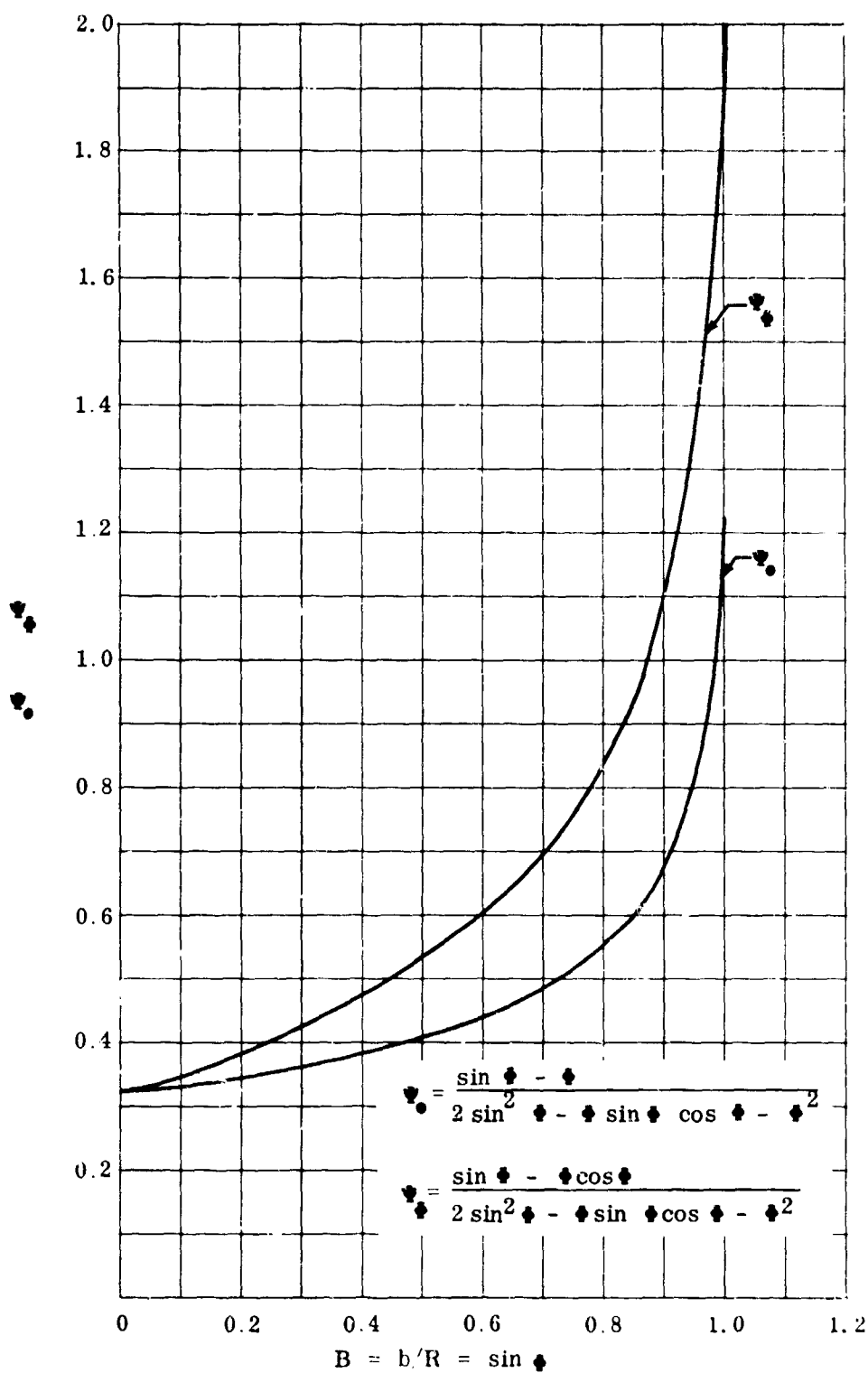
Figure 117. Suspension Stress Analysis Functions.
