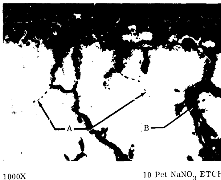
Figure 90. Sulfidation Attack.
