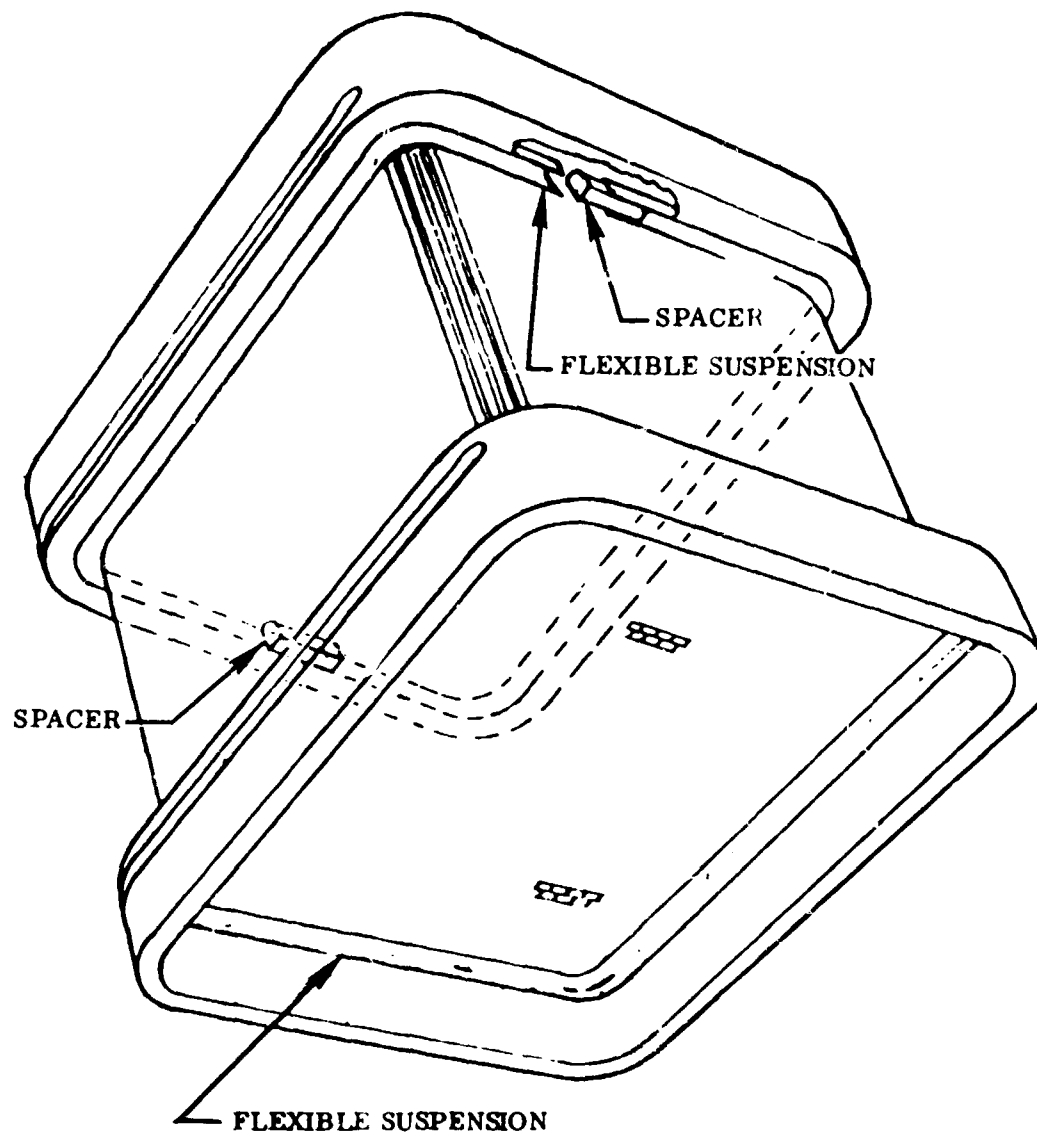
Figure 76. Suspension With Steel Spacers.
