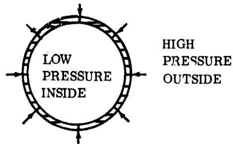
Figure 98. Sketch Showing Loading Creating Hoop Stress.
