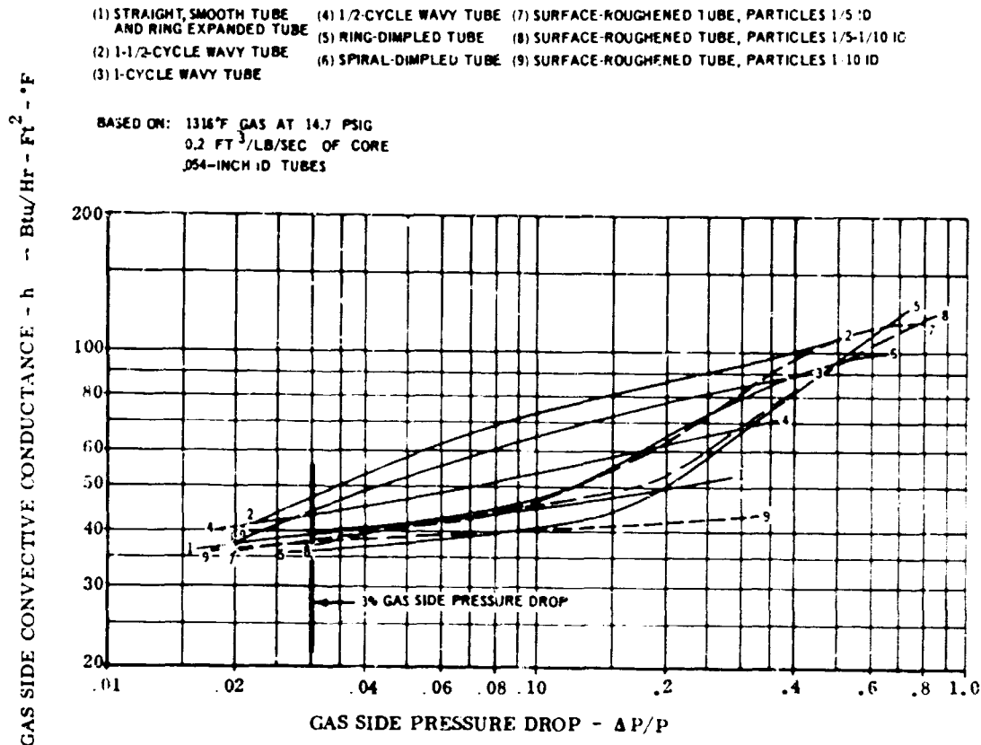
Figure 49. Characteristics of Modified Tubular Surfaces.
