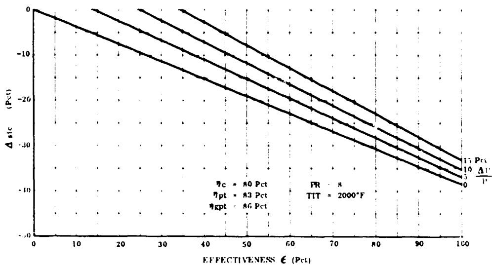
Figure 17. Fuel Flow Change by Adding Regenerator to Basic Gas Turbine Engine.
