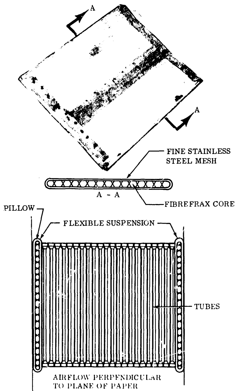
Figure 59. Sealing Pillow Showing Installation.
