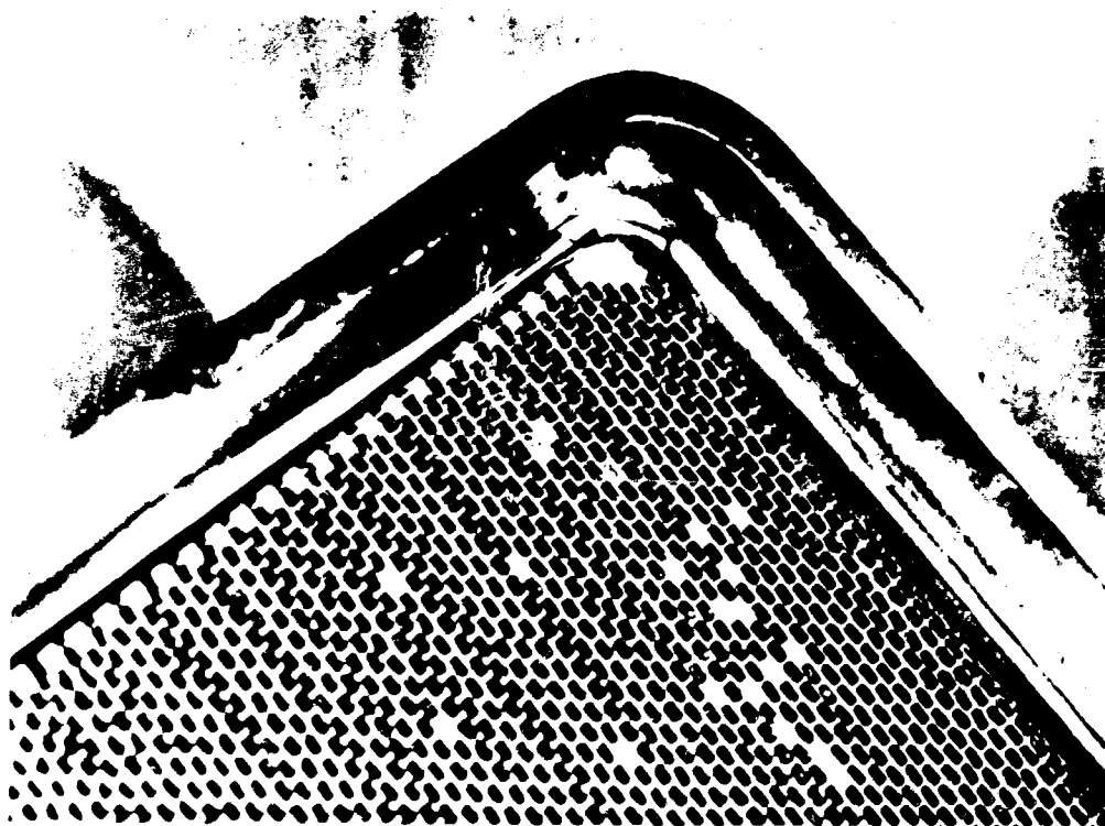
Figure 75. Damage to Corner of Suspension After First Vibration Test.
