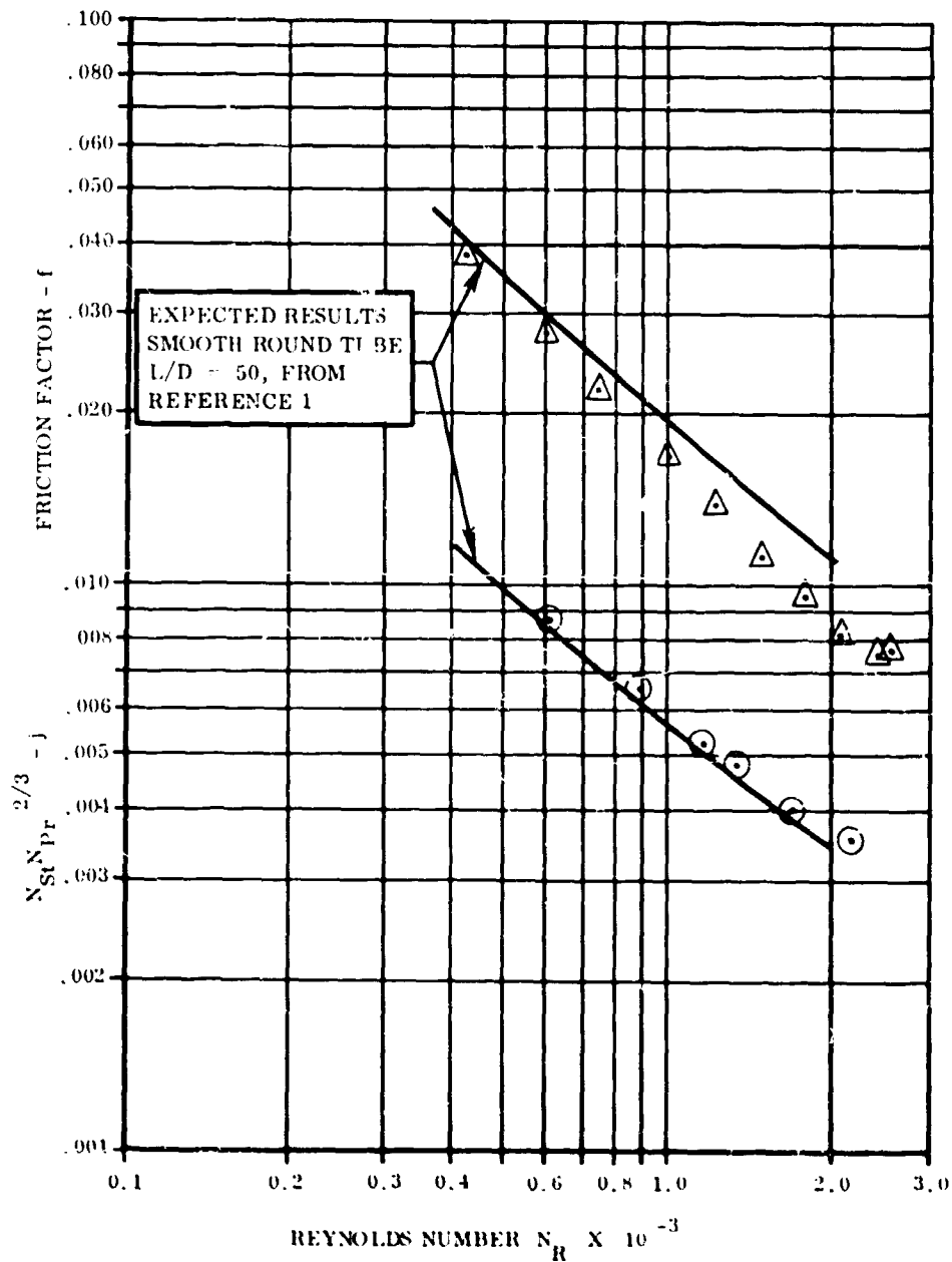
Figure 120. Heat Transfer and Pressure Drop Characteristics, Smooth Tube, Flared Ends.
