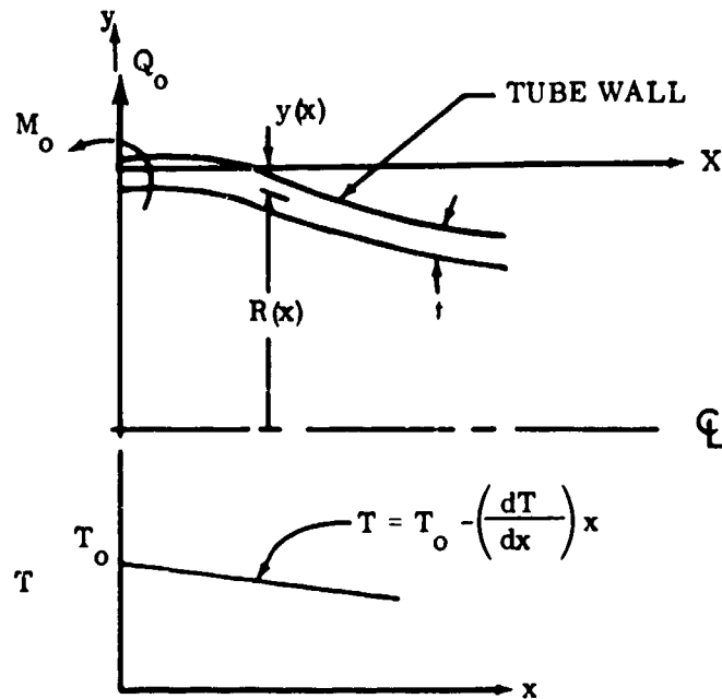
Figure 109. Loading of "Beam" (Tube Wall).
