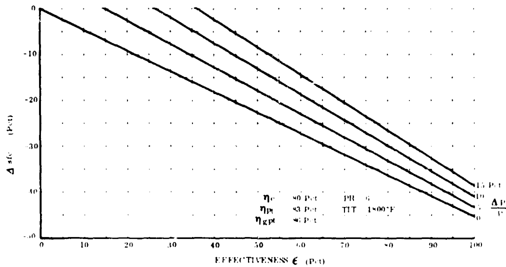
Figure 13. Fuel Flow Change by Adding Regenerator to Basic Gas Turbine Engine.
