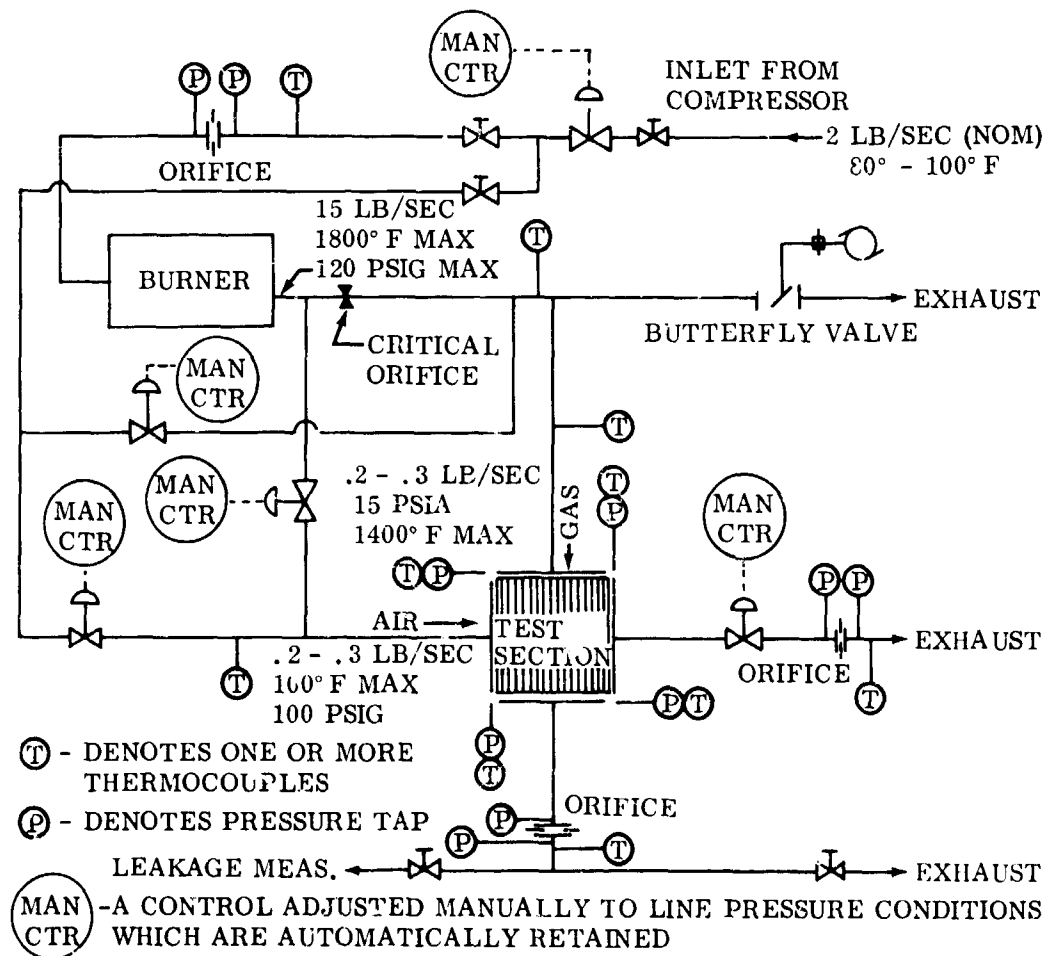
Figure 81. Thermal Shock and Fouling Rig.
