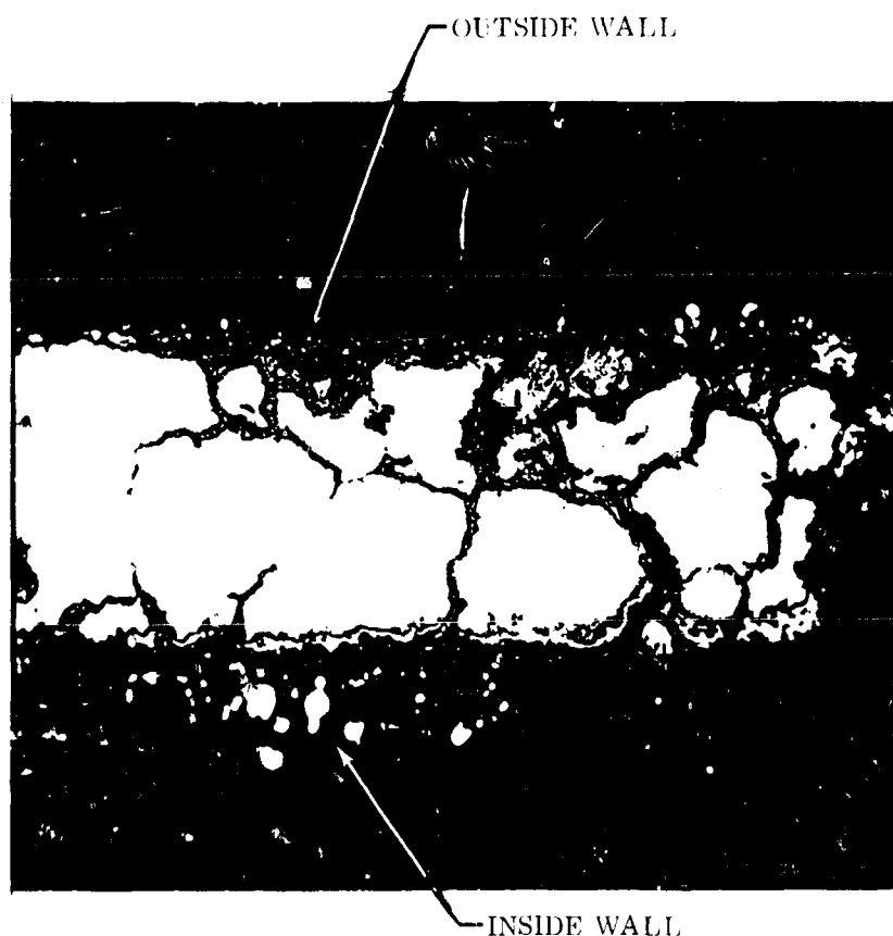
Figure 89. Intergranular Oxidation Near Tube Fracture Point.
