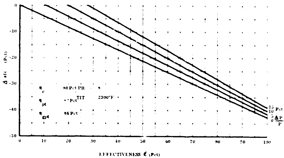
Figure 18. Fuel Flow Change by Adding Regenerator to Basic Gas Turbine Engine.
