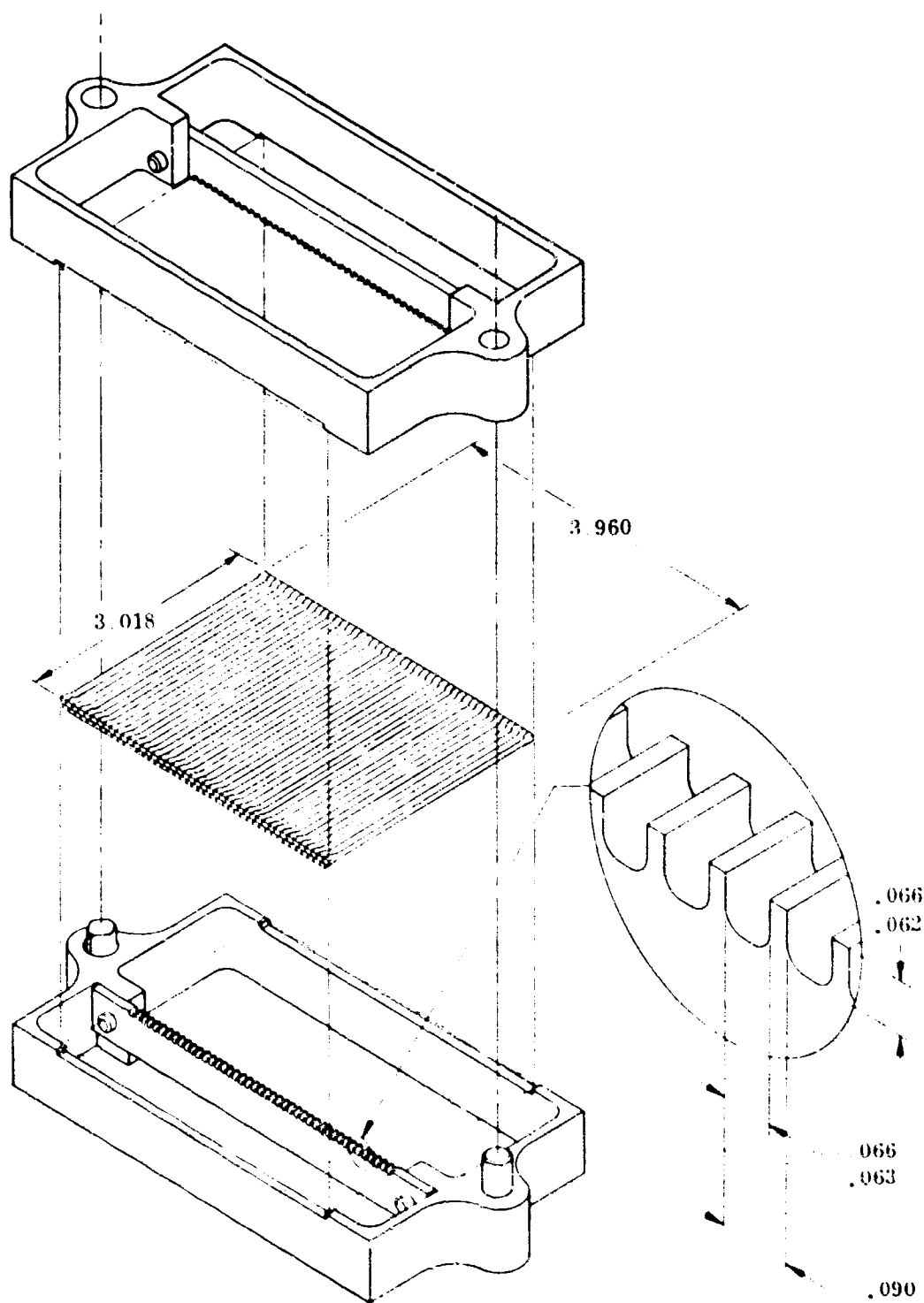
Figure 66. Double-Layer Brazing Fixture.
