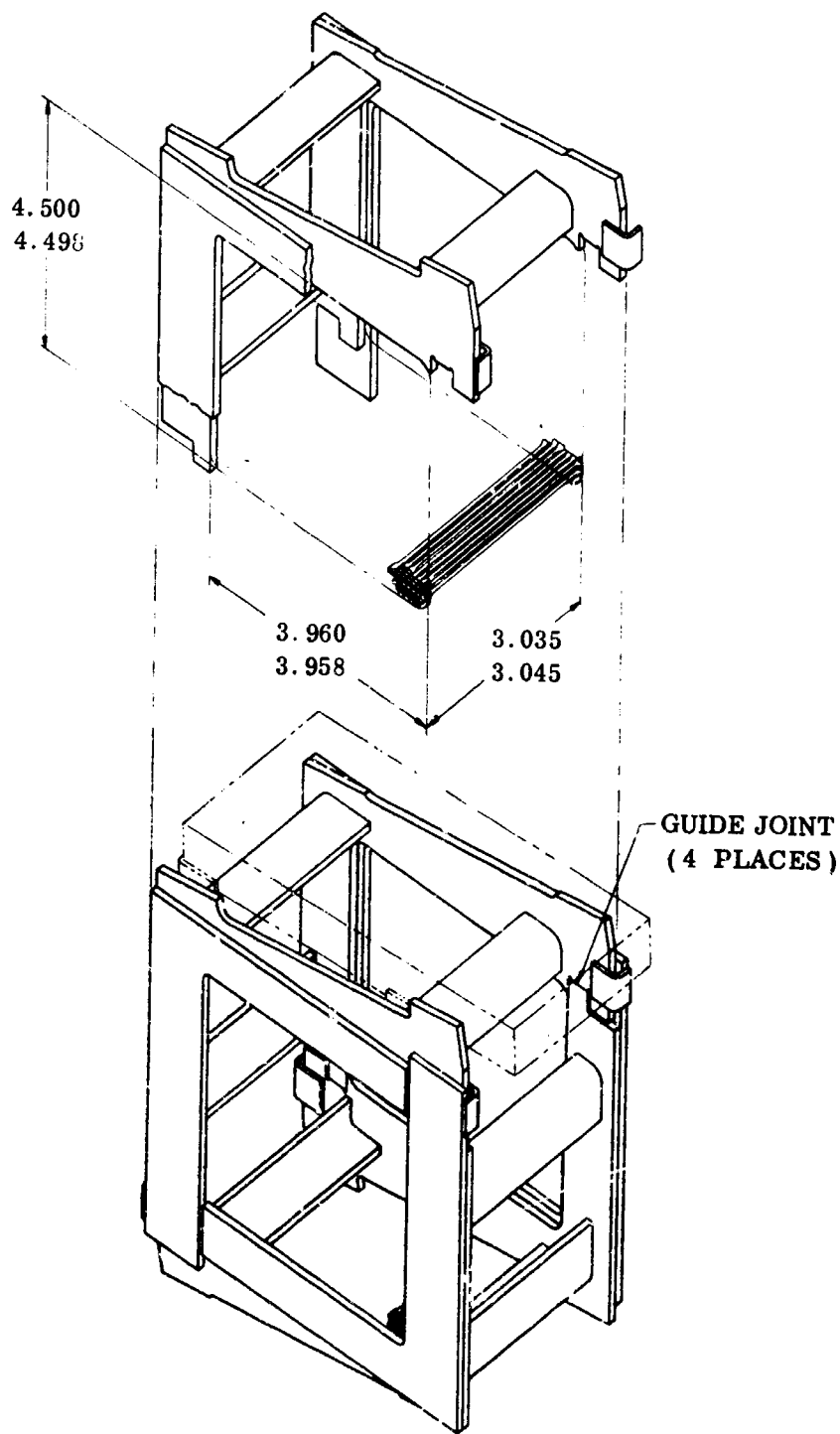
Figure 68. Complete Module Brazing Fixture.
