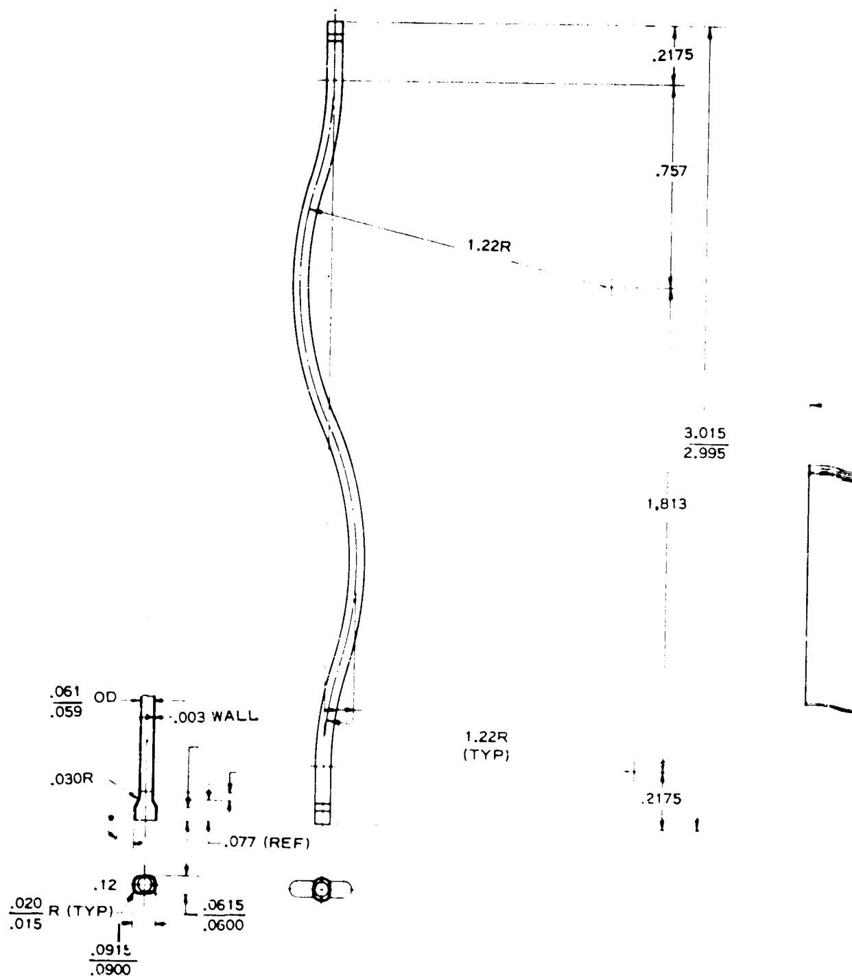
Figure 55. Wavy-Tube Module Design.
