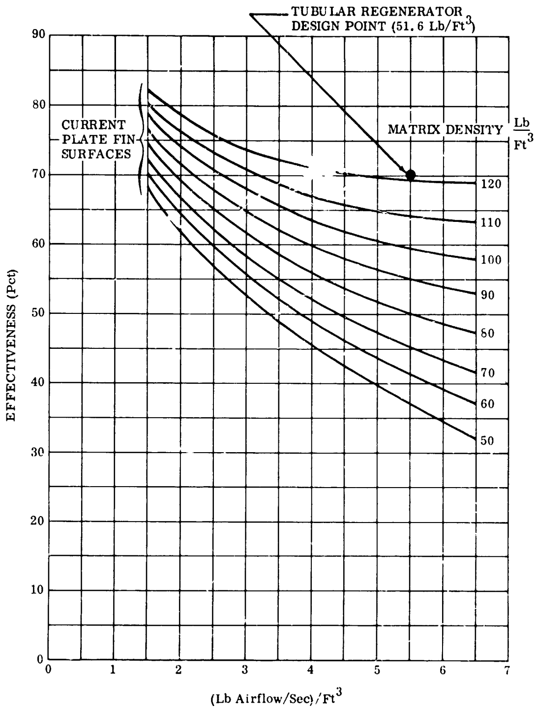
Figure 9. Regenerator Comparison.
