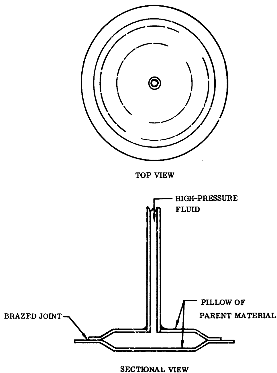
Figure 60. Brazed Pillow Test Specimen.
