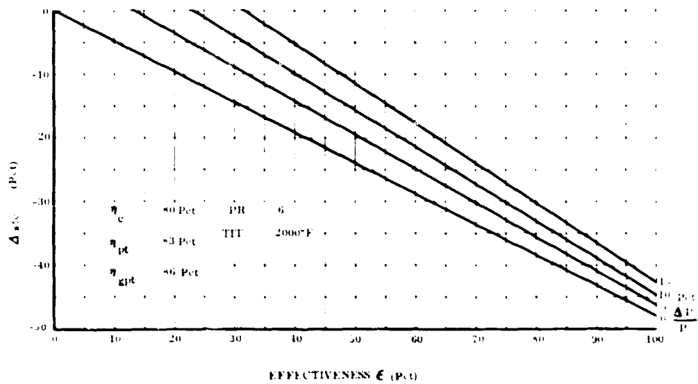
Figure 14. Fuel Flow Change by Adding Regenerator to Basic Gas Turbine Engine.
