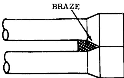
Figure 42a. Excessive Braze Causing High Stress Level
