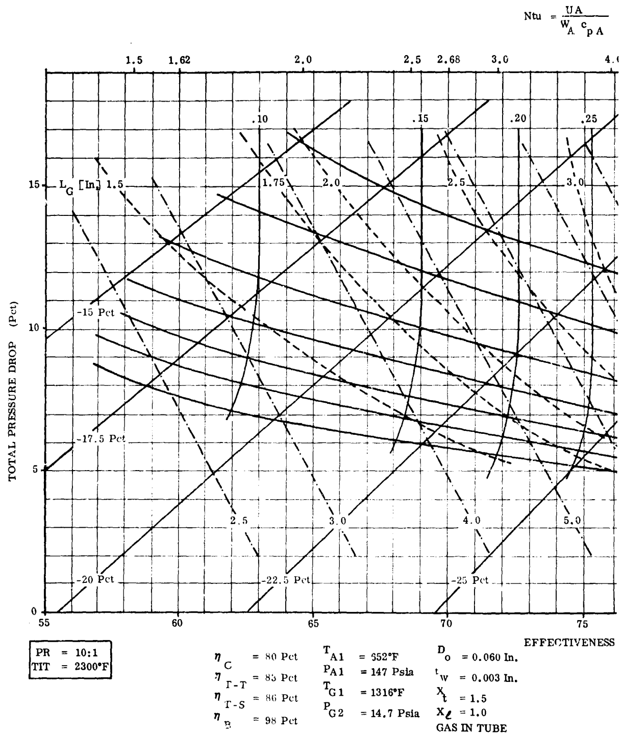
Figure 23. Regenerator Performance Map.
