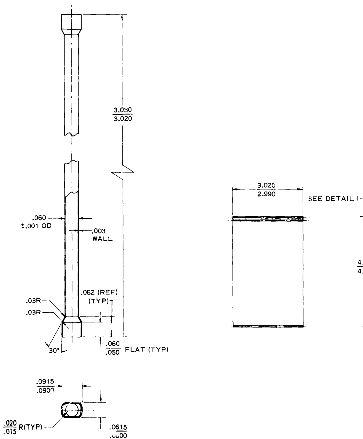
Figure 54. Straight-Tube Module Design.
