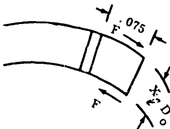
Figure 103. Region of Shear Forces at Tube End.
