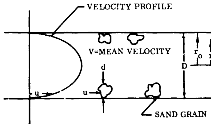
Figure 93. Surface Roughness in Tube.
