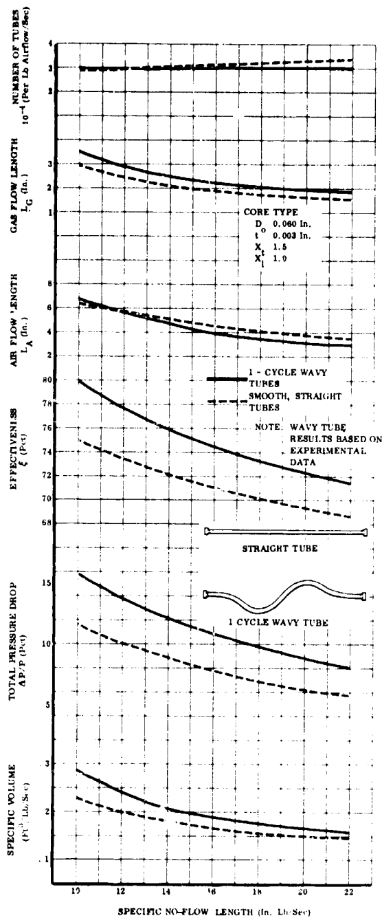
Figure 25. Optimum Regenerator Designs For Model Engine With 22.5 Percent Reduction of Specific Fuel Consumption.
