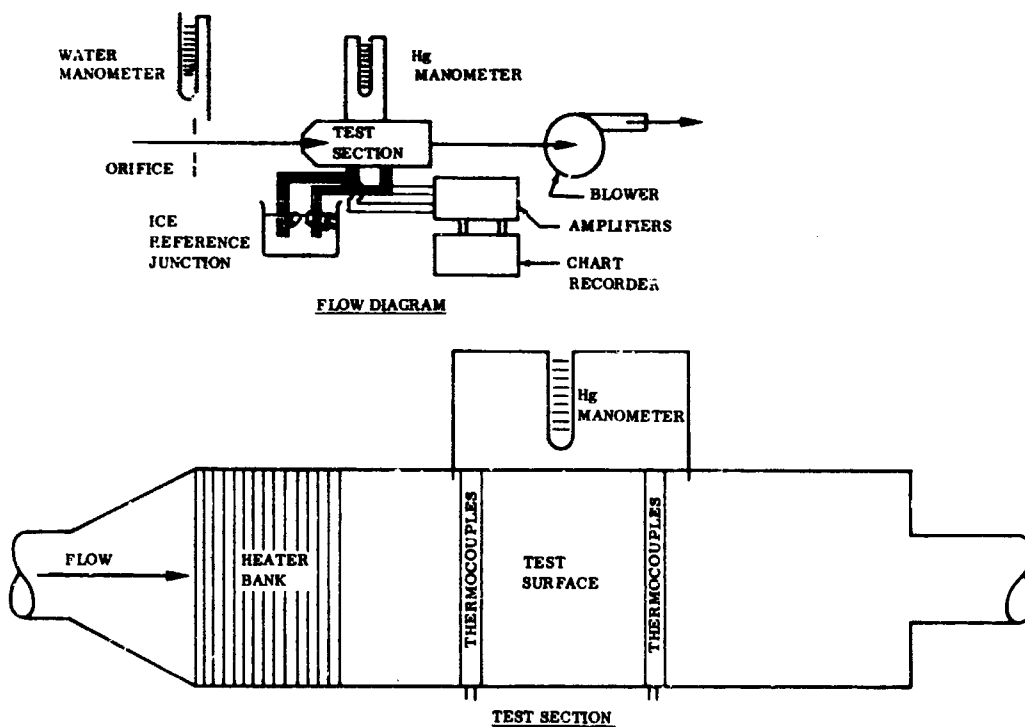
Figure 50. Transient Test Rig.
