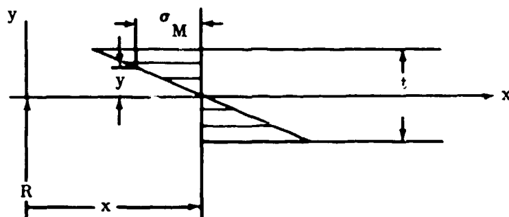
Figure 110. Meridional Normal Stress Diagram.
