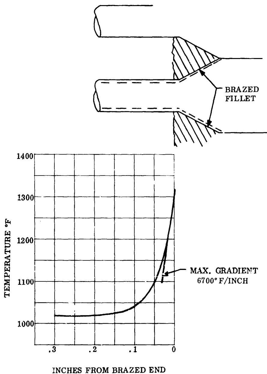
Figure 38. Temperature Gradient At Tube End.
