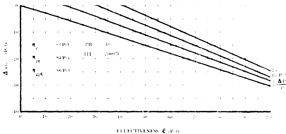
Figure 20. Fuel Flow Change by Adding Regenerator to Basic Gas Turbine Engine.
