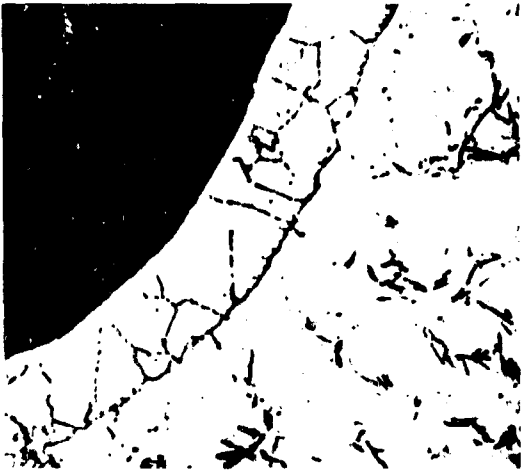
Figure 61a. Grain Boundary Penetration by Coating Metals 62
