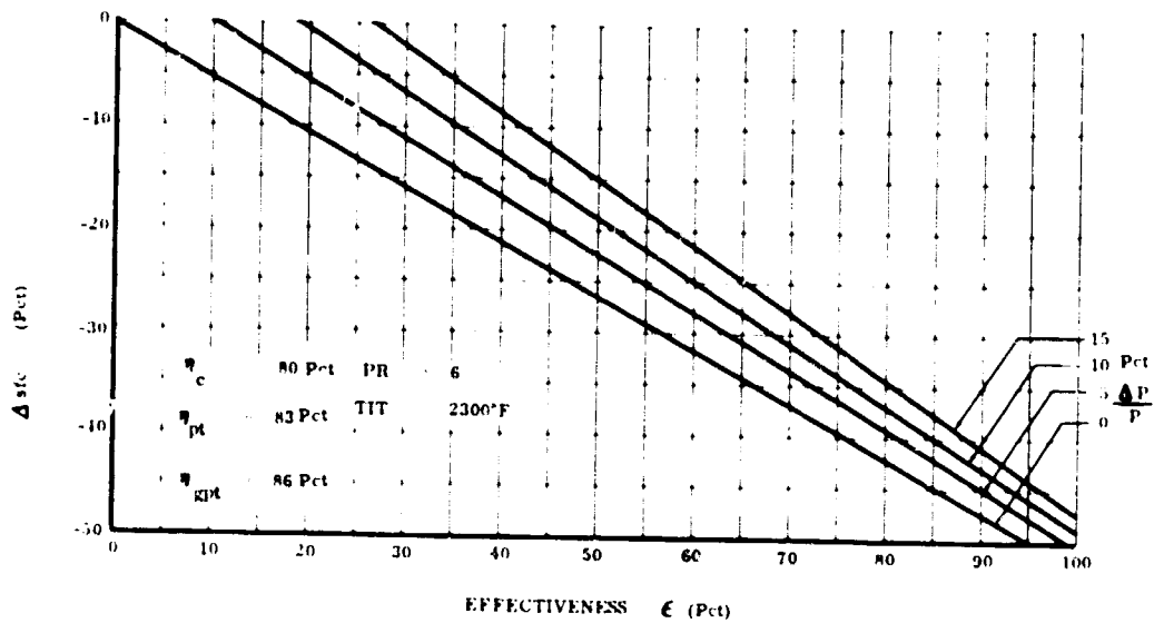
Figure 15. Fuel Flow Change by Adding Regenerator to Basic Gas Turbine Engine.
