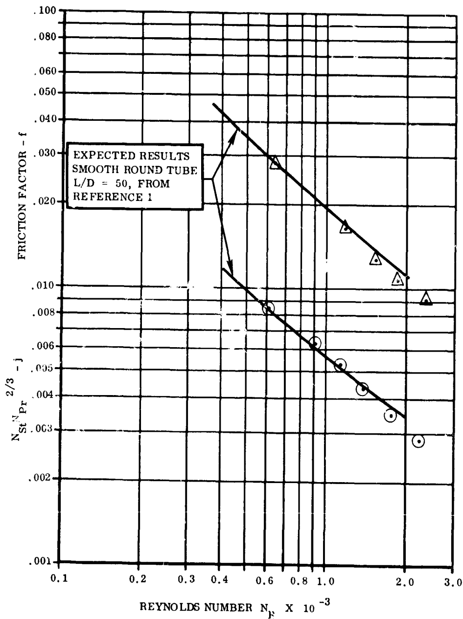
Figure 128. Heat Transfer and Pressure Drop Characteristics, Surface Roughened Tube, 0.021-Diameter Particles in 0.210 ID Tube.
