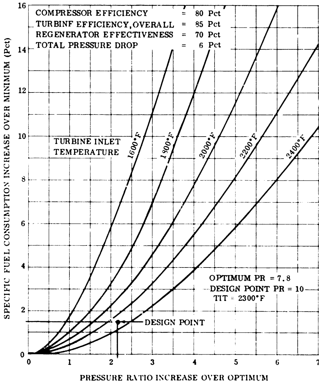
Figure 7. Specific Fuel Consumption Increase for Off-Optimum Compression Ratio.
