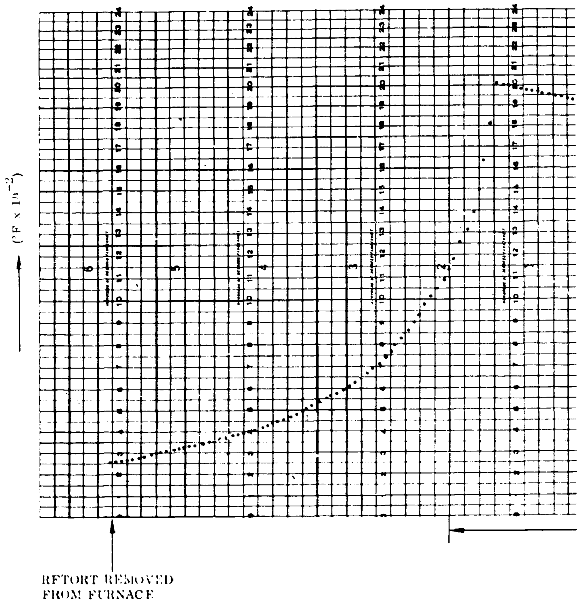
Figure 70. Pyromet Braze Cycle Temperature versus Time.
