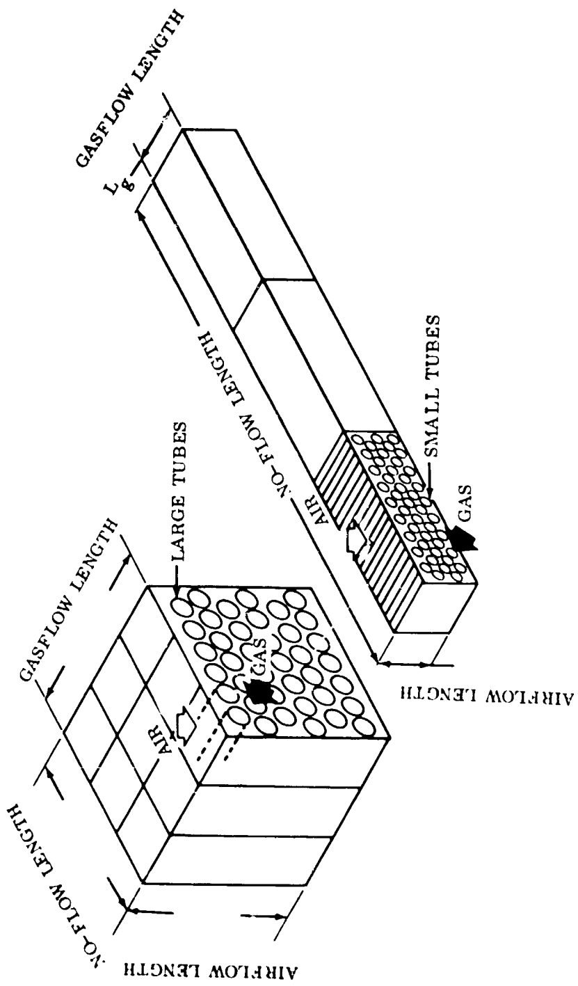
Figure 11. Effect of Tube Diameter on No-Flow Length.
