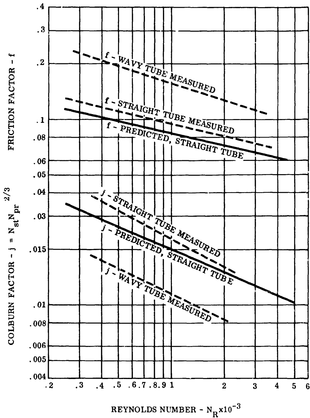
Figure 53. Heat Transfer and Pressure Drop Characteristics for Flow Across Banks of Straight and 1-Cycle Wavy Tubes.
