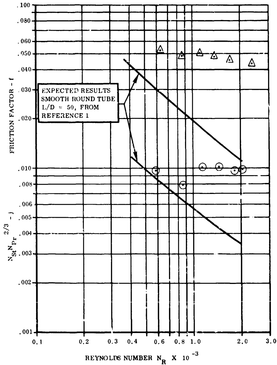
Figure 129. Heat Transfer and Pressure Drop Characteristics, Surface Roughened Tube. Mixed Sand Grains From 0.016 to 0.046 Diameter in 0.210 ID Tube.
