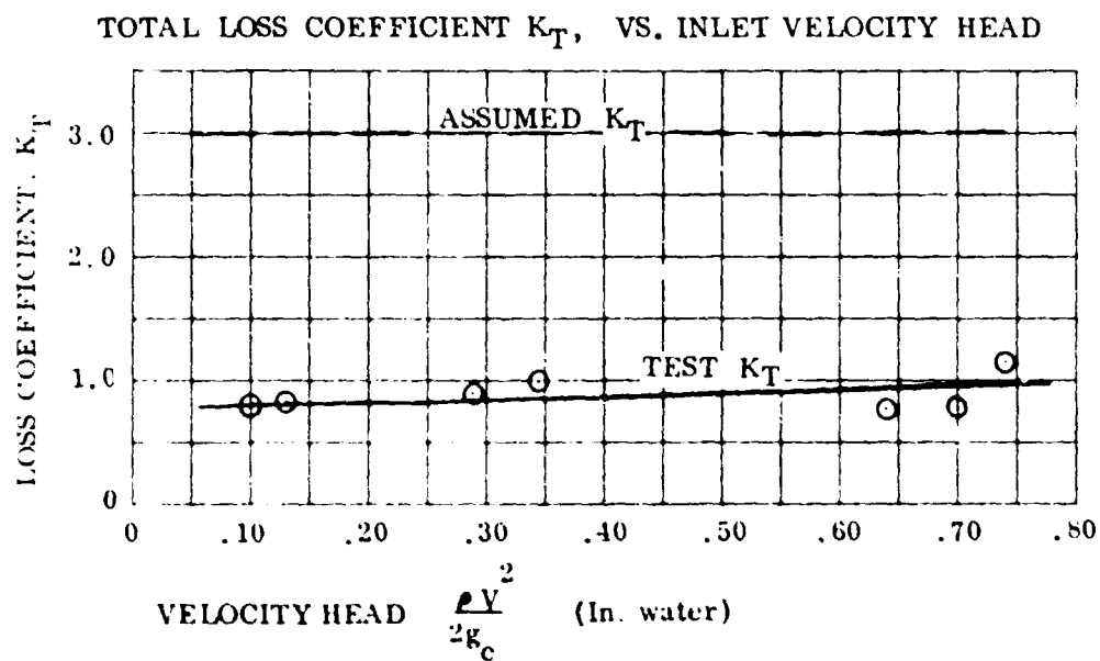
Figure 34. Duct Turning Losses.
