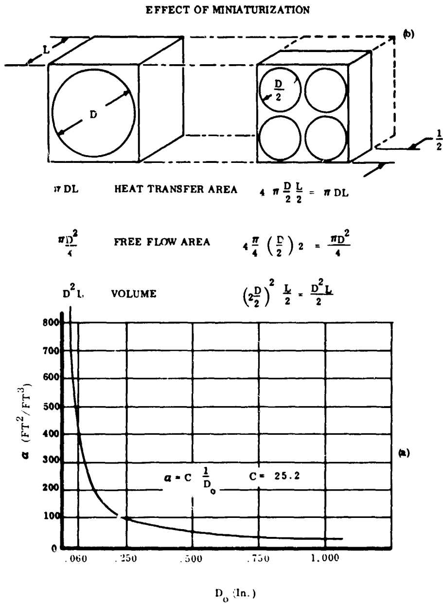
Figure 10. Core Compactness Versus Tube Diameter.
