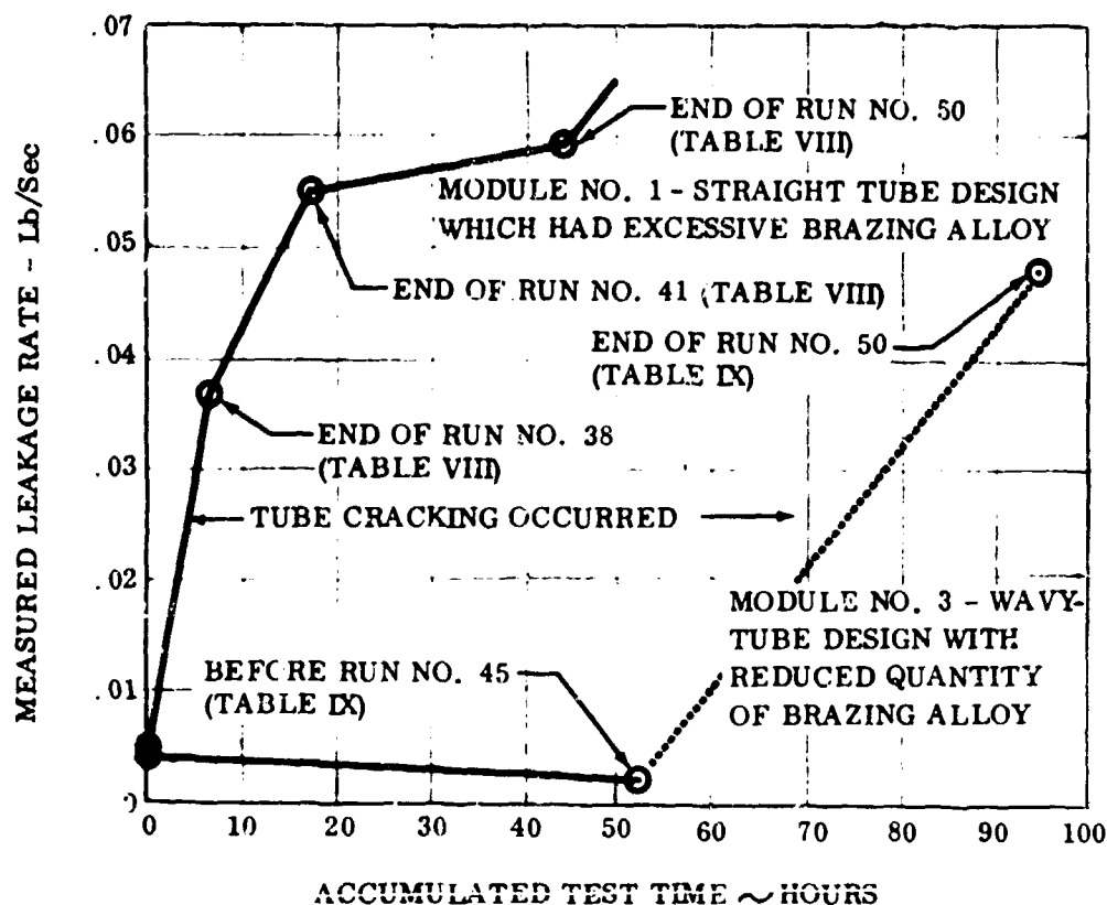
Figure 87. Module Leakage Rate With Test Time.
