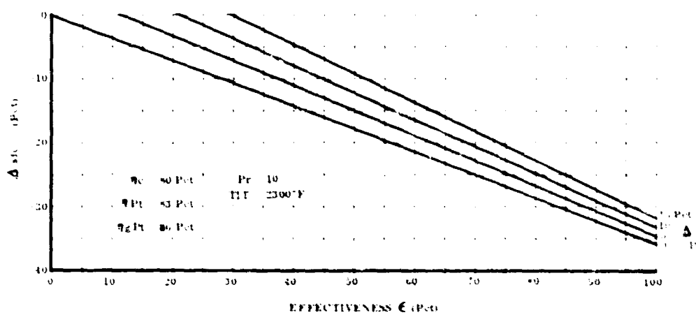
Figure 21. Fuel Flow Change by Adding Regenerator to Basic Gas Turbine Engine.
