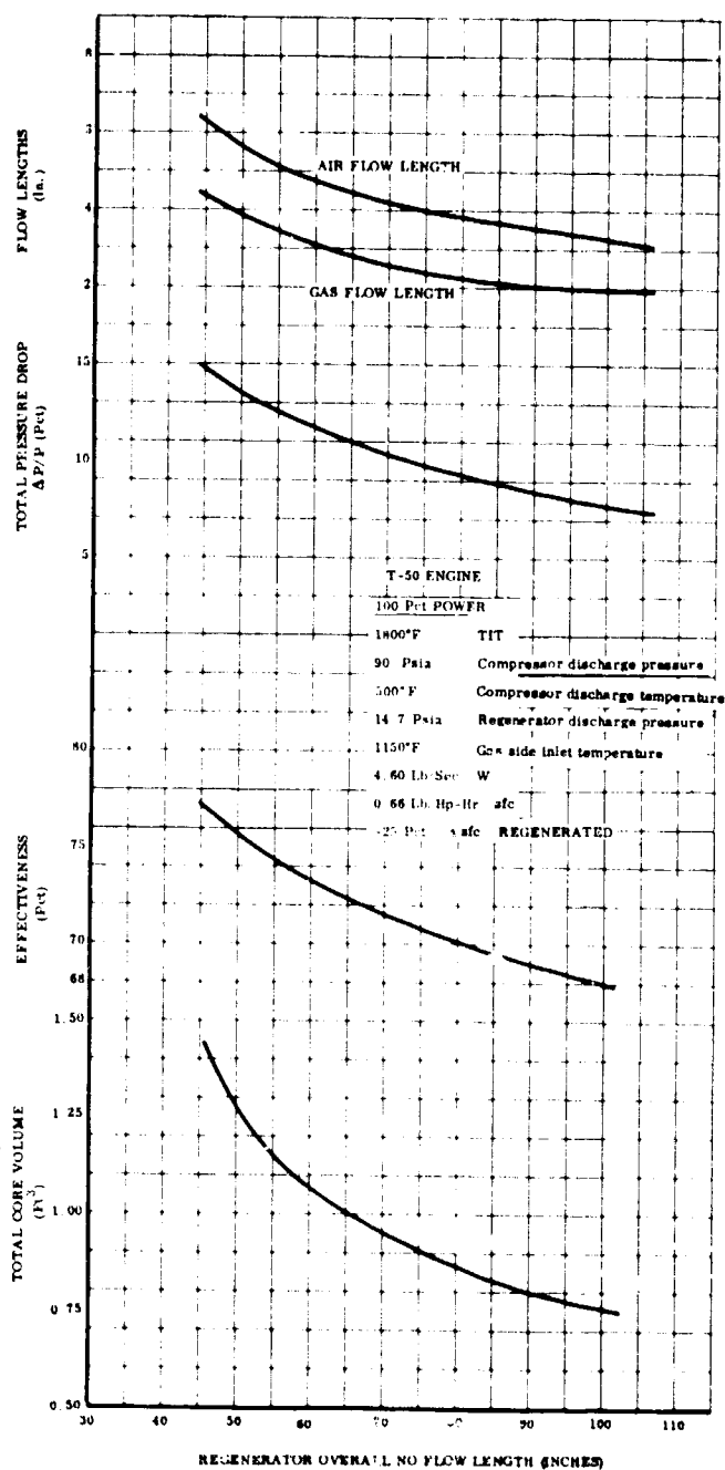
Figure 27. Optimum Regenerator Designs For T50 Engine With 25 Percent Reduction of Specific Fuel Consumption.
