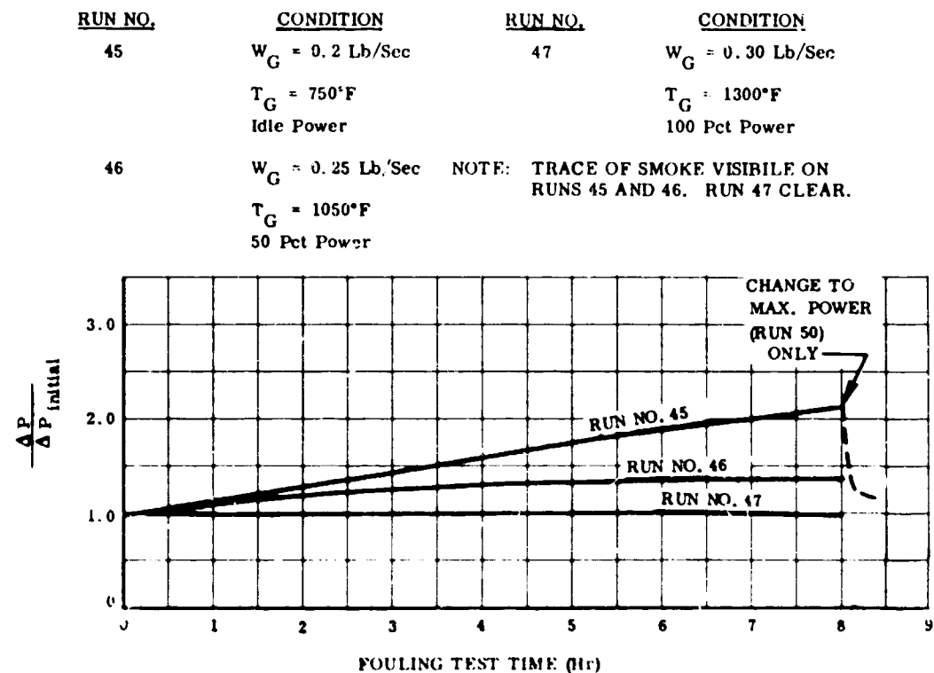
Figure 85. Gas in Tube Fouling Characteristics, Straight-Tube Module.
