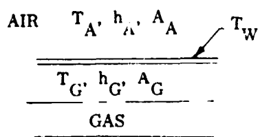
Figure 94. Tube Section Showing Heat Transfer Nomenclature.
