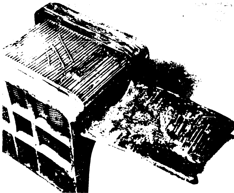
Figure 84. Damage to First Straight-Tube Module Due to Combustion of Carbon Outside Tubes.
