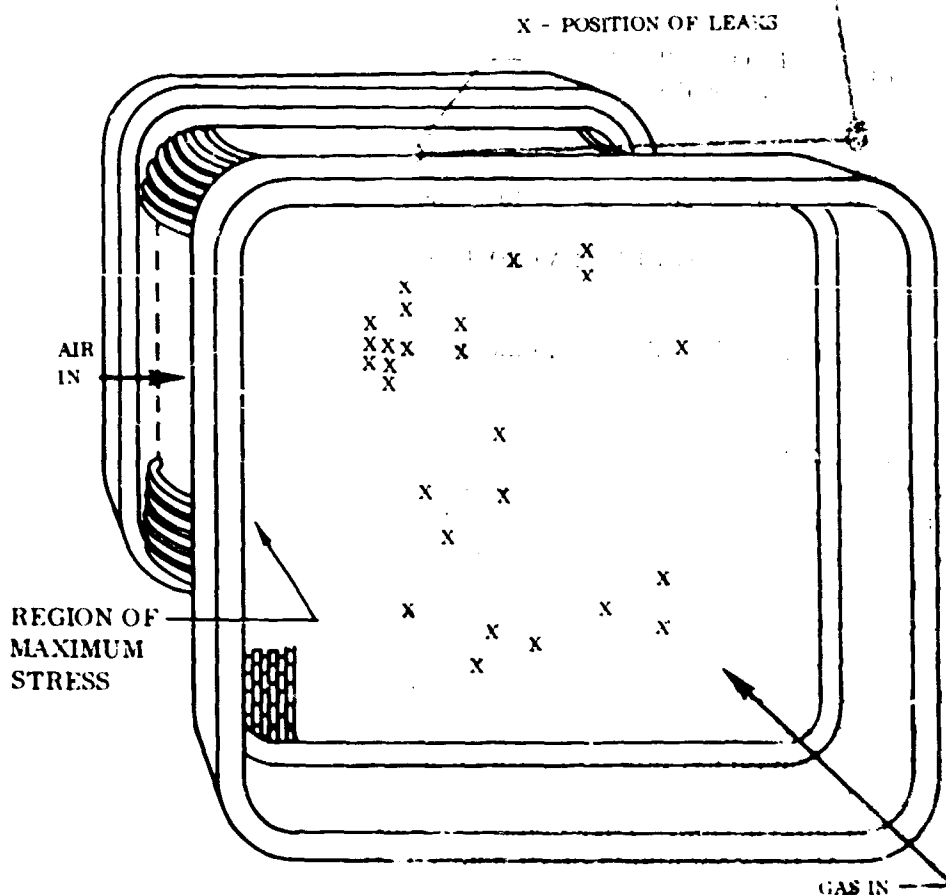
Figure 88. Wavy-Tube Module Leak Positions. (After 95 Hours)
