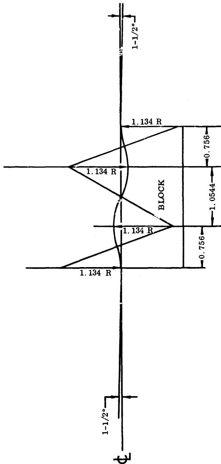
Figure 132. Wavy-Tube Die Block.
