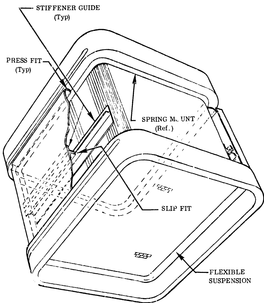
Figure 77. Module With Stiffener Guide.
