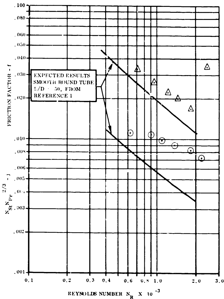
Figure 125. Heat Transfer and Pressure Drop Characteristics, 1-1/2-Cycle Wavy Tube.
