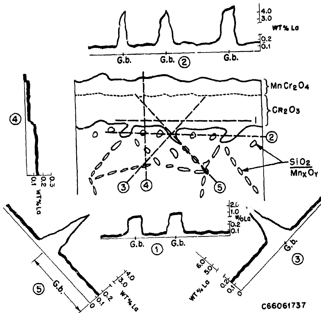
FIGURE 66 Microprobe Analysis of René Y for La Detection
