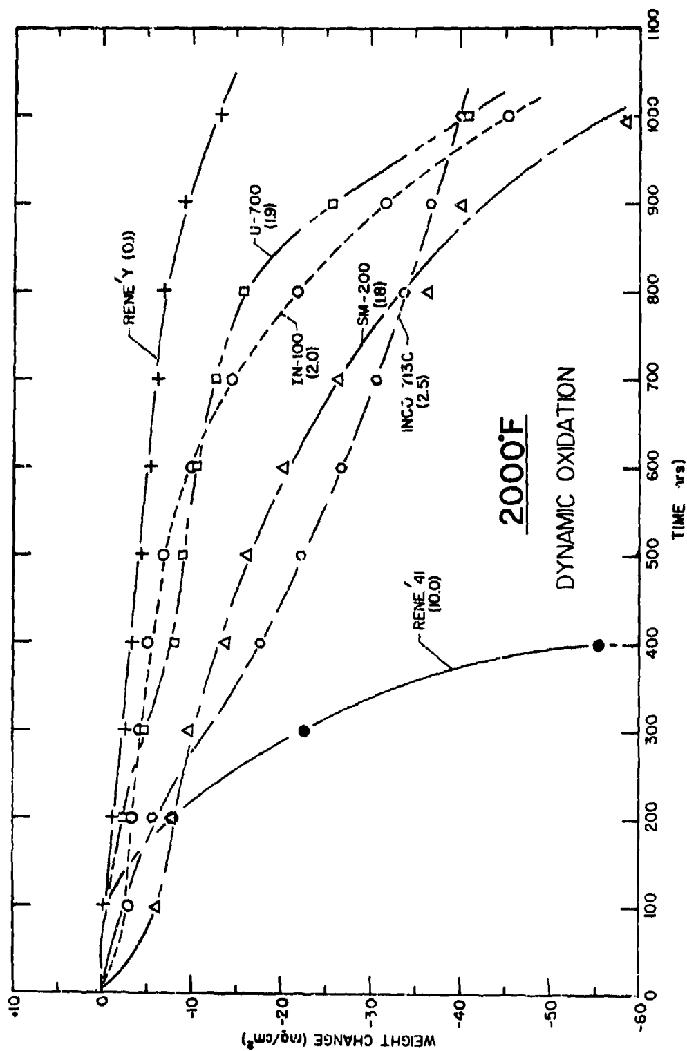
FIGURE 60 Weight Change During Oxidation in High Velocity Natural Gas Combustion Products at 2000°F
