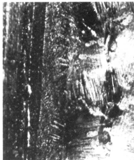
Figure A17. Tungsten-Arc Weld, dc, on E-130R2 Bomblet Without Filler-Metal Addition
