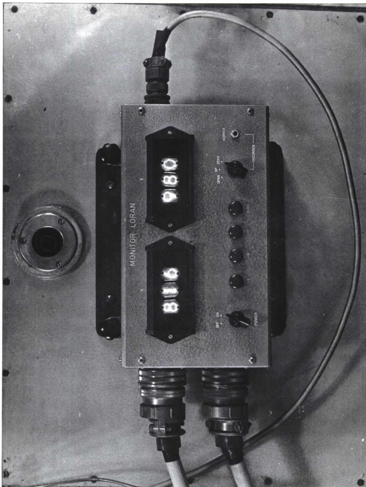
FIG. 7 BRIDGE REPEATER
