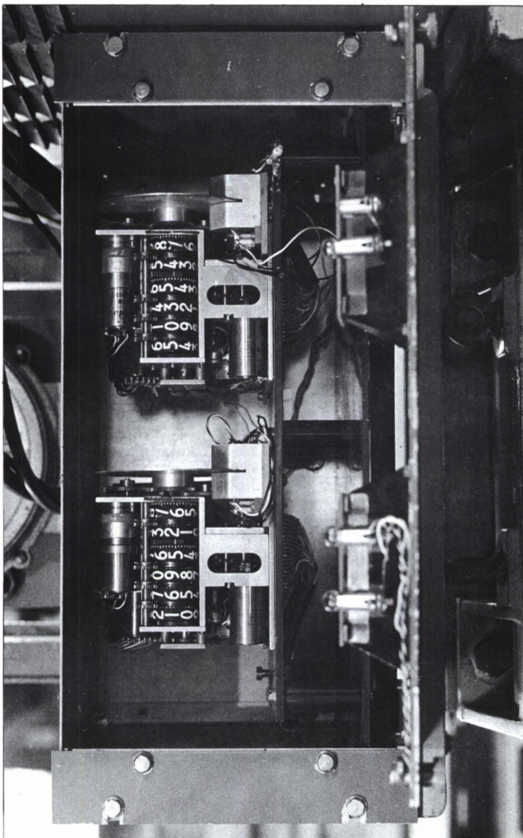
FIG. 5 PHOTODIODE SYSTEM FITTED TO THE SLAVE DELAY MODULES
