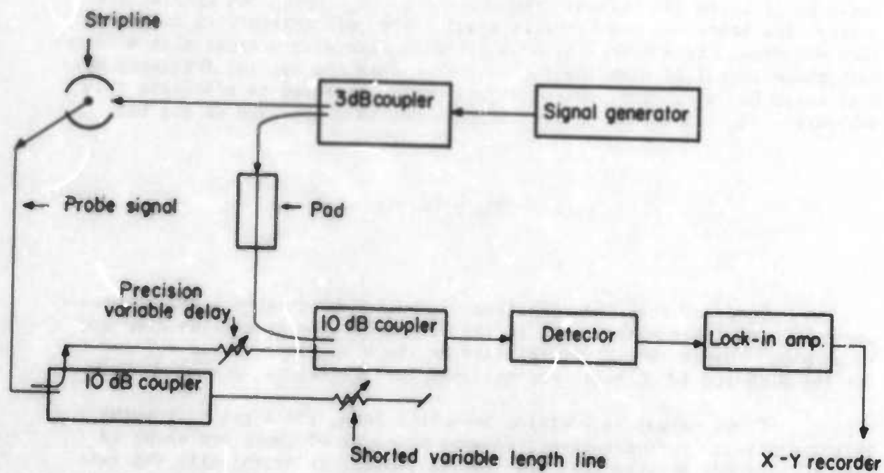
FIG. 9 Experimental set up for the detection of the phase velocity of the electrostatic waves propagating across the plasma column.
