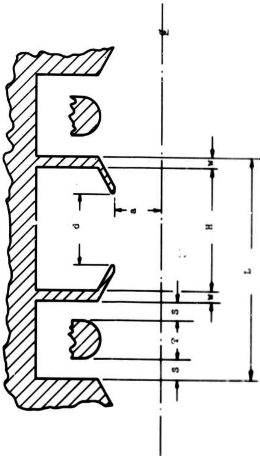
CAVITY-LENS CONFIGURATION
