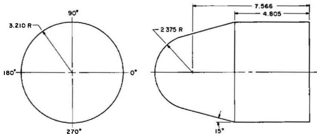
MODIFIED GEMINI DETAILS
