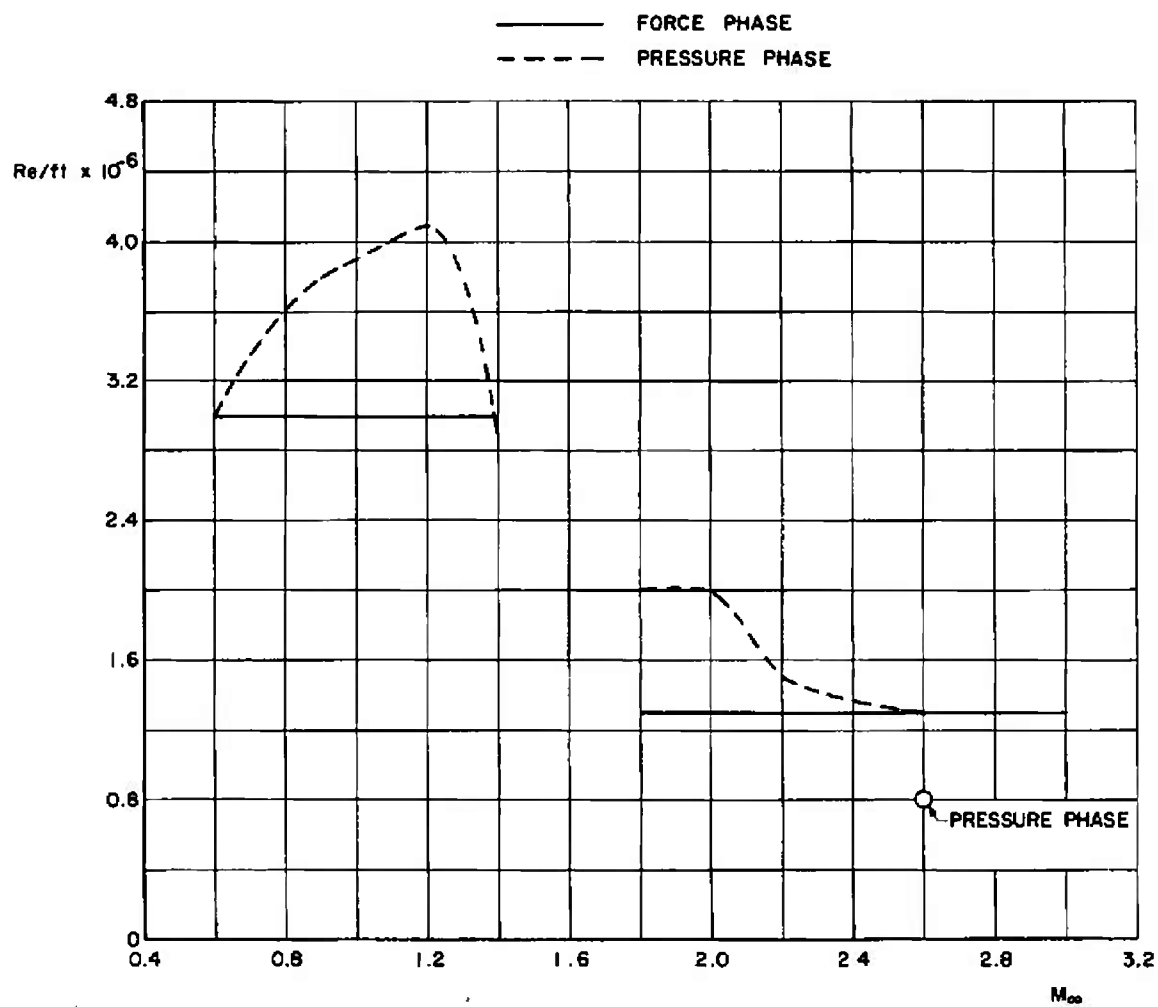
Fig. 8 Variation of Reynolds Number with Mach Number
