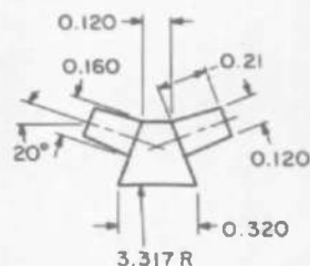
c. Sketch of Attitude Control Rockets and Horizon Sensor
