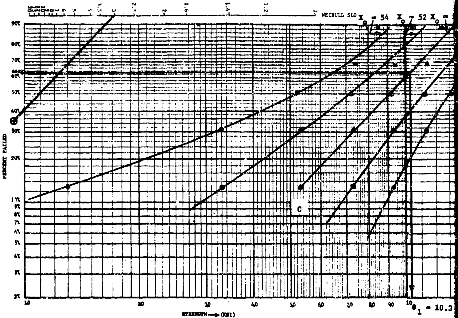
Figure 6.8 Modified Weibull Plot for D 6AC Steel, Life of 10^6 Cycles, Fatigue
