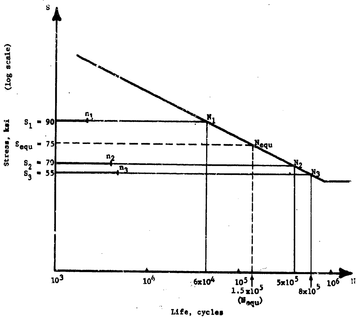
Figure 7.5 Miner's Rule
