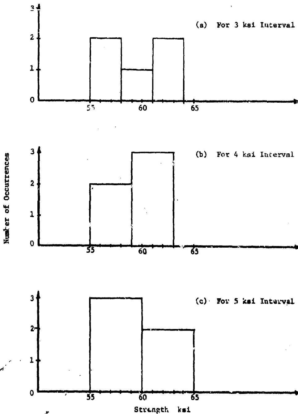
Figure 6.5 Histograms for Fatigue Strength of D_{6Ac} Steel at 800F for 10^6 Life Cycles
