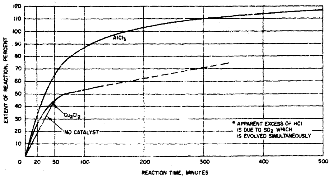
Figure 11. Rate of HCl evolution from catalyzed polyphenylene 4,4'-diphenyl ether disulfonyl chloride mixtures in trichlorobenzene at 210°C.
