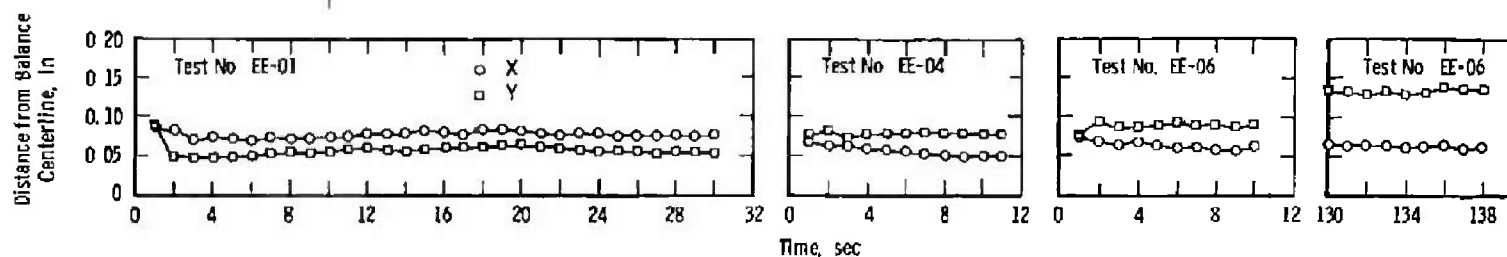
a. Variation of Thrust Vector Intercept Components in the Gimbal Plane
