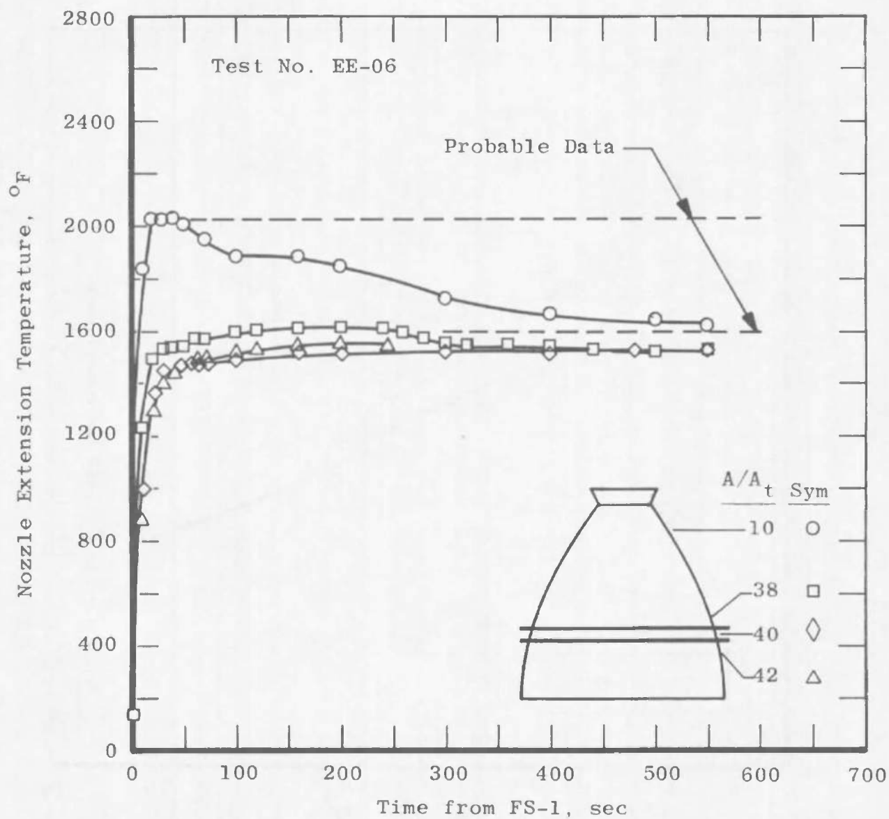
Fig. 29 Nozzle Extension Temperature History
