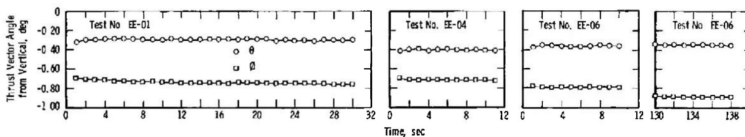
b. Angular Variation of Thrust Vector Components
