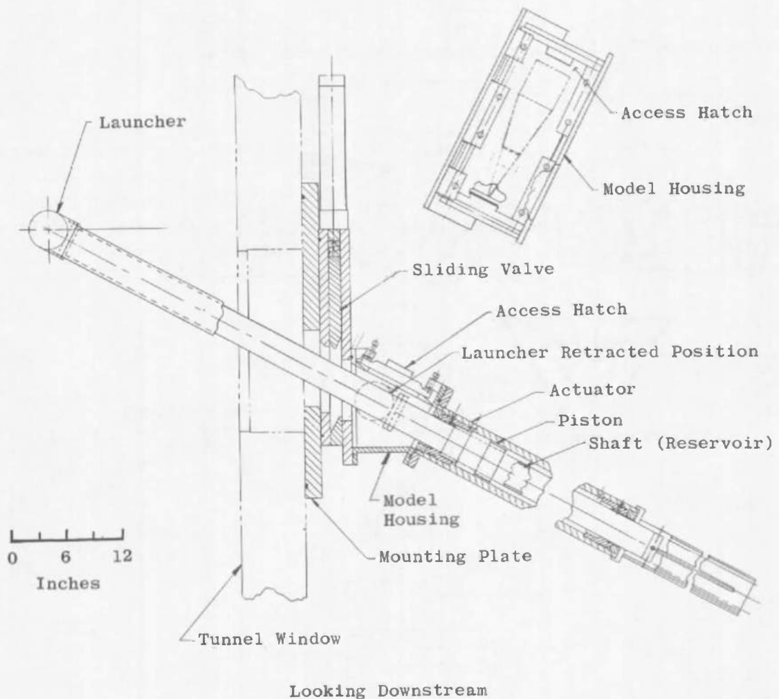
Fig. 5 Tunnel A Launcher Support System
