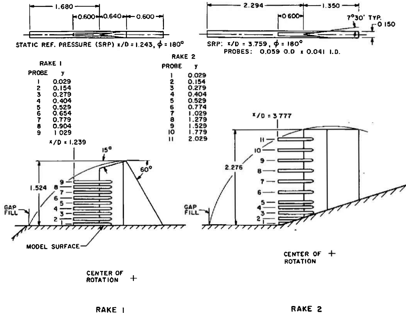
a. Rakes 1 and 2 Fig. 4 Details of Boundary-Layer Rakes
