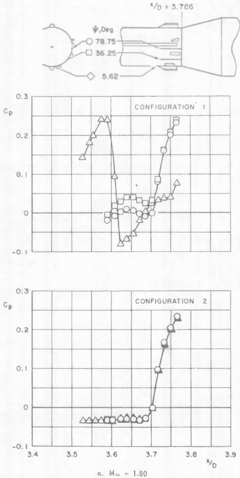
Fig. 7 Pressure Coefficient Distribution in the S-IVB Flare Region, Showing Protuberance and Interstage Effects, \alpha = 0
