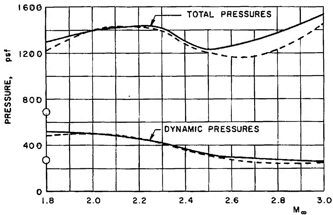
b. Total and Dynamic Pressures
