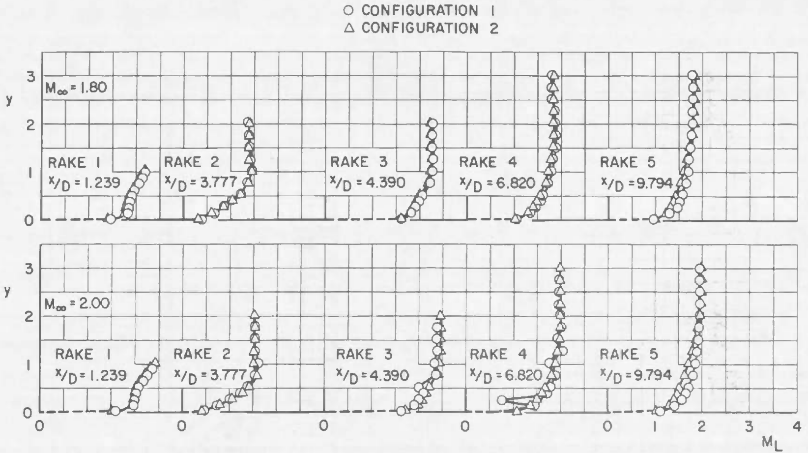
Fig. 9 Boundary-Layer Profiles for Configurations 1 and 2
