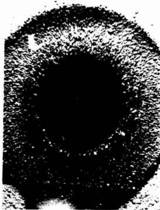
Fig. 23. Appearance of overcoated segments from tube B-133 after 230 hours (10x magnification). (a) Anode end and (b) cathode end of typical bore segment. (c) Cathode end of segment in the anode constriction.
