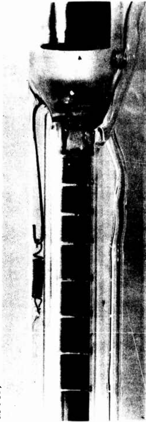
Fig. 22. Appearance of quartz envelope and bore segments at the anode end of tube B-133 after 230 hours.
