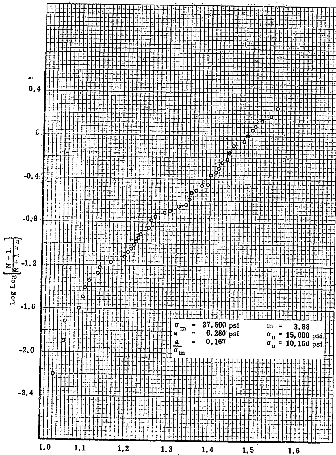
Figure 38. \text{Log Log} \left[ \frac{N+1}{N+1-n} \right] versus \text{Log} (\sigma - \sigma_u) with \sigma_u = 15,000 psi for Type IV Alumina Specimens
