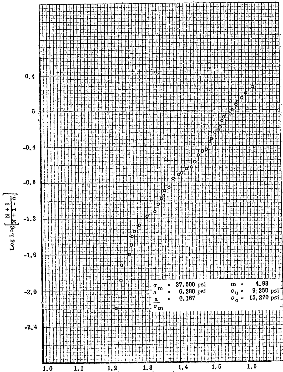
Figure 37. \text{Log Log} \left[ \frac{N+1}{N+1-n} \right] versus \text{Log} (\sigma - \sigma_u) with \sigma_u = 9350 psi for Type IV Alumina Specimens
