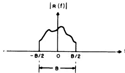
(a) ECHO PULSE MODULATION SPECTRUM
