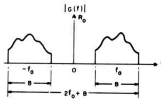
(b) SPECTRUM WITH SPATIAL CARRIER AND BIAS
