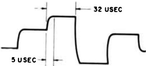
SIGNAL TO CRT ASSEMBLY
