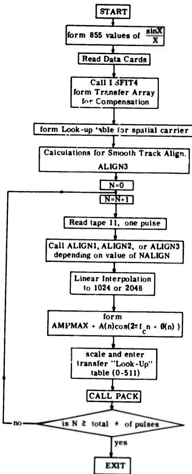
Flow Chart for Optical Processor Program.
