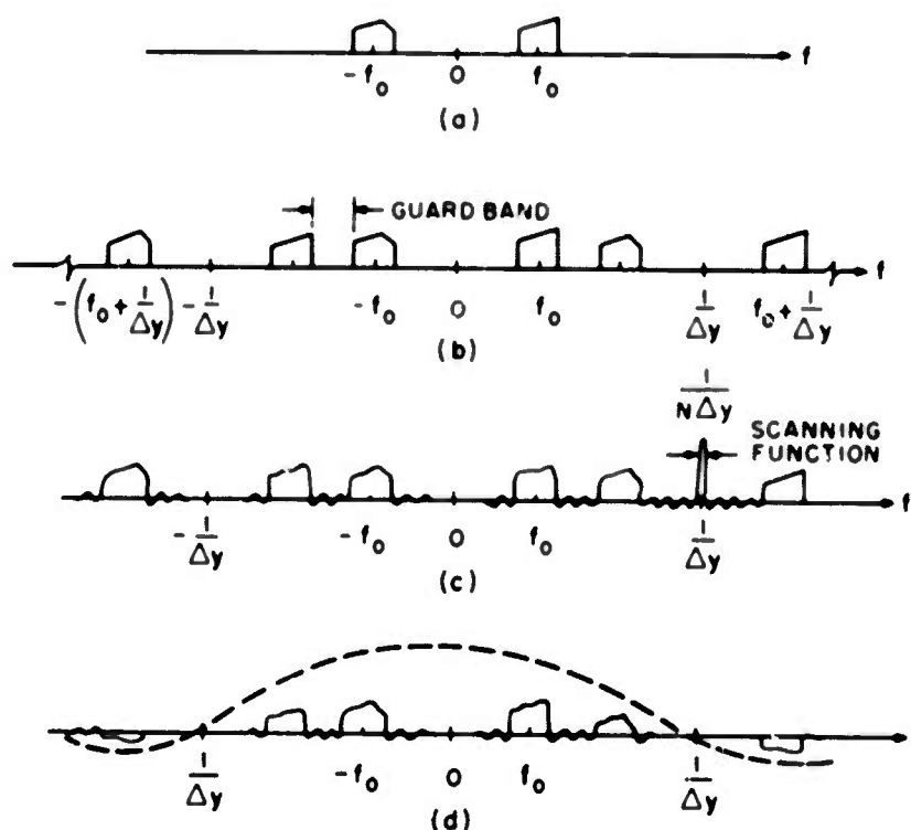
Figure 7. Effects of Sampling
