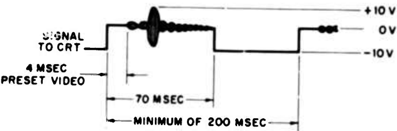
VIDEO-PICTURE ELEMENTS (TYPICAL, FOR 2048 WORDS PER LINE)
