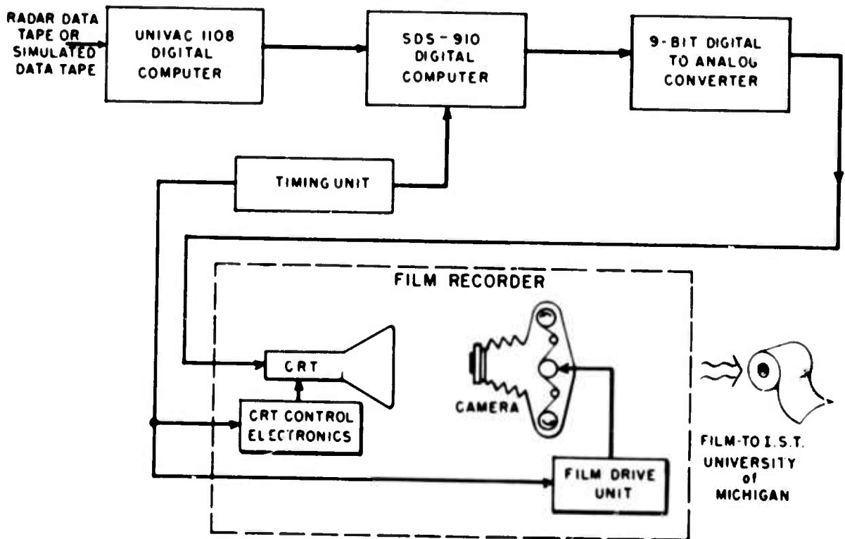
Figure 2. Optical Processor for Synthetic Spectrum Data
