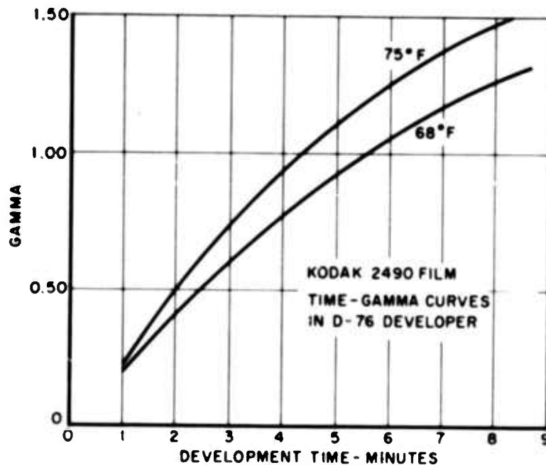
Figure 13 . Gamma vs Development Time
