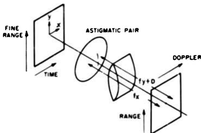
Figure 22. Simplified Processor Diagram
