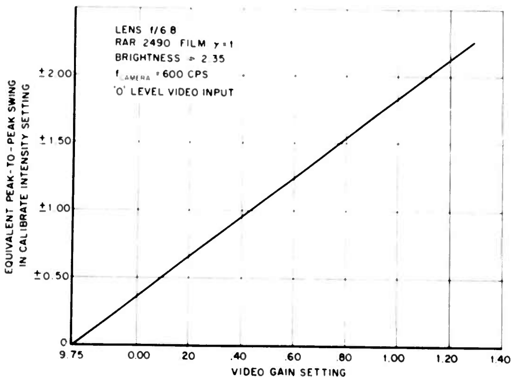
Figure 16 . Dynamic Swing of the Video Input Signal
