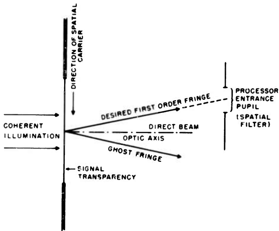
Figure 6. Diffraction Pattern Introduced by the Spatial Carrier
