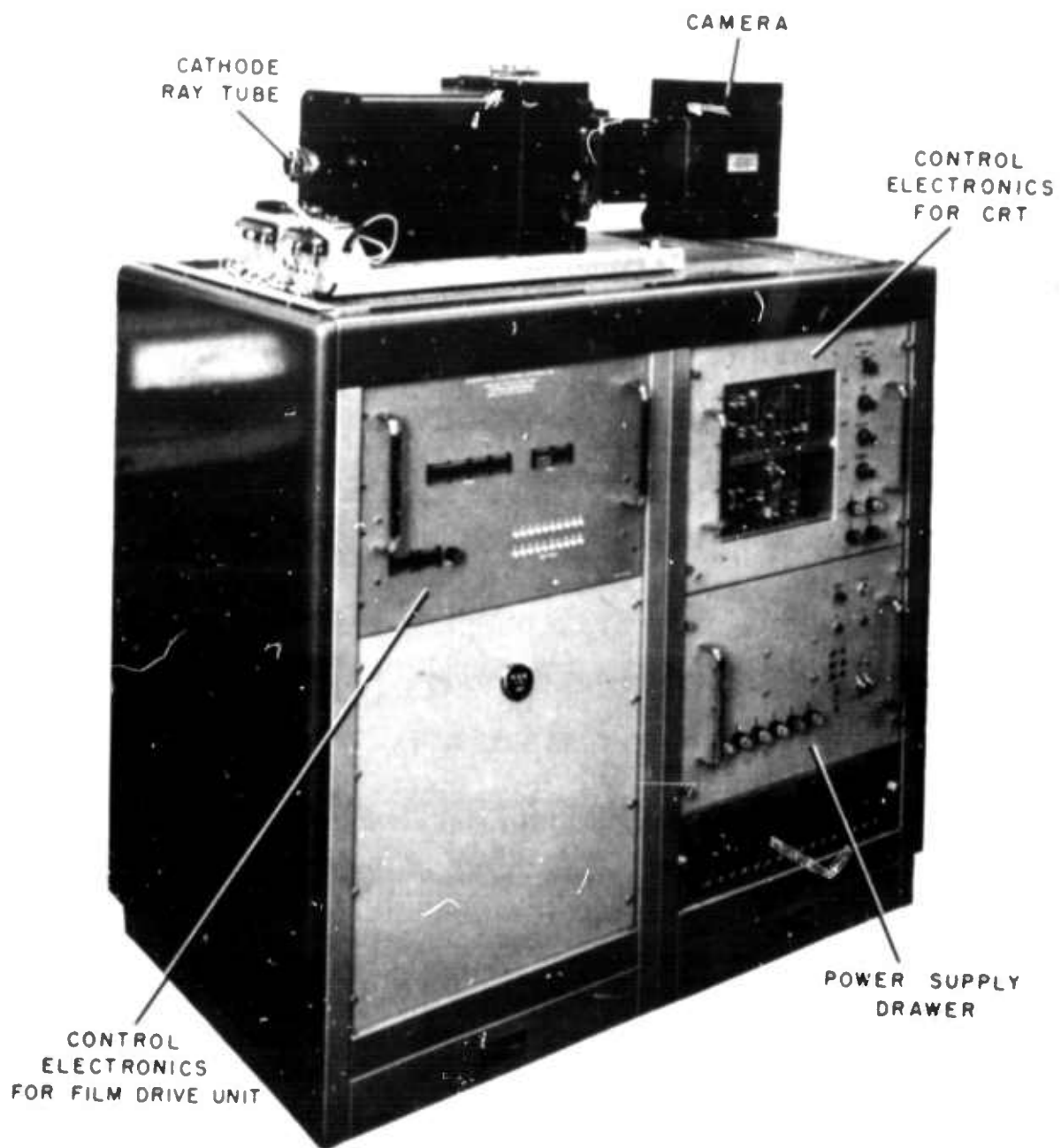
Figure 1. Film Recorder for Synthetic Spectrum Data
