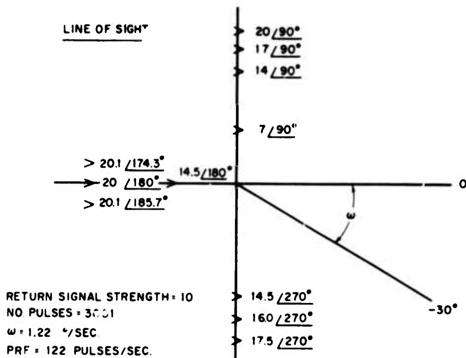
Figure 18. Michigan 11 - Element Target
