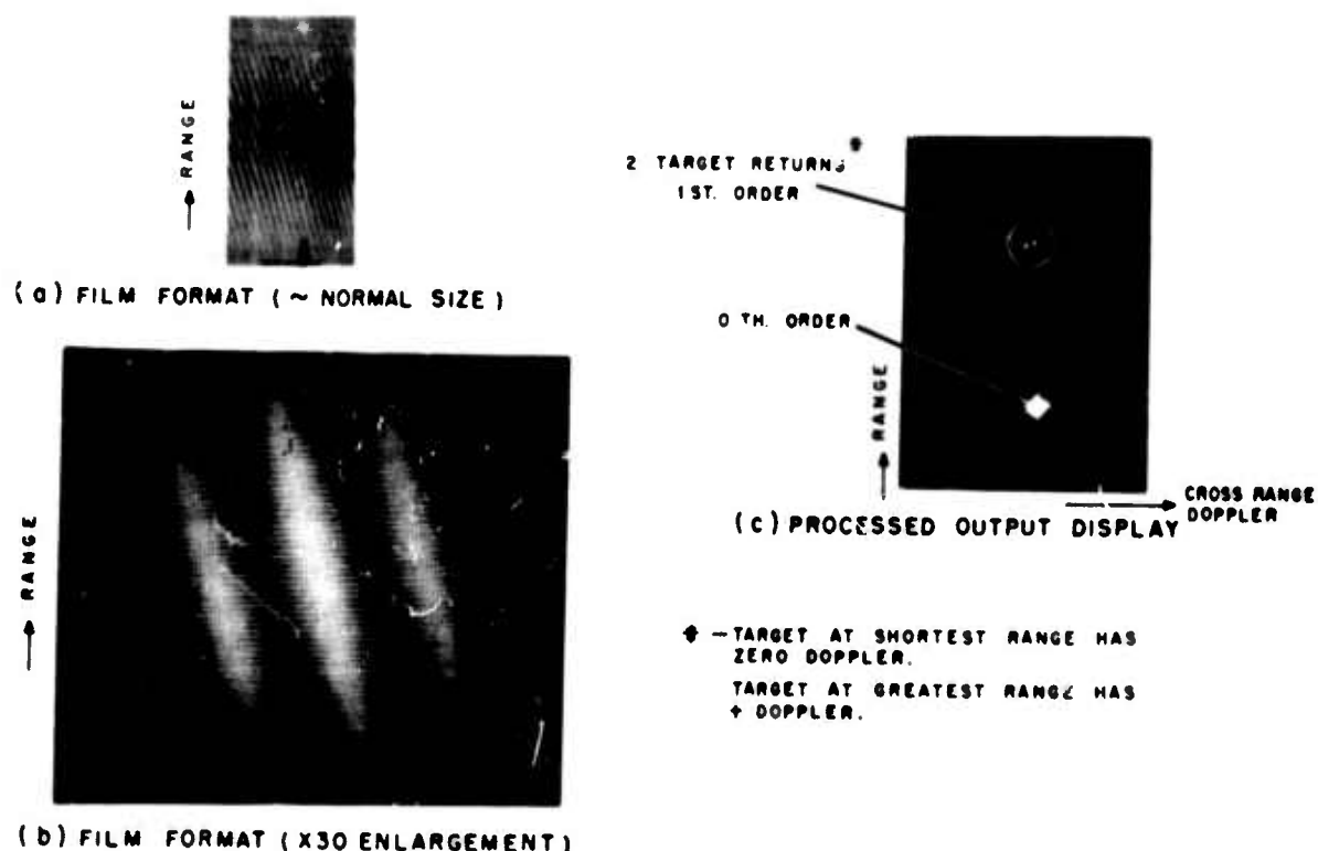
Figure 3. Typical Film Recording and Processed Output-Format II
