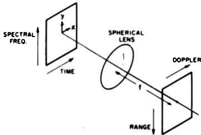
Figure 24. Simplified Processor Diagrams
