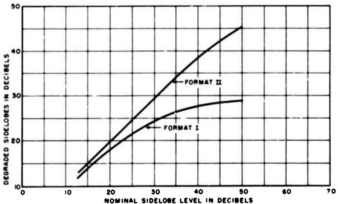
Figure 27. Sidelobes Will Be Below The Degraded Sidelobe Level for 99.9% Of The Time For A System Designed To Yield A Given Nominal Sidelobe Level
