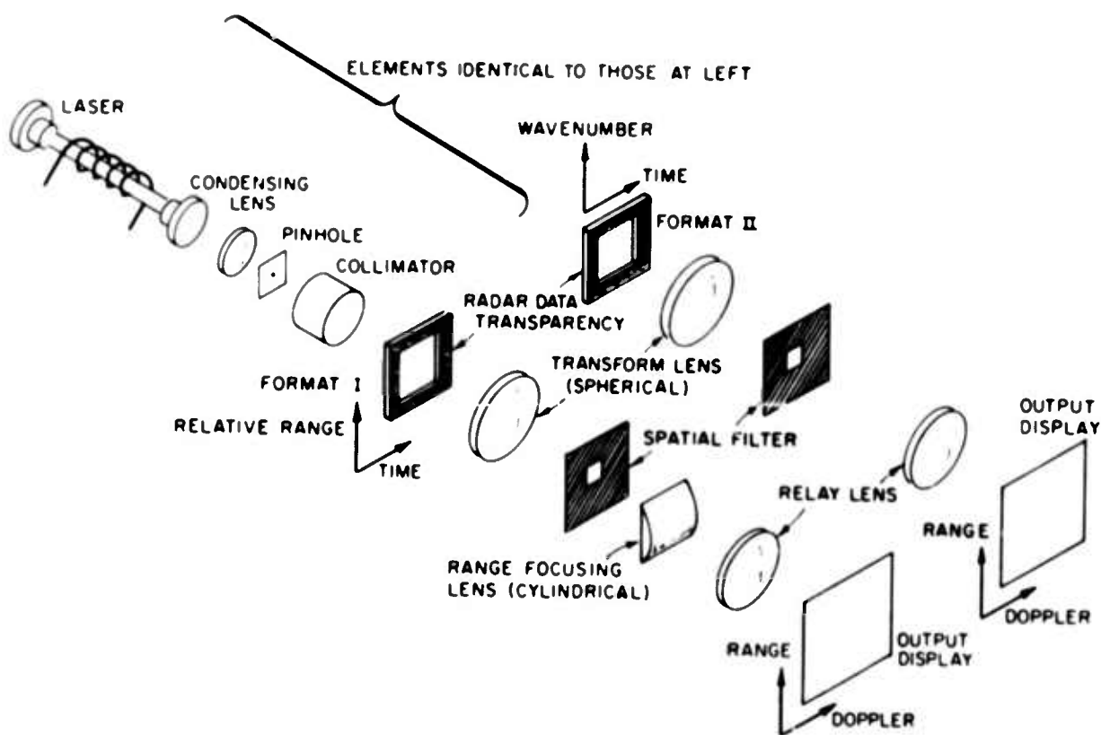
Figure 4. Basic Optical Processor Schematic
