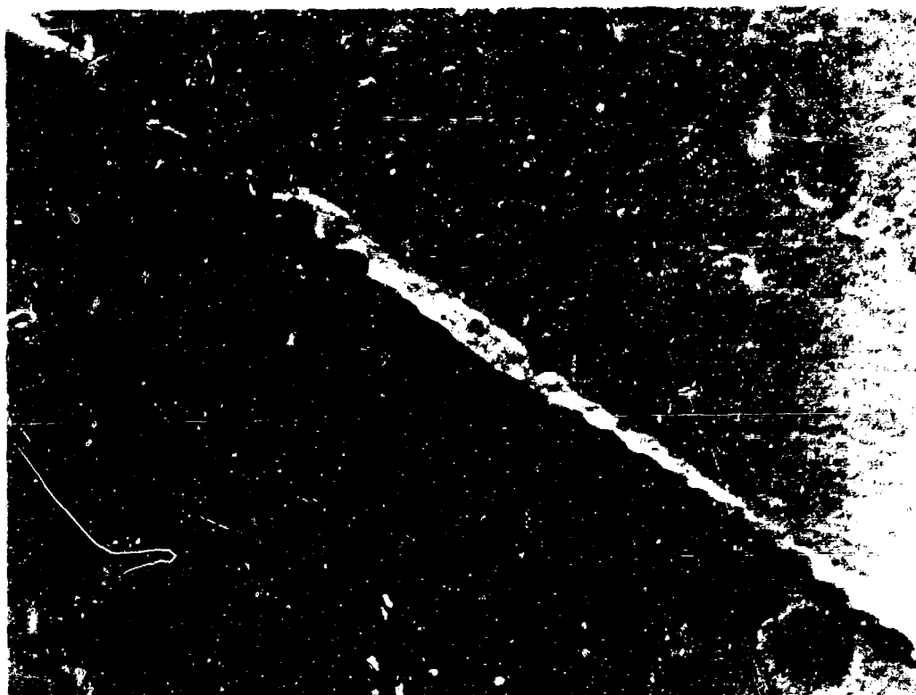
Figure 45. Microstructures of L-605 specimen after test at 1200° F and 65,000 psi. Rupture life 5.1 hours.
