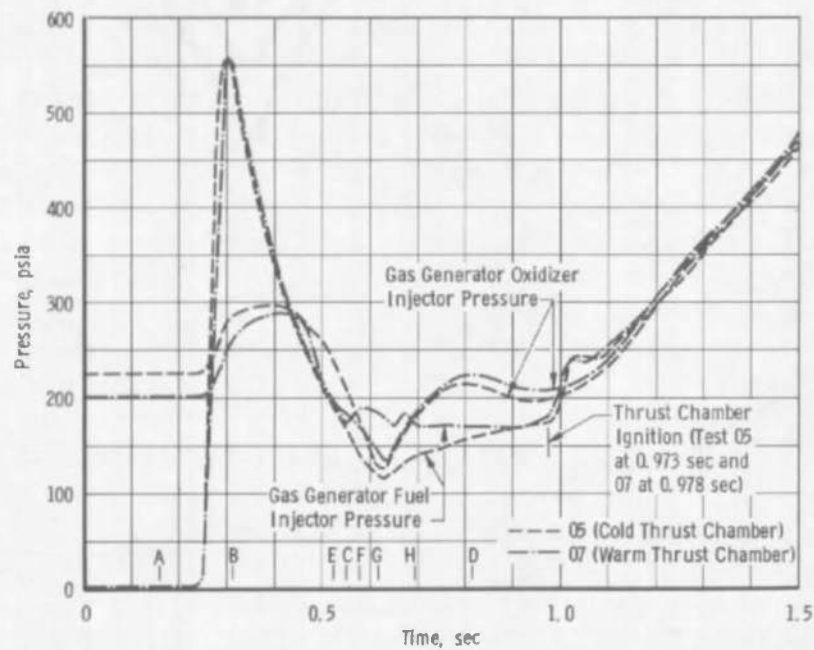
b. Gas Generator Fuel and Oxidizer Injector Pressures
