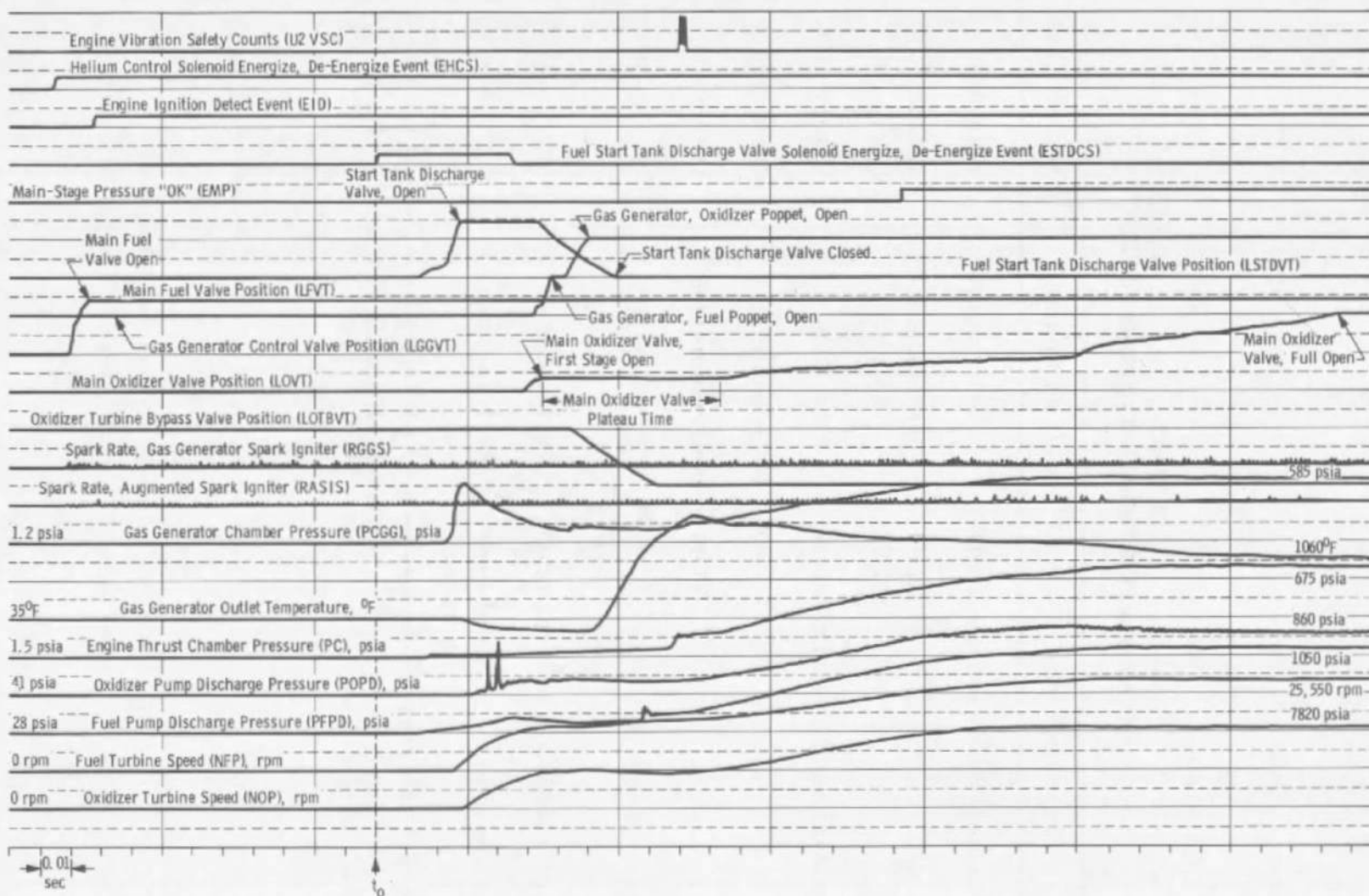
Fig. 17 Selected Engine Parameters for a Typical J-2 Transient
