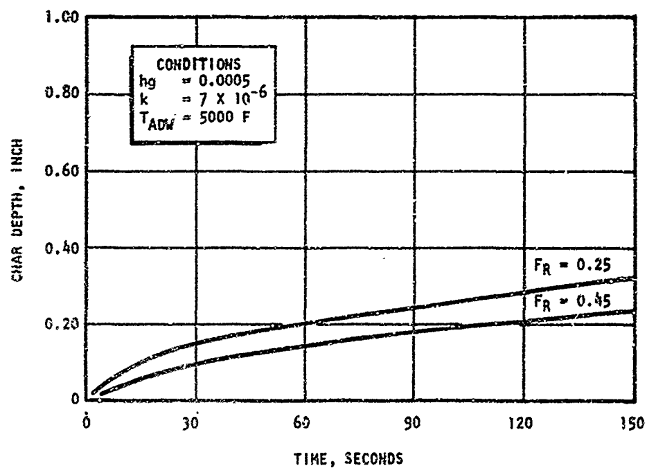
Figure 37. Effect of Resin Fraction on Char Front Advance For Low Thermal Conductivity and Low Heat Transfer Coefficient
