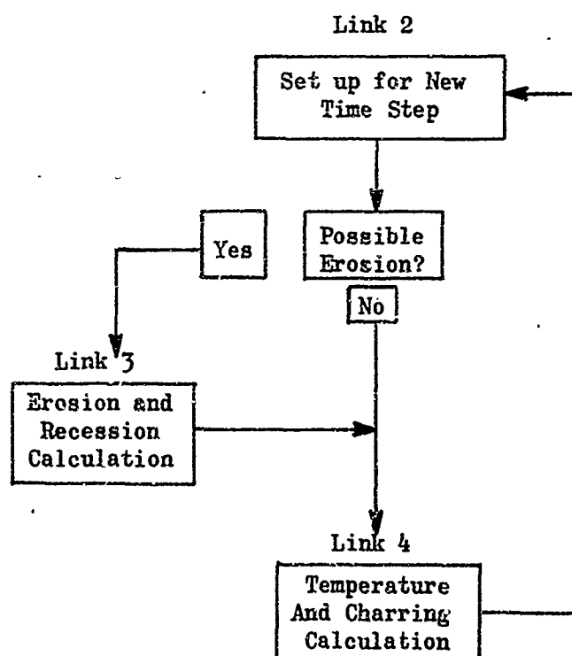
(b) Program flow in Link 2
