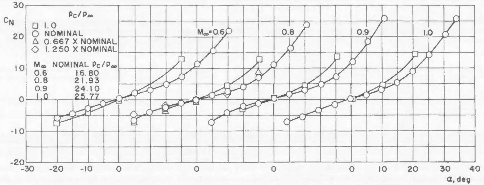
Fig. 8 Effect of Jet Pressure Ratio on Normal-Force Coefficient for Various Mach Numbers throughout the Angle-of-Attack Range, \beta = 0^\circ
