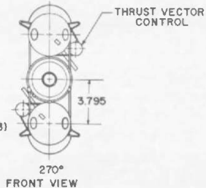
Fig. 2 Model Details
