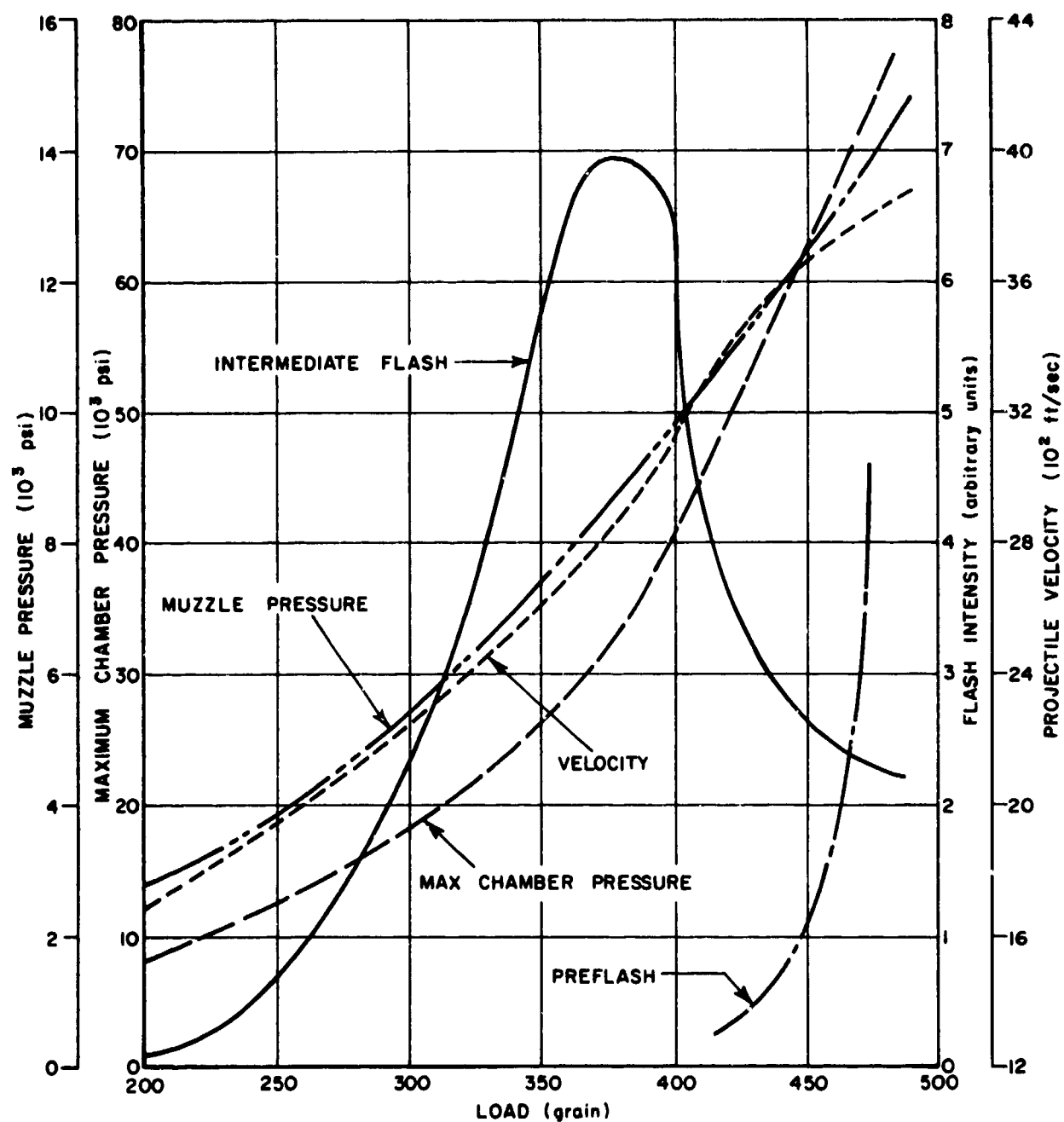
FIGURE 2 — 7 — EFFECT OF LOAD ON VELOCITY, PRE-FLASH, INTERMEDIATE FLASH, MUZZLE PRESSURE, AND MAXIMUM CHAMBER PRESSURE, (FROM REF. 9b)
