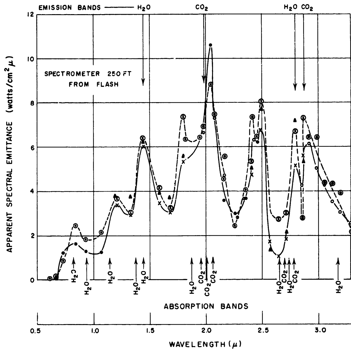
FIGURE 3—8—APPARENT SPECTRAL EMITTANCE OF UNSUPPRESSED FLASH FROM 280-MM GUN (FROM REF. 8d)
