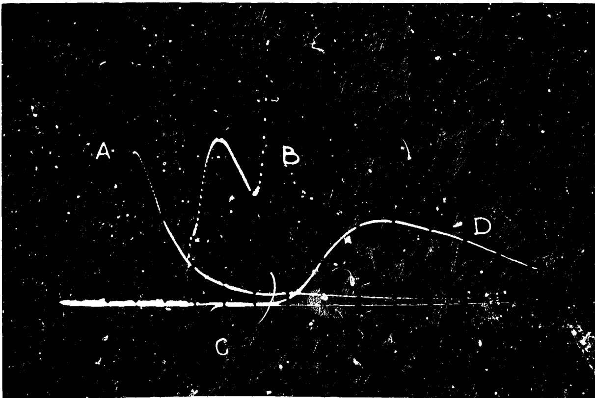
FIGURE 4-3—VARIATION OF BREECH PRESSURE AND FLASH INTENSITY WITH TIME (FROM REF. 4b)
