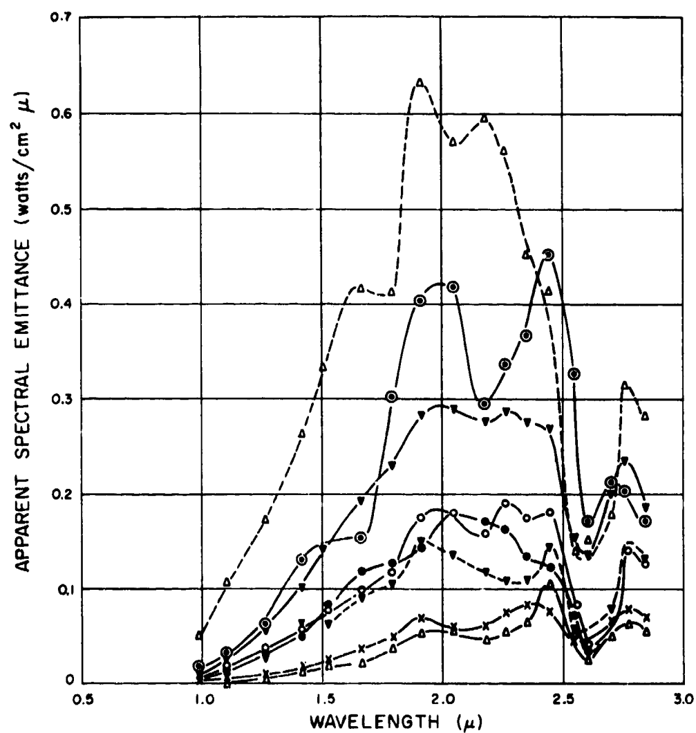
FIGURE 3—10—APPARENT SPECTRAL EMITTANCE OF FLASH FROM LARGE CALIBER WEAPONS (FROM REF. 8a) (B) \lambda = 0.99 TO 2.84 \mu . SEE TABLE 3—8(B) INTERMEDIATE FLASH
