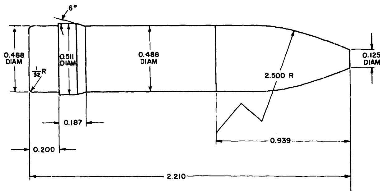
FIGURE A-1—SPECIAL ARTILLERY-TYPE, BANDED STEEL PROJECTILE
