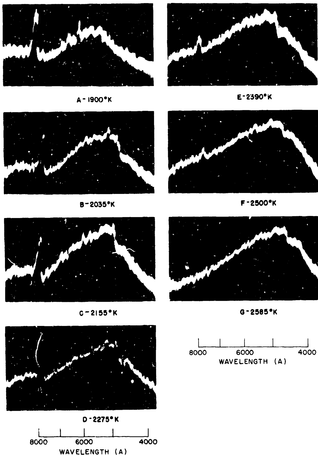
FIGURE 4-5 — SPECTRAL DISTRIBUTION OF SECONDARY FLASH SUPERIMPOSED ON CONTINUOUS BACKGROUND FROM TUNGSTEN FILAMENT AT VARIOUS TEMPERATURES (FROM REF. 5b)
