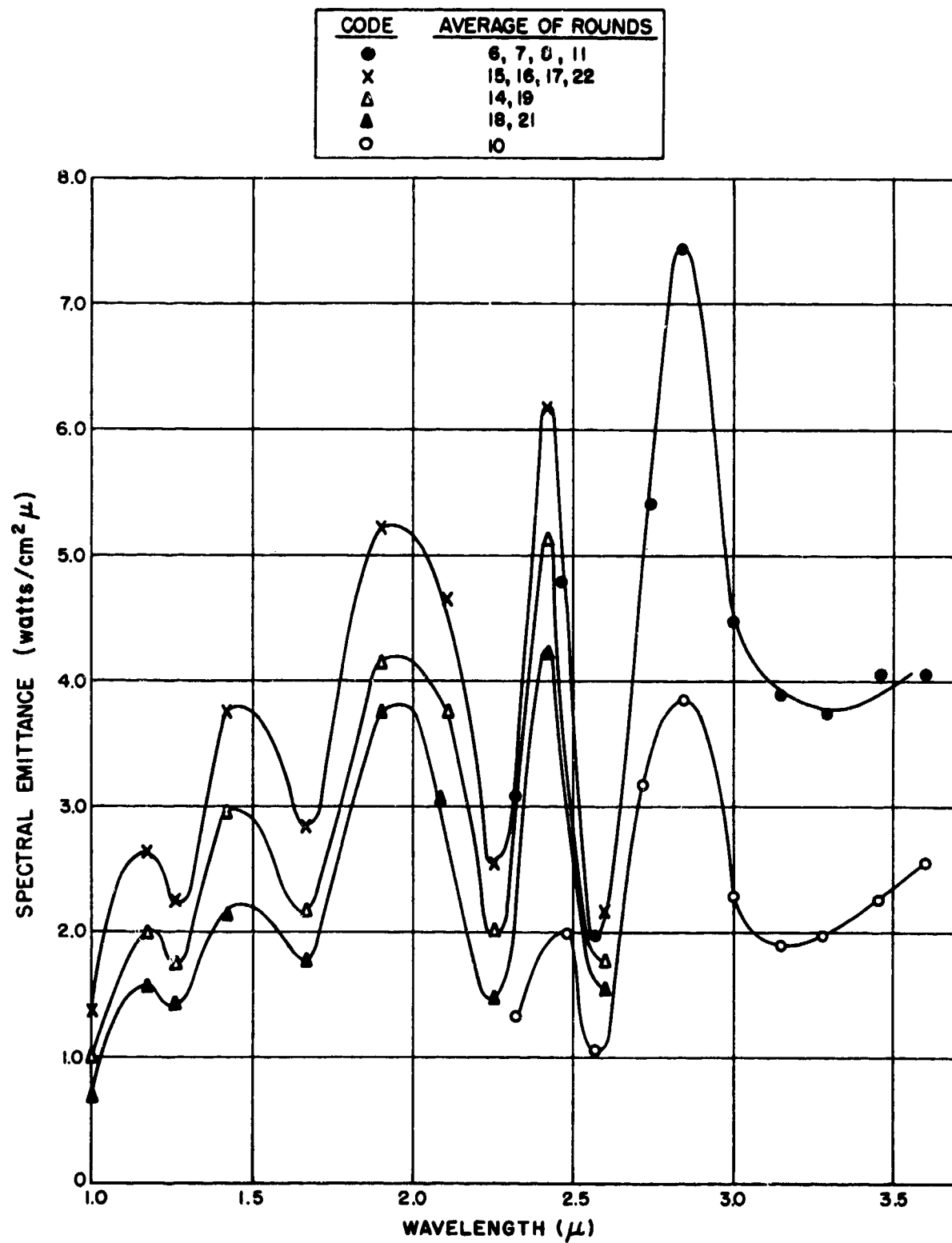
FIGURE 3 — 3 — SPECTRAL EMITTANCE OF UNSUPPRESSED FLASH FROM 155-MM GUN (FROM REF. 8a)
