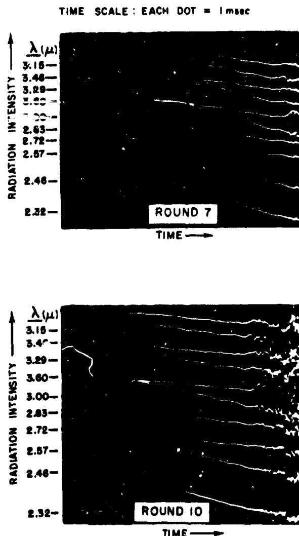
FIGURE 3-4—EXAMPLES OF SPECTROGRAPHIC RECORDS FOR UNSUPPRESSED FLASH (FROM REF. 8a) (155-MM GUN)
