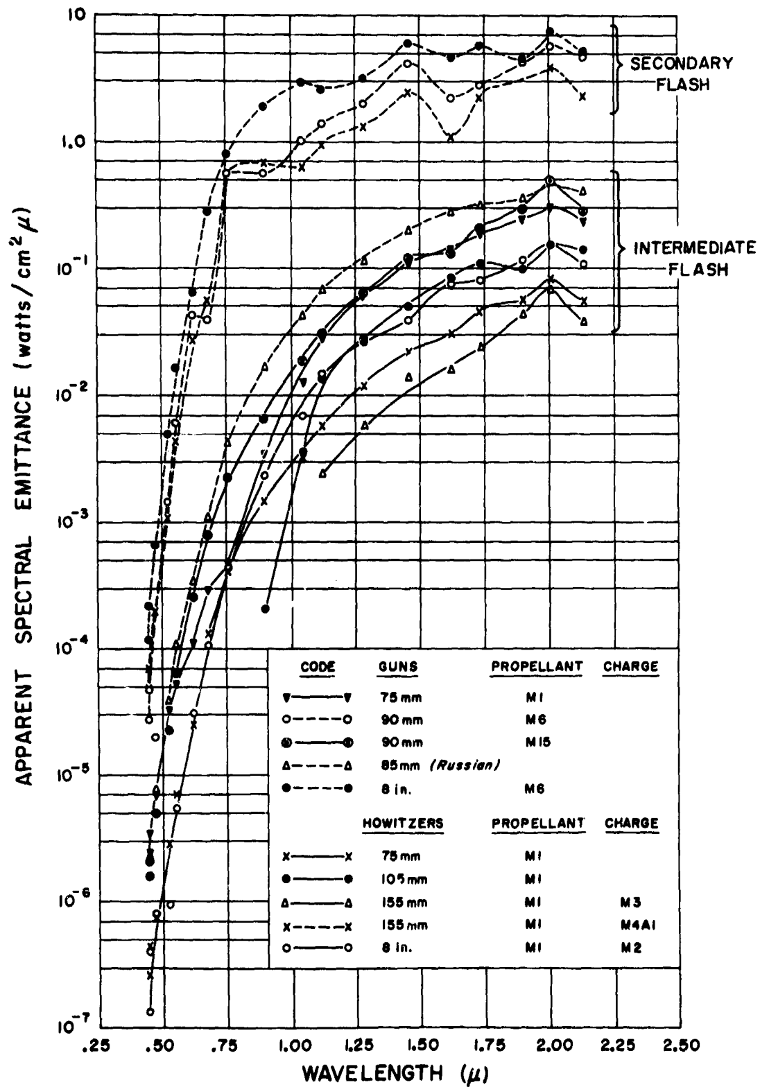
FIGURE 3-10—APPARENT SPECTRAL EMITTANCE OF FLASH FROM LARGE CALIBER WEAPONS (FROM REF. 8a) (A) \lambda = 0.41 TO 2.13\mu . SEE TABLE 3-8(A).
