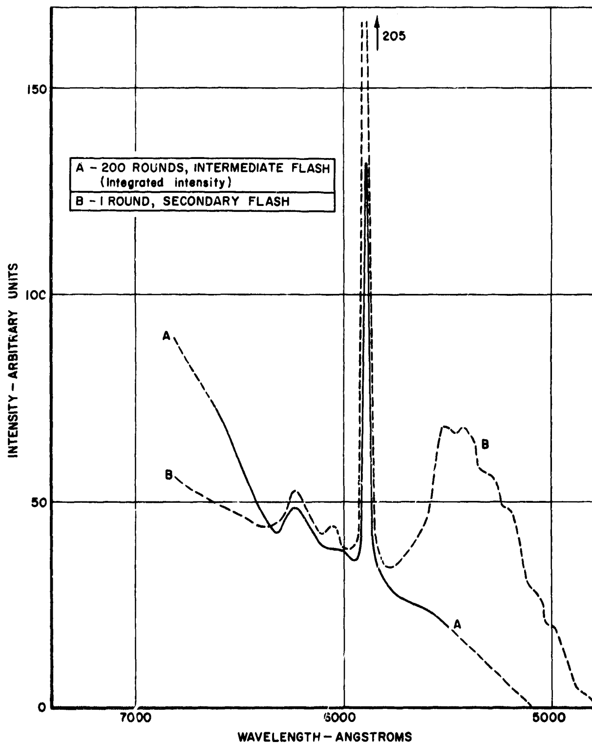
FIGURE 2-1 — COMPARISON OF VISIBLE SPECTRAL DISTRIBUTION OF INTERMEDIATE AND SECONDARY FLASH (FROM REF. 4a)
