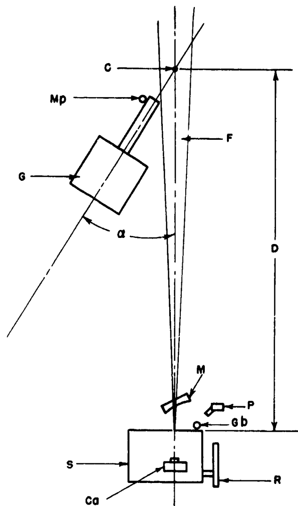
FIGURE 3-2—ARRANGEMENT OF FIELD-TEST EQUIPMENT FOR OBSERVING GUN FLASH (FROM REF. 8a)
