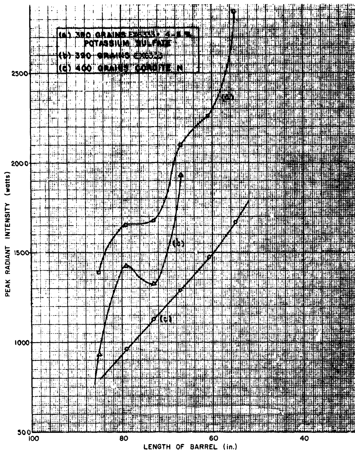
FIGURE 2—8— VARIATION OF PEAK RADIANT INTENSITY WITH BARREL LENGTH FOR VARIOUS CHARGES (FROM REF. 6c)
