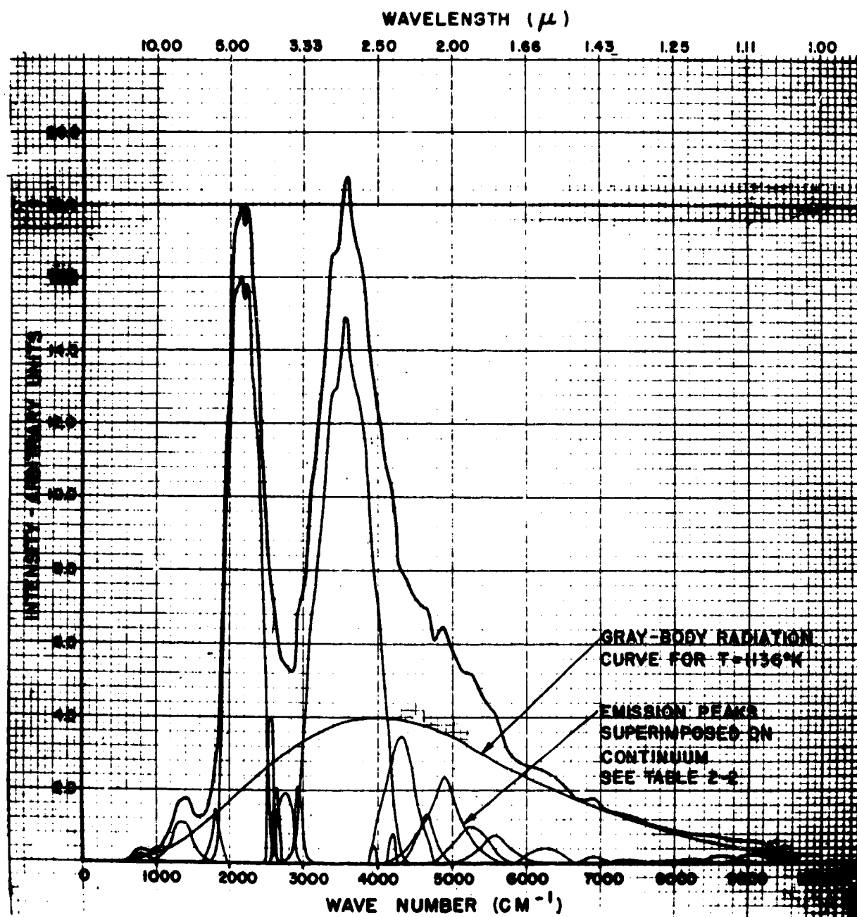
FIGURE 2-5—SPECTRAL DISTRIBUTION OF INFRARED RADIATION FROM SECONDARY FLASH (PLOTTED AGAINST WAVE NUMBER) (FROM REF. 6a)
