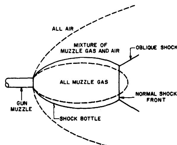
FIGURE 1-1—FLOW PATTERN AT A GUN MUZZLE (FROM REF. 11b)
