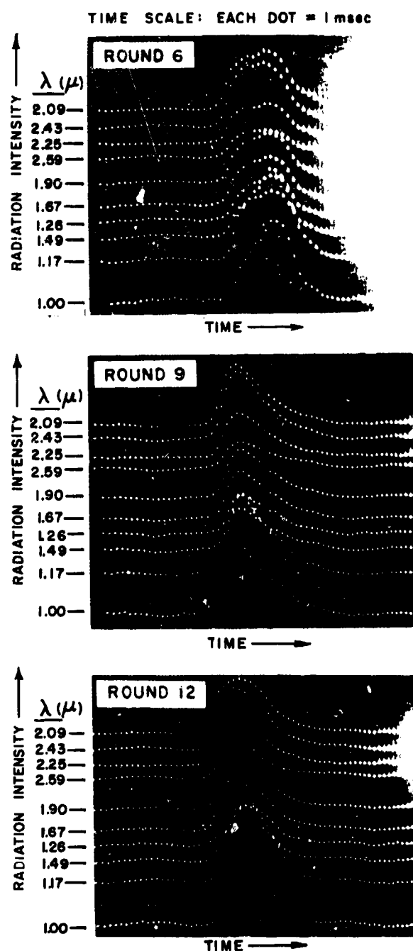
FIGURE 3—6—EXAMPLES OF SPECTROGRAPHIC RECORDS FOR SUPPRESSED FLASH (FROM REF. 8a) (155-MM GUN)
