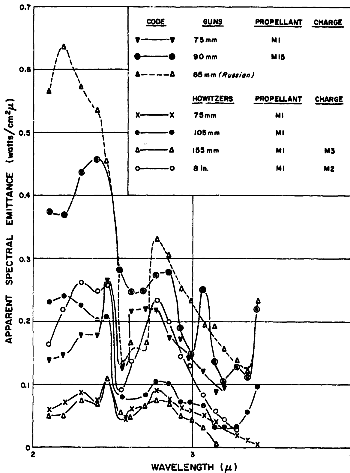
FIGURE 3 — 10 — APPARENT SPECTRAL EMITTANCE OF FLASH FROM LARGE CALIBER WEAPONS (FROM REF. 8a) (D) \lambda = 2.1 TO 3.40\mu . SEE TABLE 3 — 3(C) INTERMEDIATE FLASH
