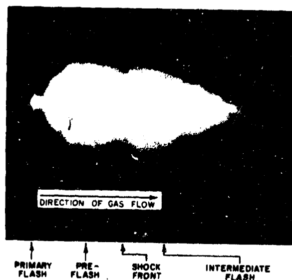
FIGURE 1—2—PRIMARY, INTERMEDIATE, AND PRE-FLASH (FROM REF. 5c)
