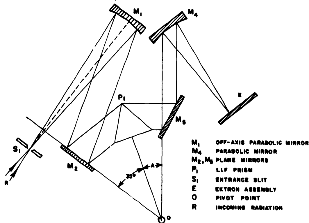
FIGURE A-7 — OPTICAL SYSTEM OF THE 18-CHANNEL SPECTROMETER (FROM REF. 8e)
