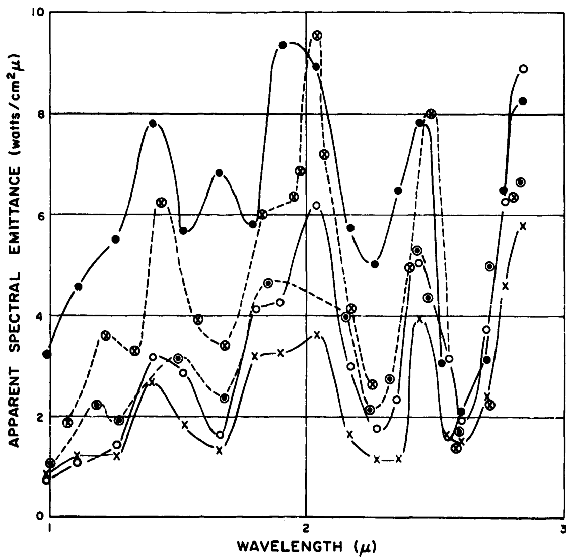
FIGURE 3-10 — APPARENT SPECTRAL EMITTANCE OF FLASH FROM LARGE CALIBER WEAPONS (FROM REF. 8a) (C) \lambda = 0.99 TO 2.84\mu . SEE TABLE 3 — 8(B) SECONDARY FLASH
