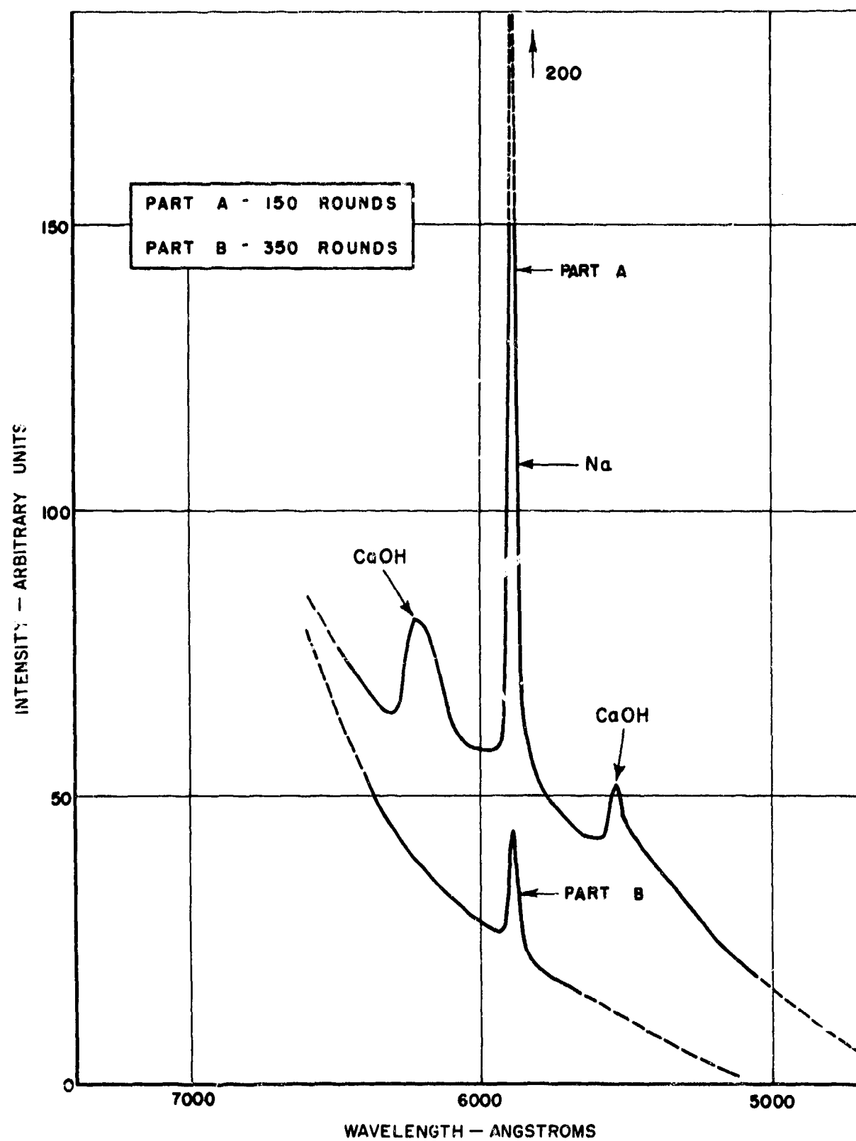
FIGURE 2 — 2 — VISIBLE SPECTRUM OF TWO COMPONENTS OF INTERMEDIATE FLASH (FROM REF. 5a)
