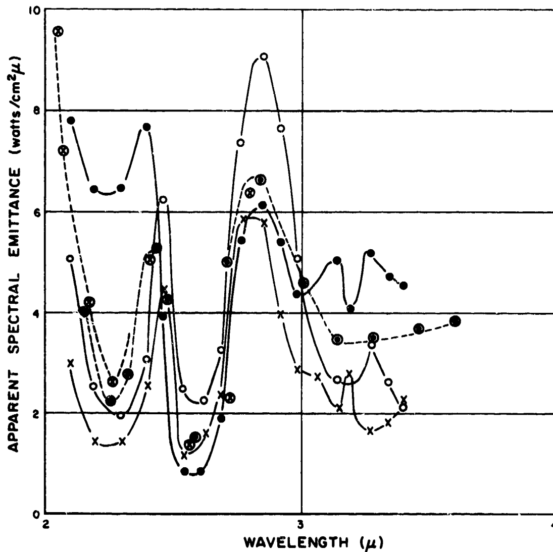
FIGURE 3-10—APPARENT SPECTRAL EMITTANCE OF FLASH FROM LARGE CALIBER WEAPONS (FROM REF. 8a) (E) \lambda = 2.1 TO 3.4\mu . SEE TABLE 3-8(C).
