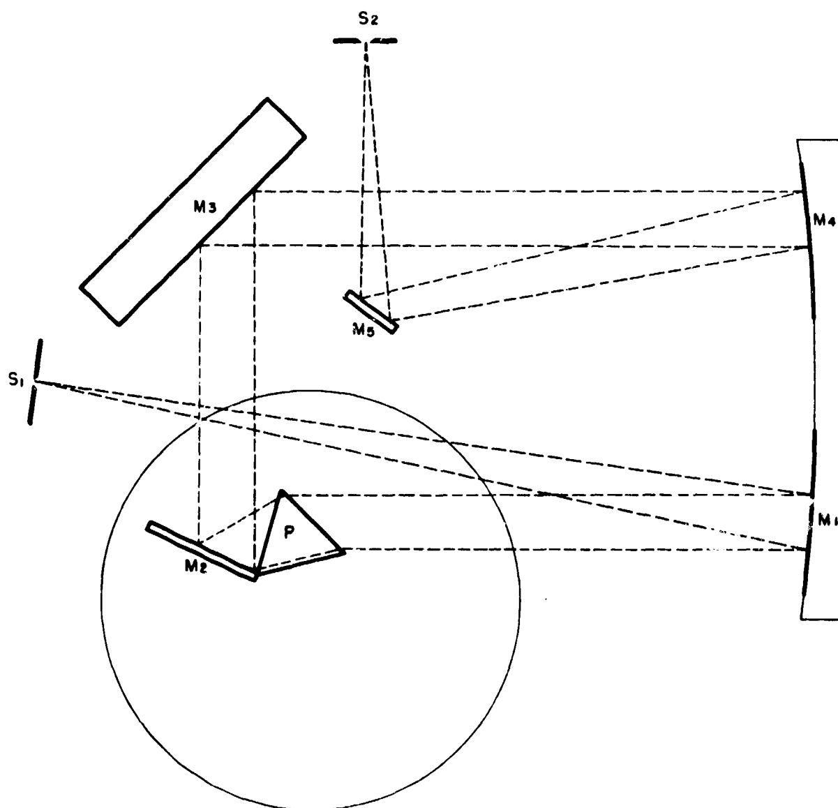
FIGURE A-2—SCHEMATIC DIAGRAM OF MONOCHROMATOR (FROM REF. 6a)
