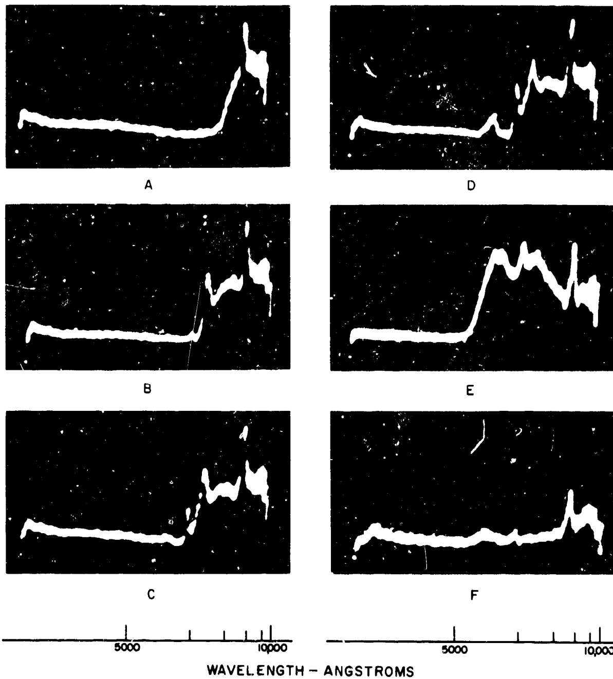
FIGURE 4 — 1 — VARIATION OF THE SPECTRAL DISTRIBUTION OF SECONDARY FLASH WITH TIME (FROM REF. 5a) FRAME TIMES WERE NOT INDICATED ON THE ORIGINAL, BUT SOME TIME INFORMATION IS GIVEN IN PAR. 4 — 1.
