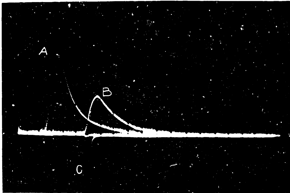
FIGURE 4-2 — VARIATION OF BREECH PRESSURE AND INTENSITY OF MUZZLE GLOW WITH TIME (FROM REF. 4b)
