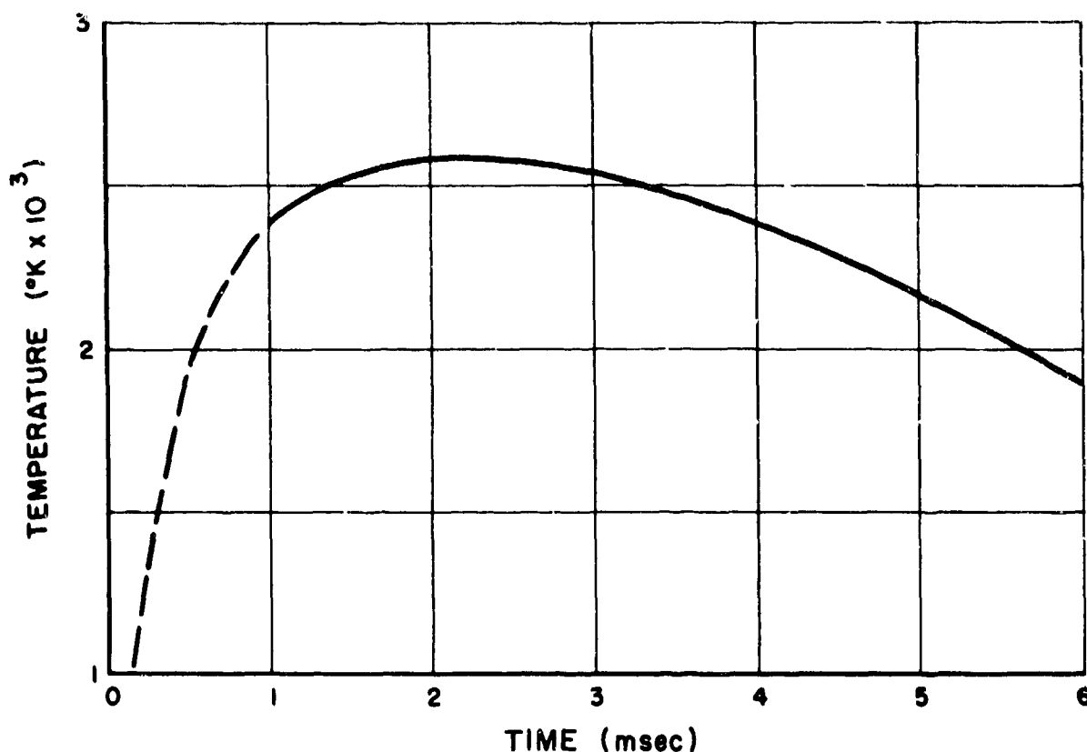
FIGURE 4-6—VARIATION IN TEMPERATURE OF SECONDARY FLASH WITH TIME (FROM REF. 5b)
