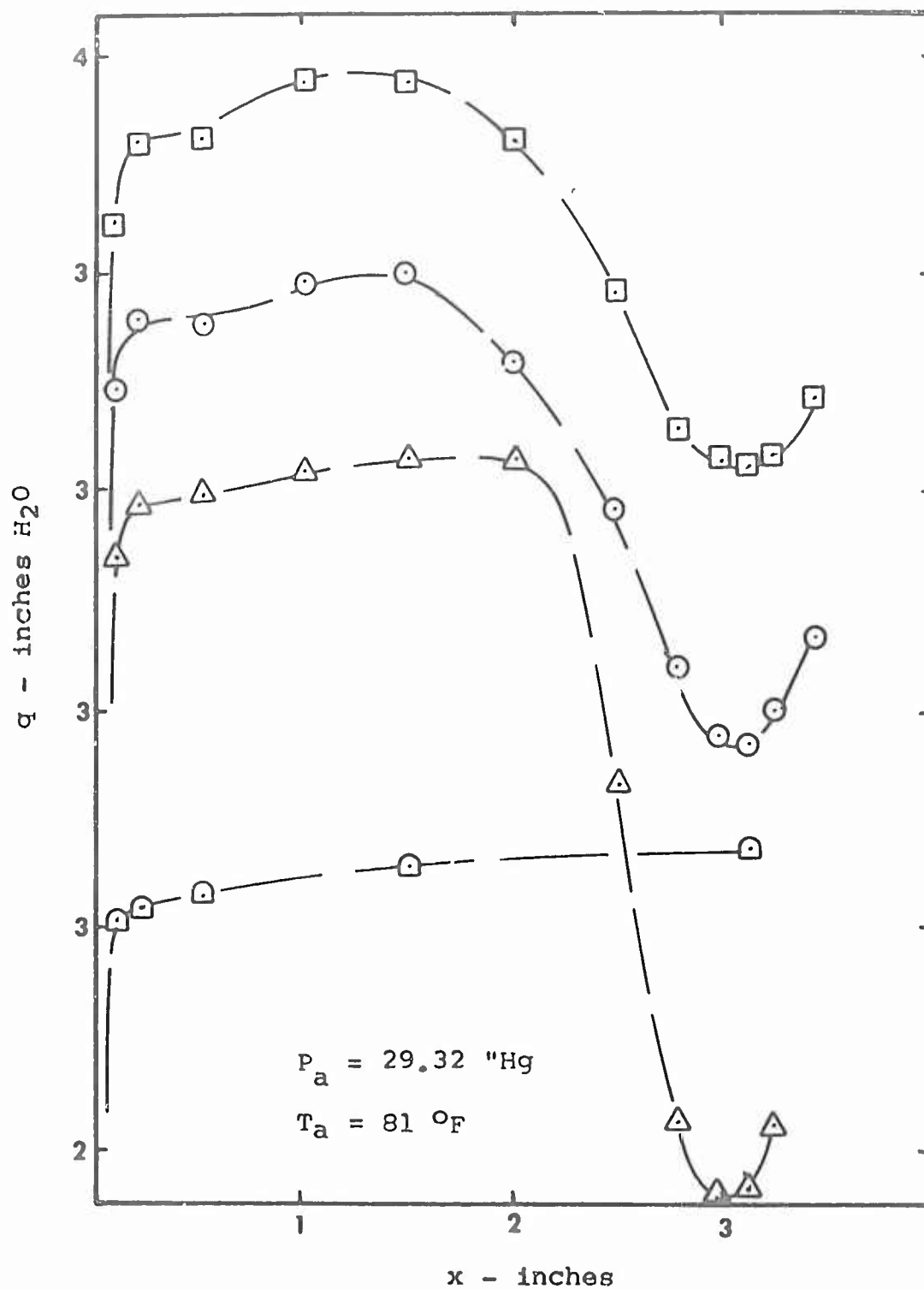
Figure 41 Dynamic Pressure vs. Distance from Wall Cyl. C v = 124.6 \text{ fps} I^2R/L = 260.5 \text{ Btu/hr-inch}
