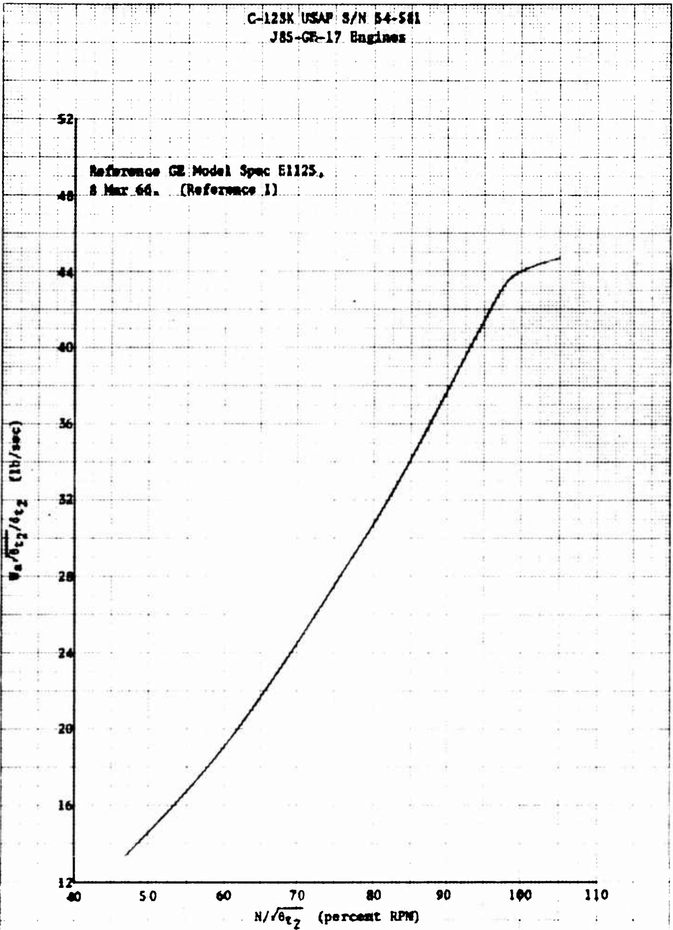
Figure 45. Corrected Airflow vs Corrected Engine Speed
