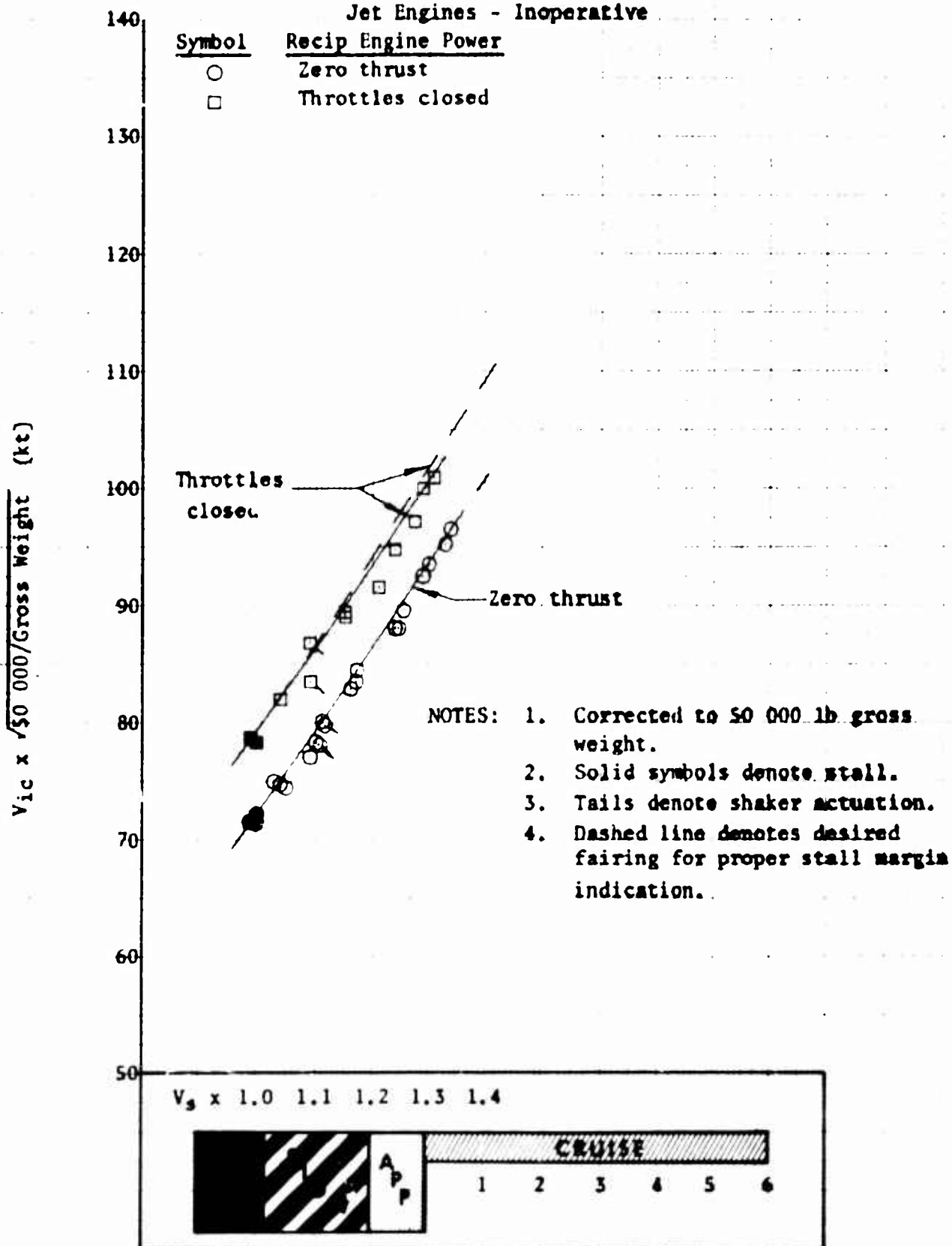
Figure 4. Stall Margin Indication vs Indicated Airspeed
