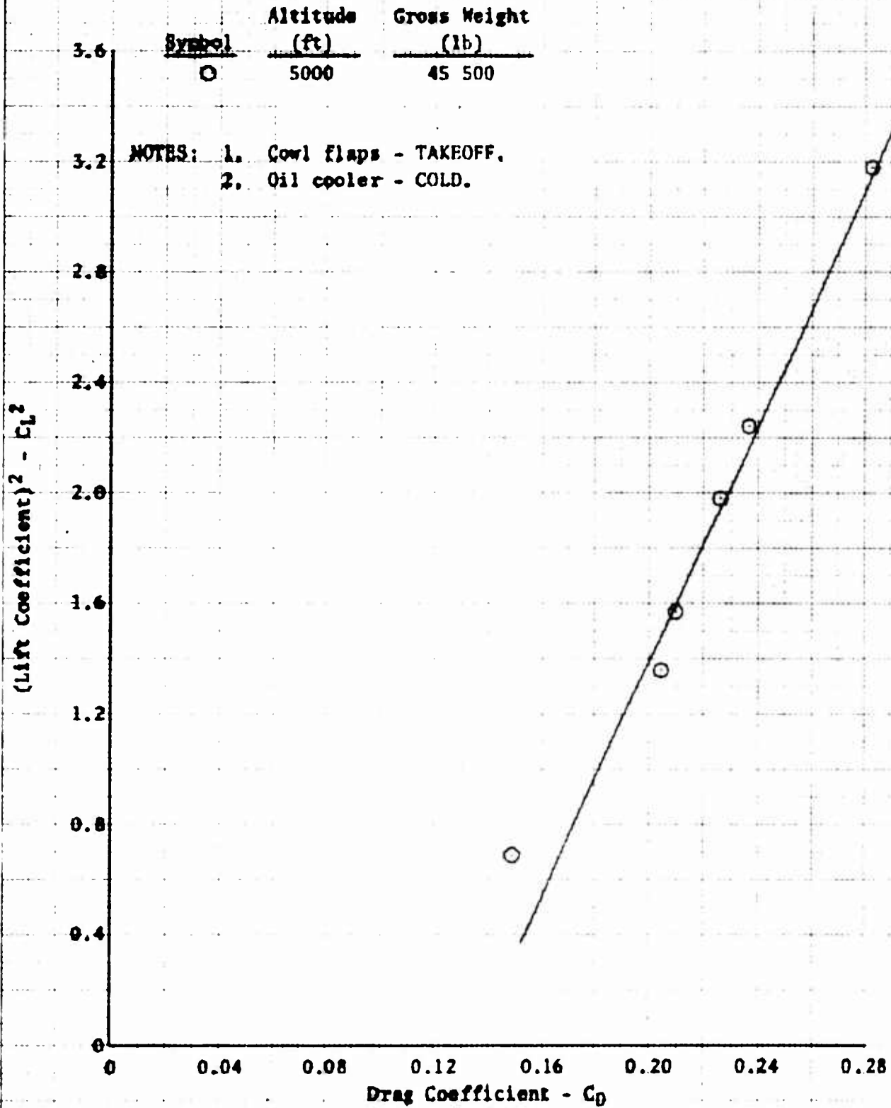
Figure 37. Drag Polar
