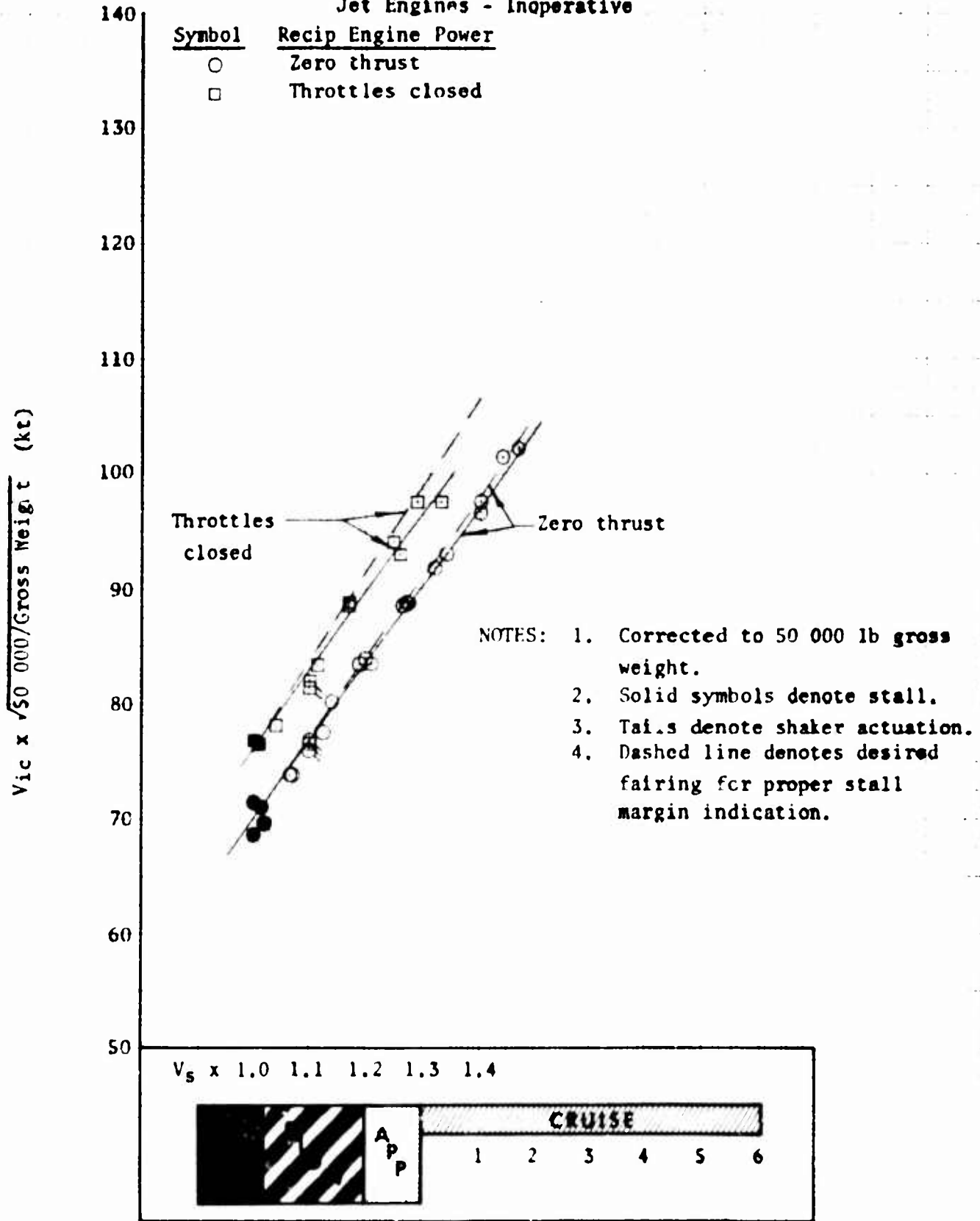
Figure 5. Stall Margin Indication vs Indicated Airspeed
