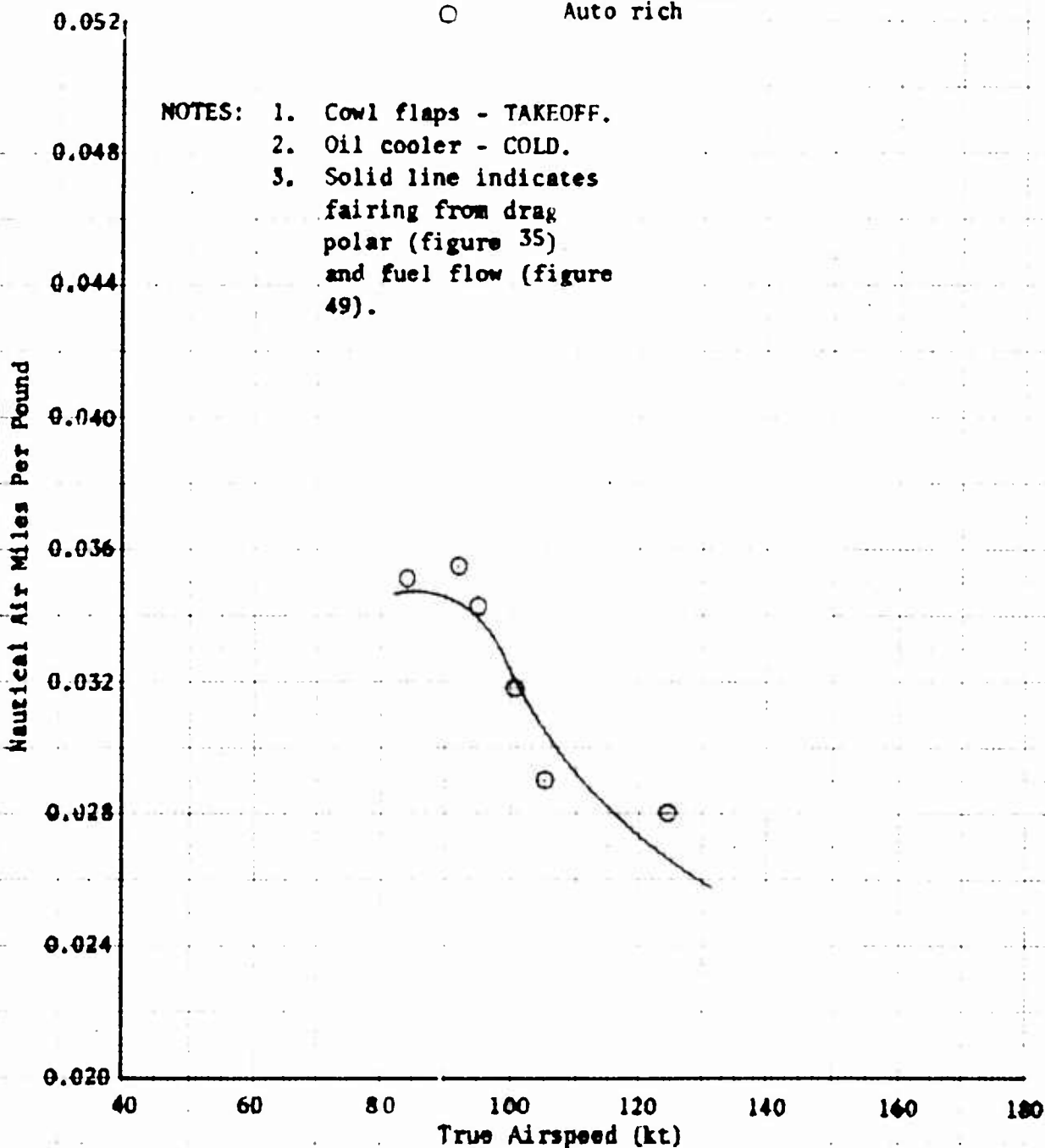
Figure 25. Specific Range
