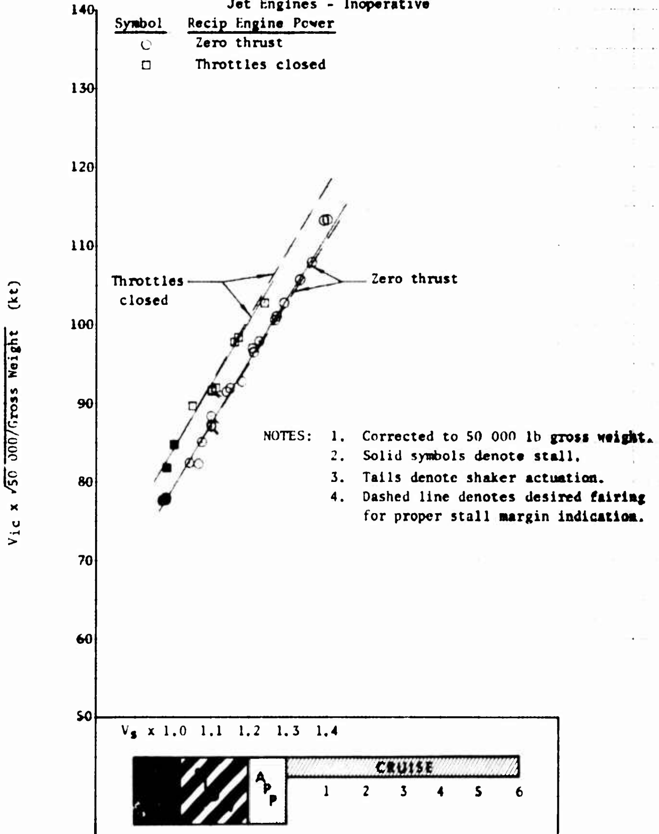
Figure 3. Stall Margin Indication vs Indicated Airspeed
