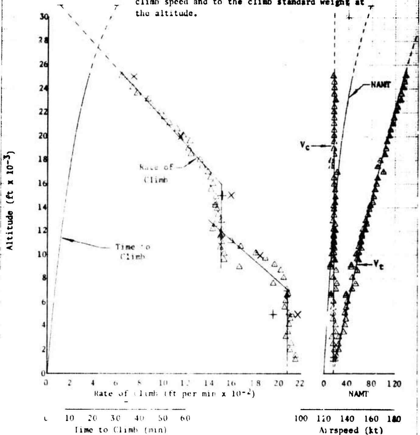
Figure 7. Climb Performance
