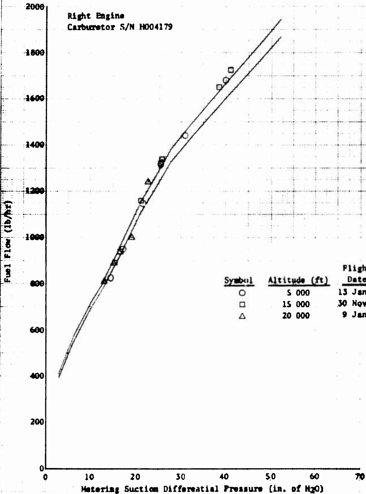
Figure 52. Carburetor Calibration
