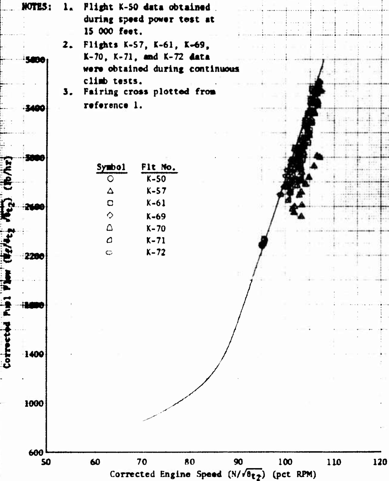
Figure 48. Corrected Fuel Flow vs Corrected Engine Speed
