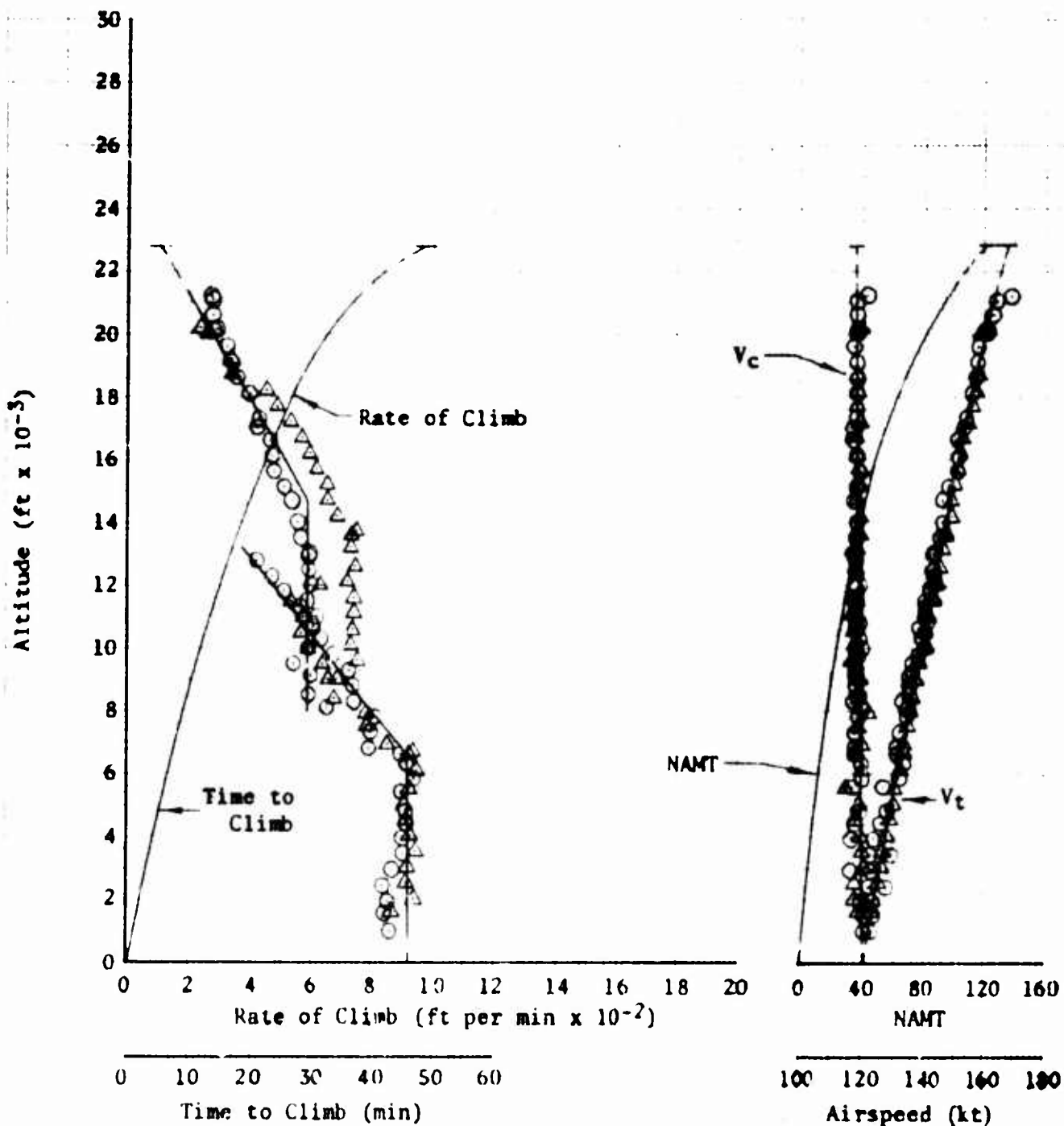
Figure 9. Climb Performance
