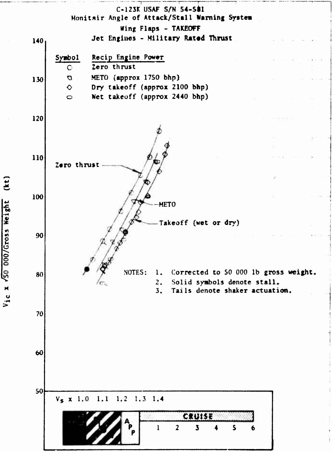
Figure 9. Stall Margin Indication vs Indicated Airspeed
