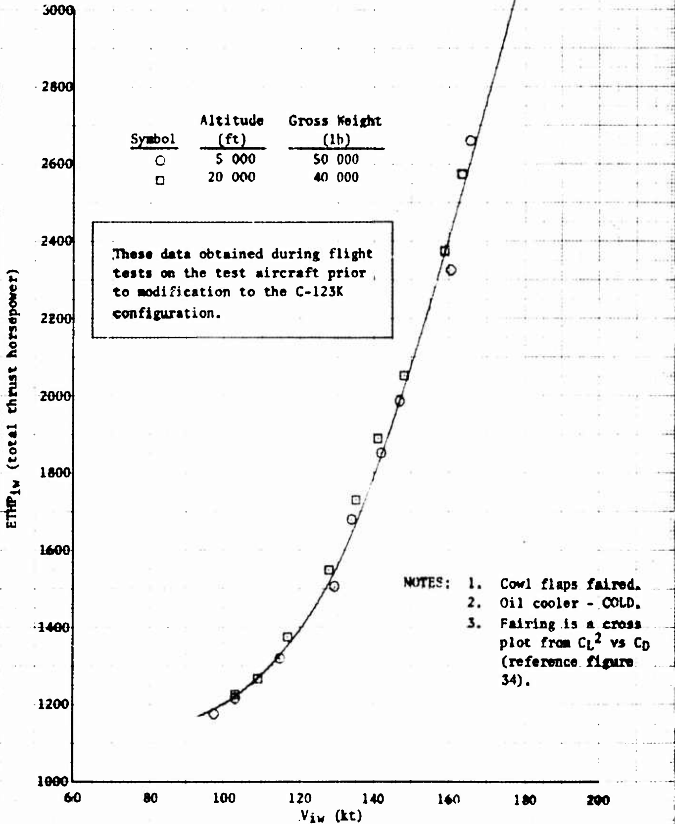
Figure 30. Level Flight Performance
