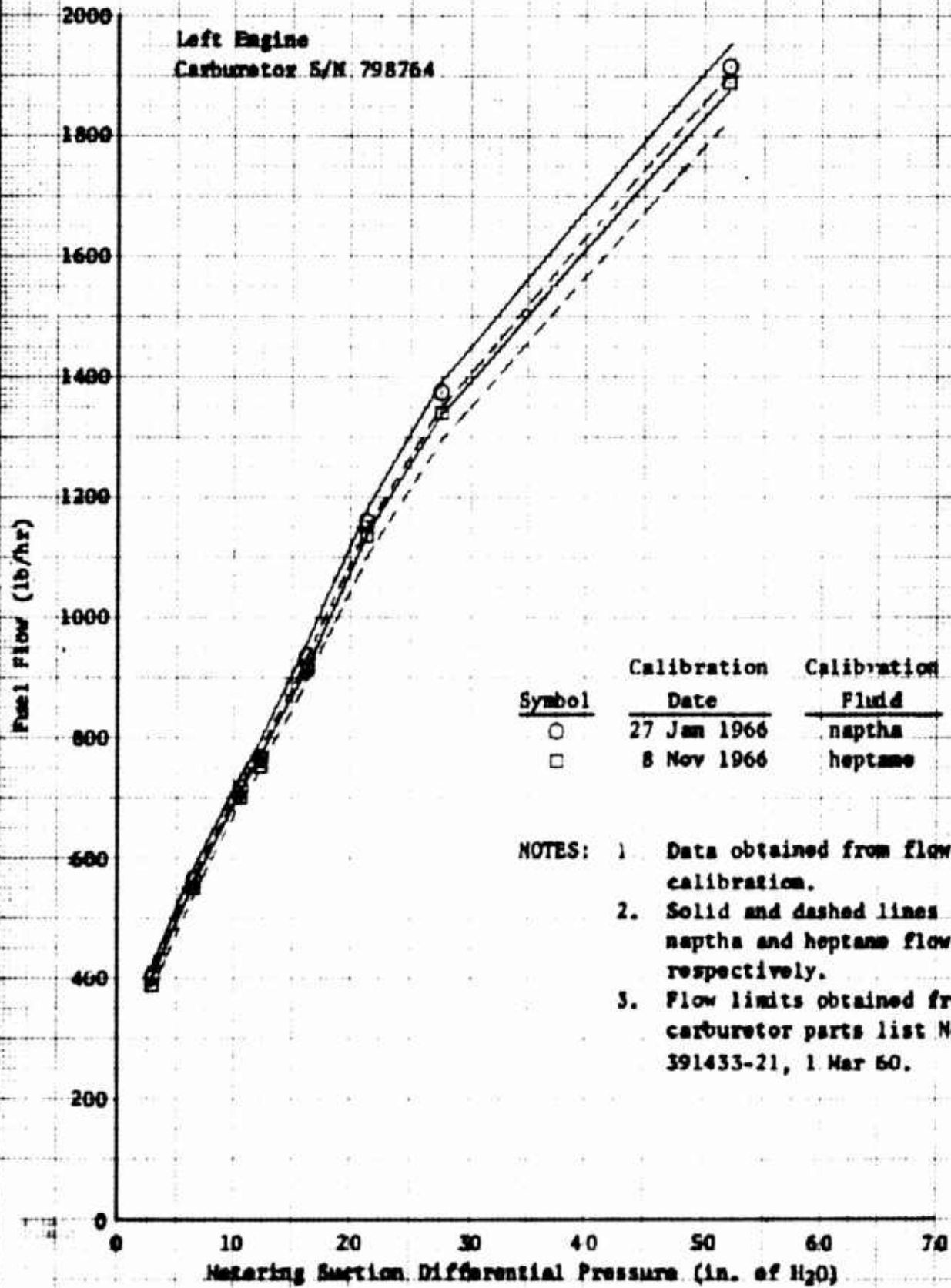
Figure 50. Carburetor Calibration
