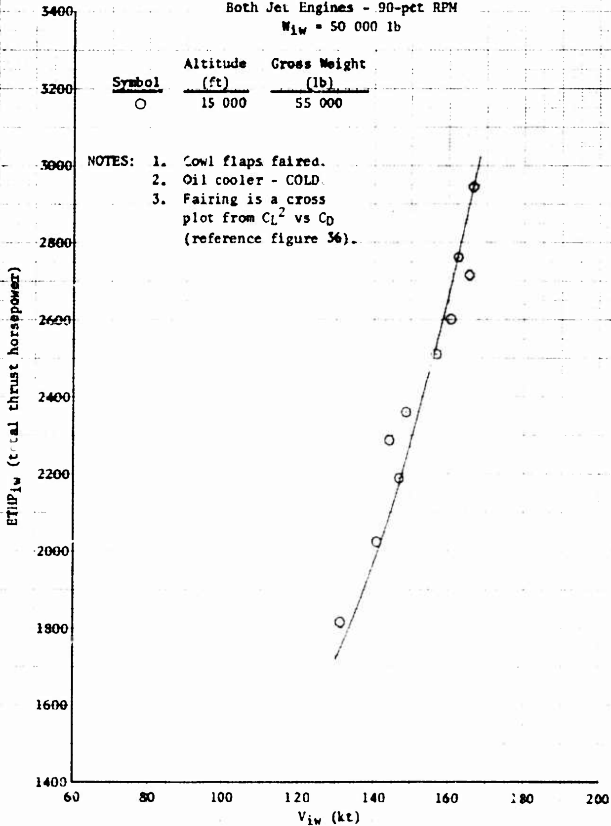
Figure 32. Level Flight Performance
