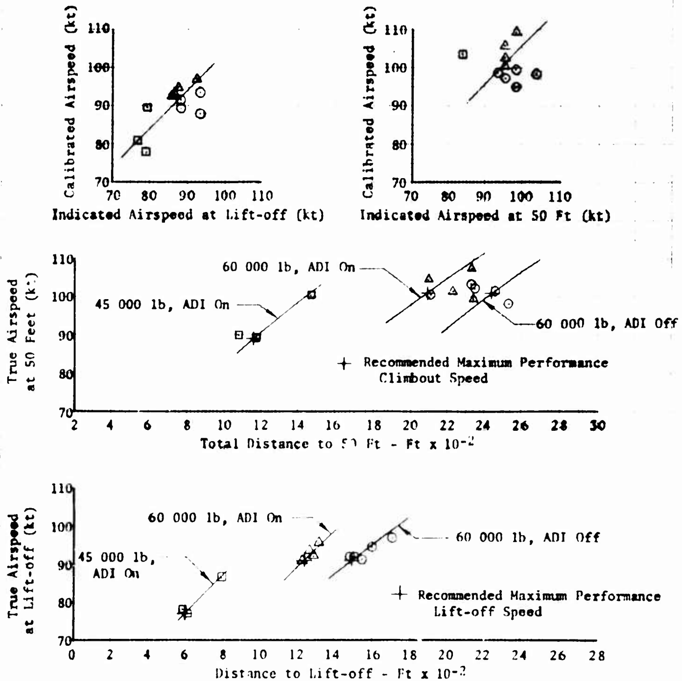
Figure 4. Takeoff Performance
