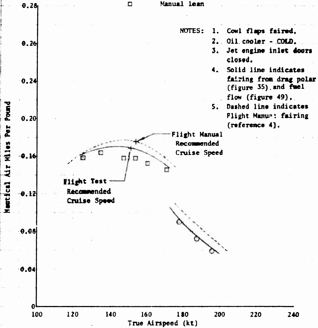
Figure 21. Specific Range
