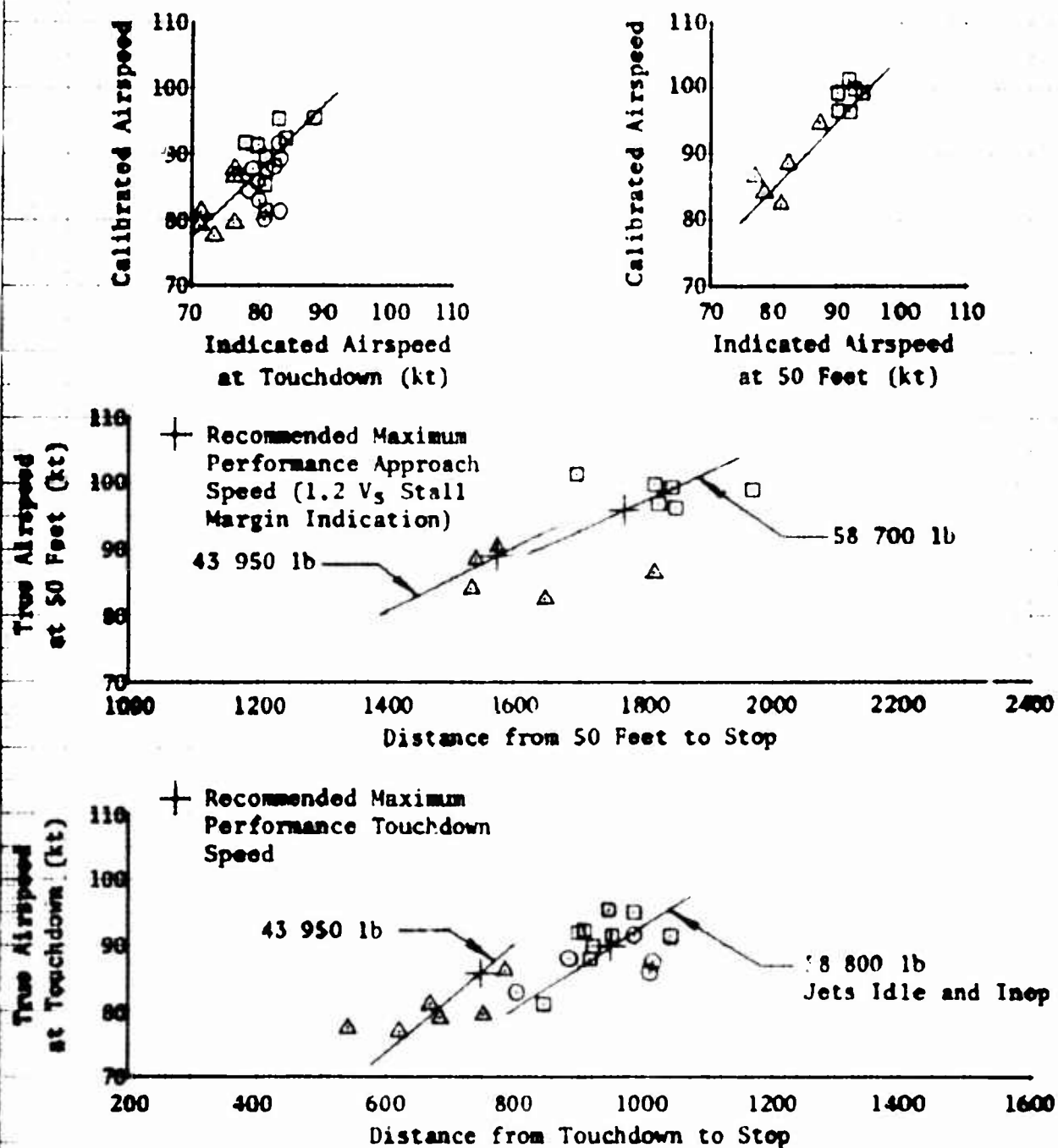
Figure 38. Landing Performance
