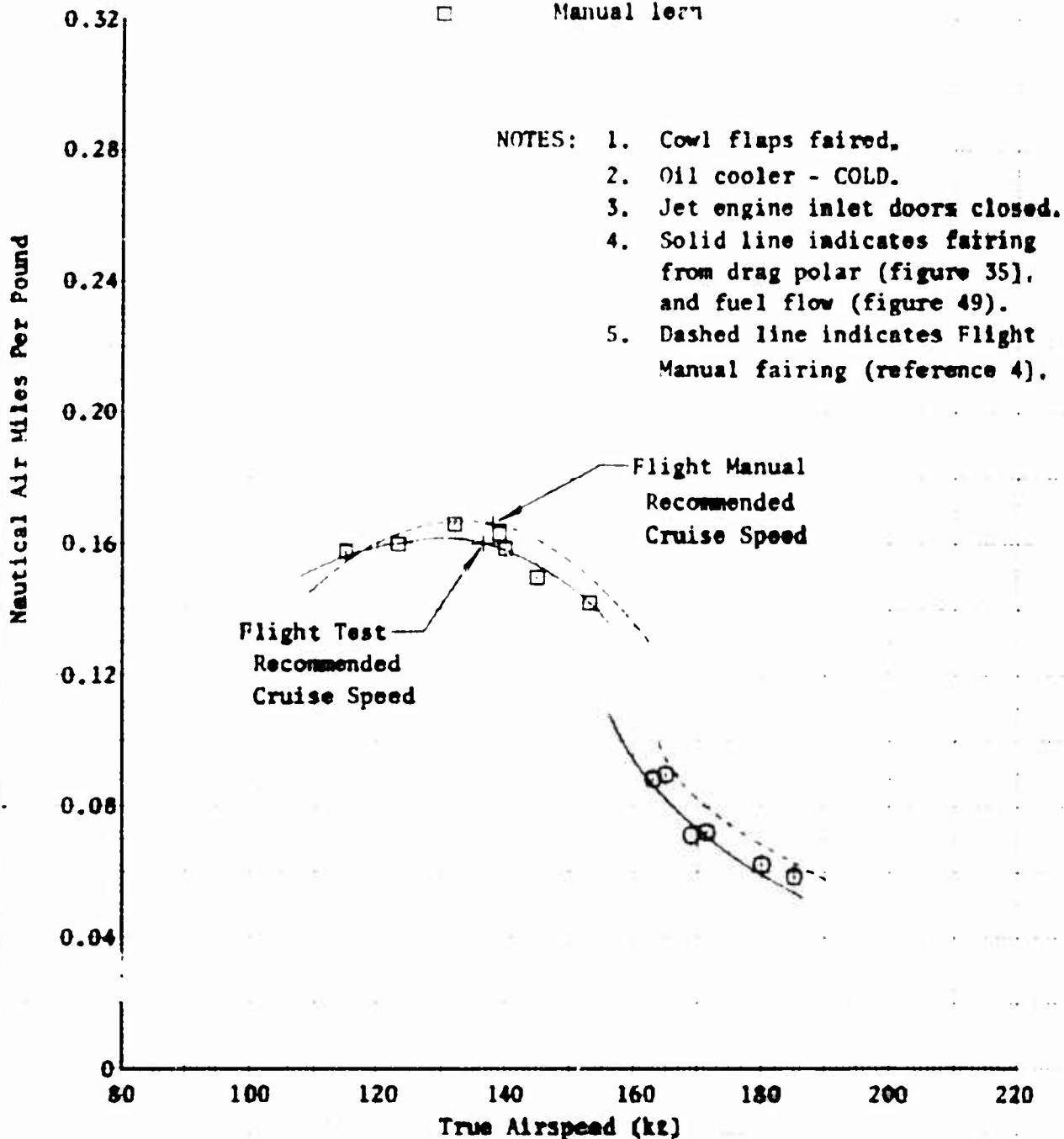
Figure 19. Specific Range
