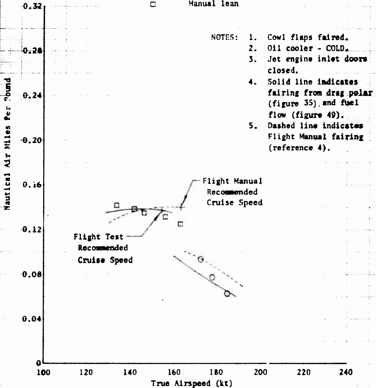
Figure 22. Specific Range
