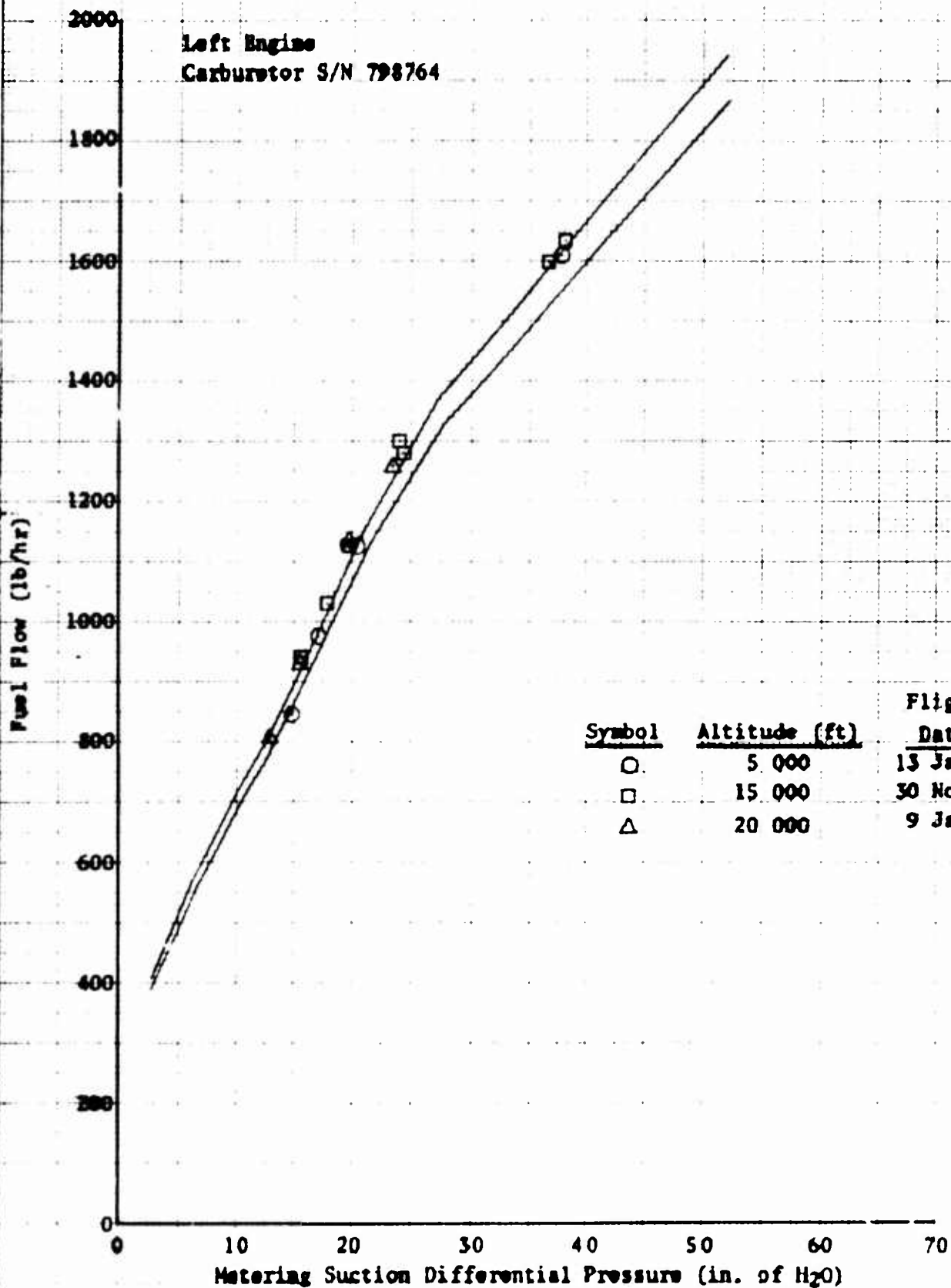
Figure 53. Carburetor Calibration
