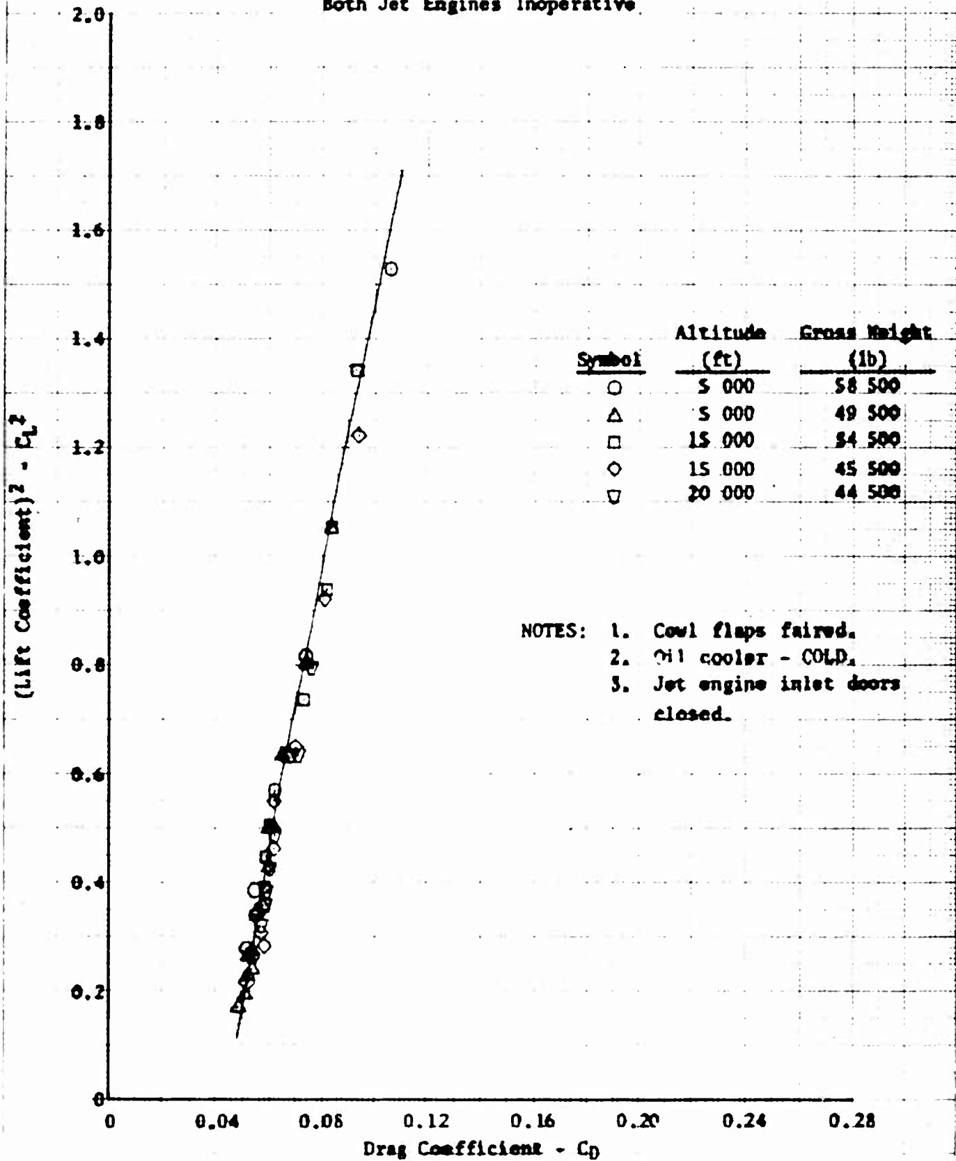
Figure 35. Drag Polar
