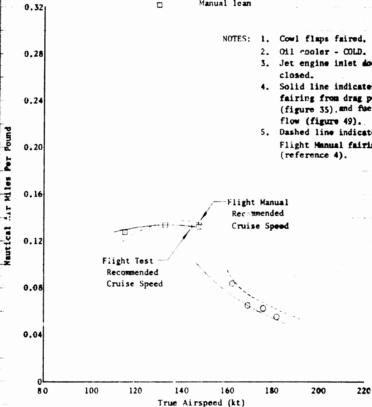
Figure 20. Specific Range
