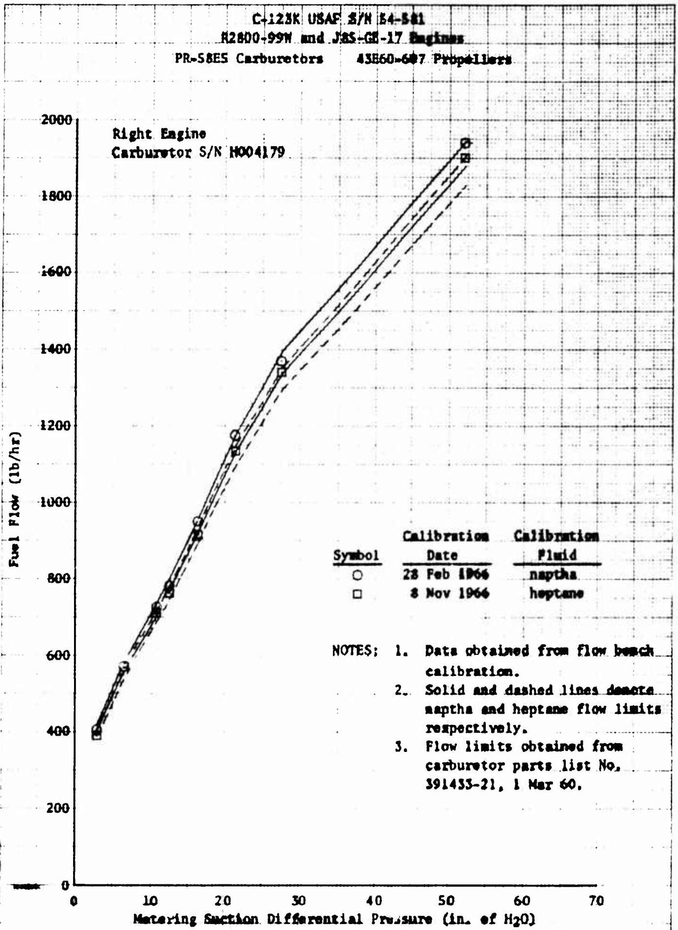
Figure 51. Carburetor Calibration
