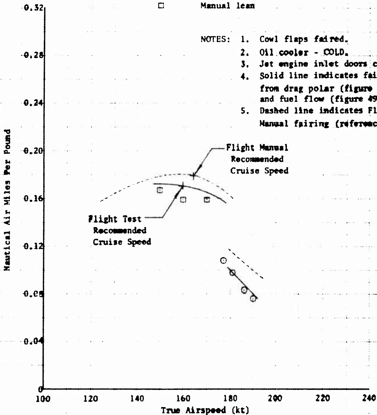
Figure 23. Specific Range
