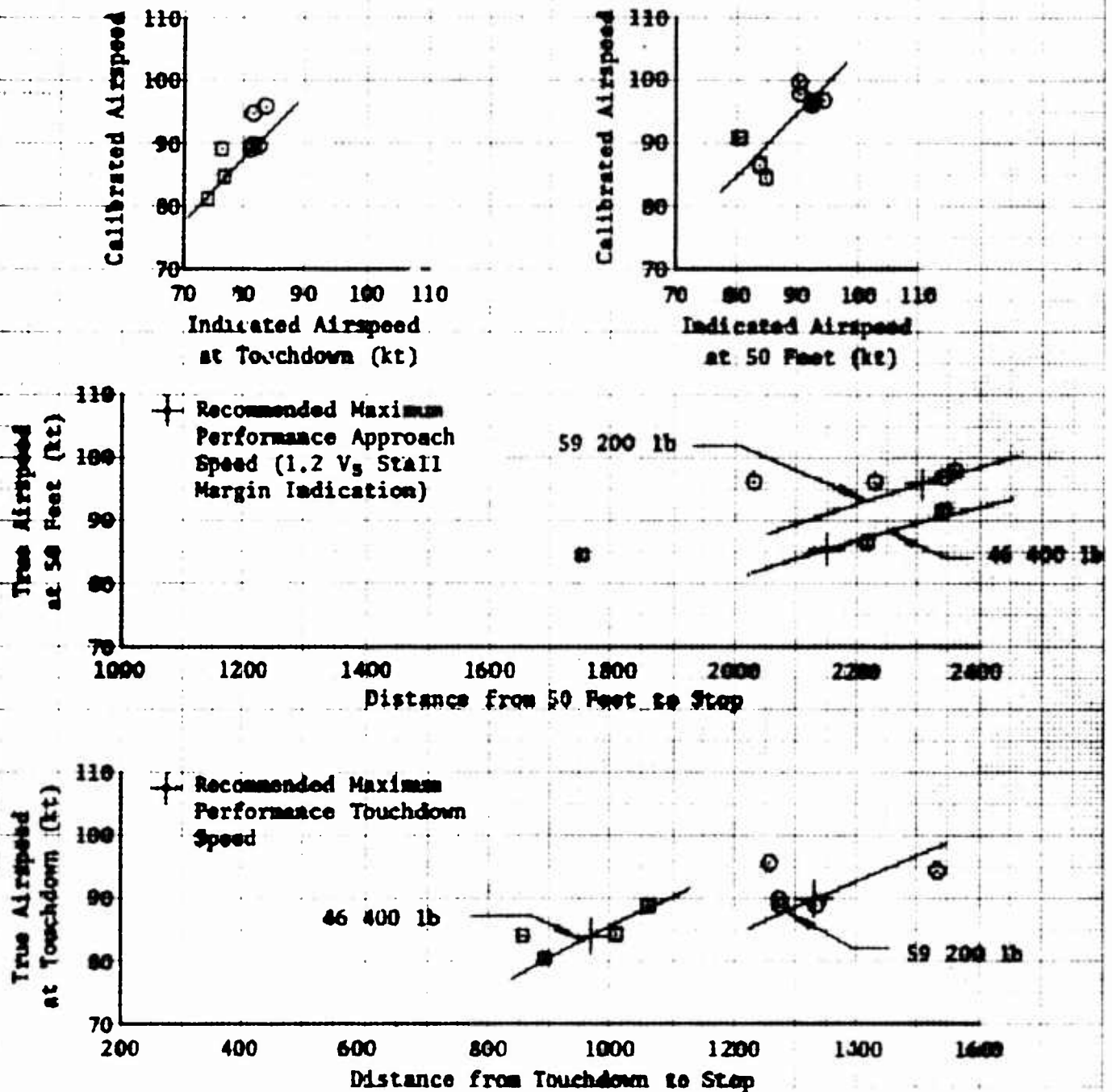
Figure 39. Landing Performance
