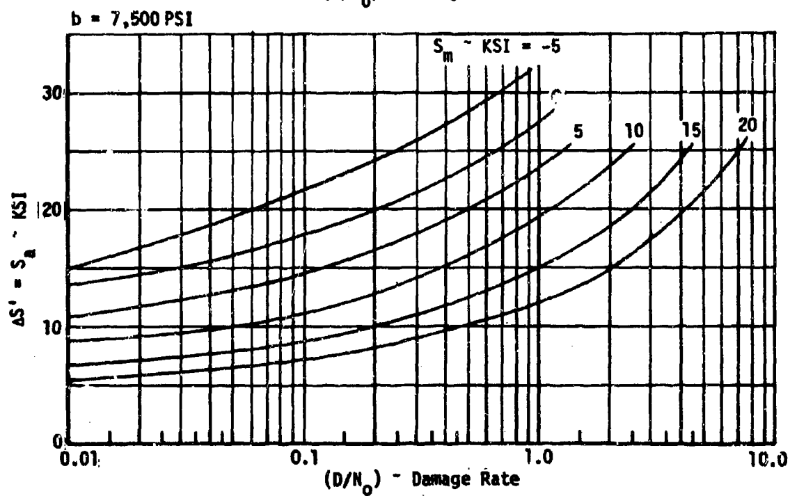
FIGURE 14. 7075-T6 ALUMINUM, K_f = 2.62 , DAMAGE RATES FOR \sum n = N_0 e^{-\Delta s/b} LOADS SPECTRA WITH CONSTANT S_m ; N_0 = 10^5 (Continued)
