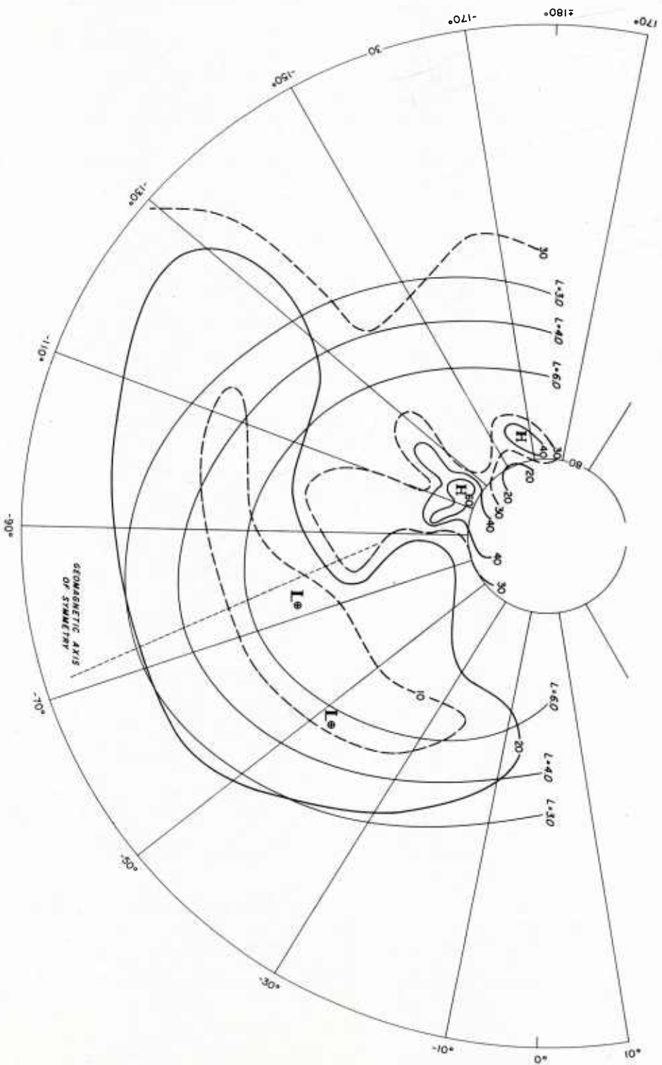
Figure 5. Horizontal cross section, at 700 km, of the polar ionospheric electron density ( \times 10^{-3} \text{ cm}^{-3} ) distribution on
