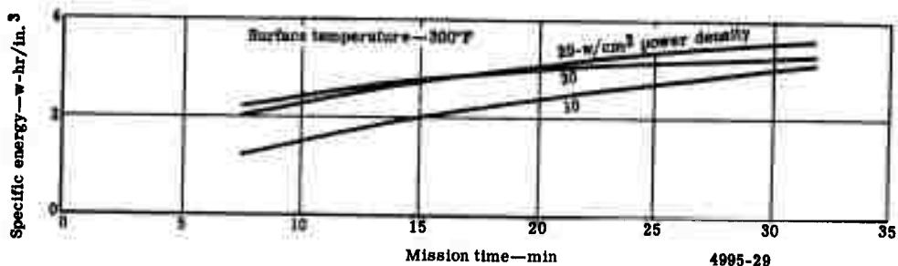
Figure 77. Volume energy density versus mission time at a 10- \text{kW}_e power level for the A-2 battery design.
