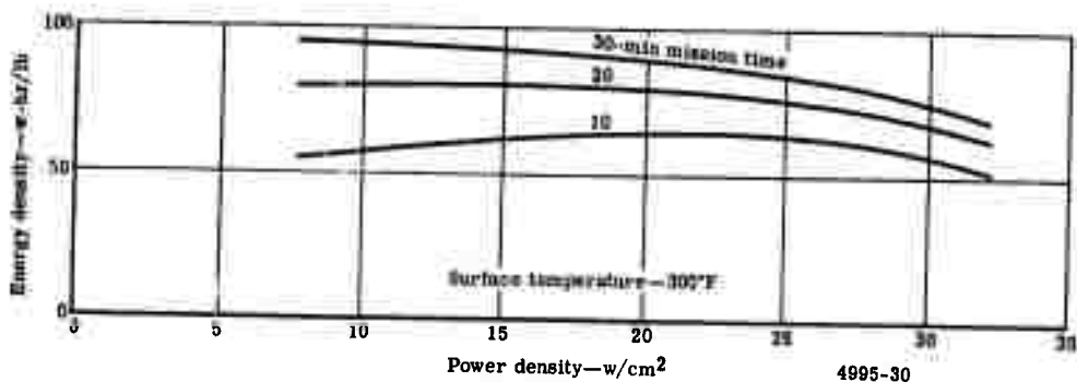
Figure 78. Weight energy density versus power density at a 10- \text{kW}_e power level for the A-2 battery design.
