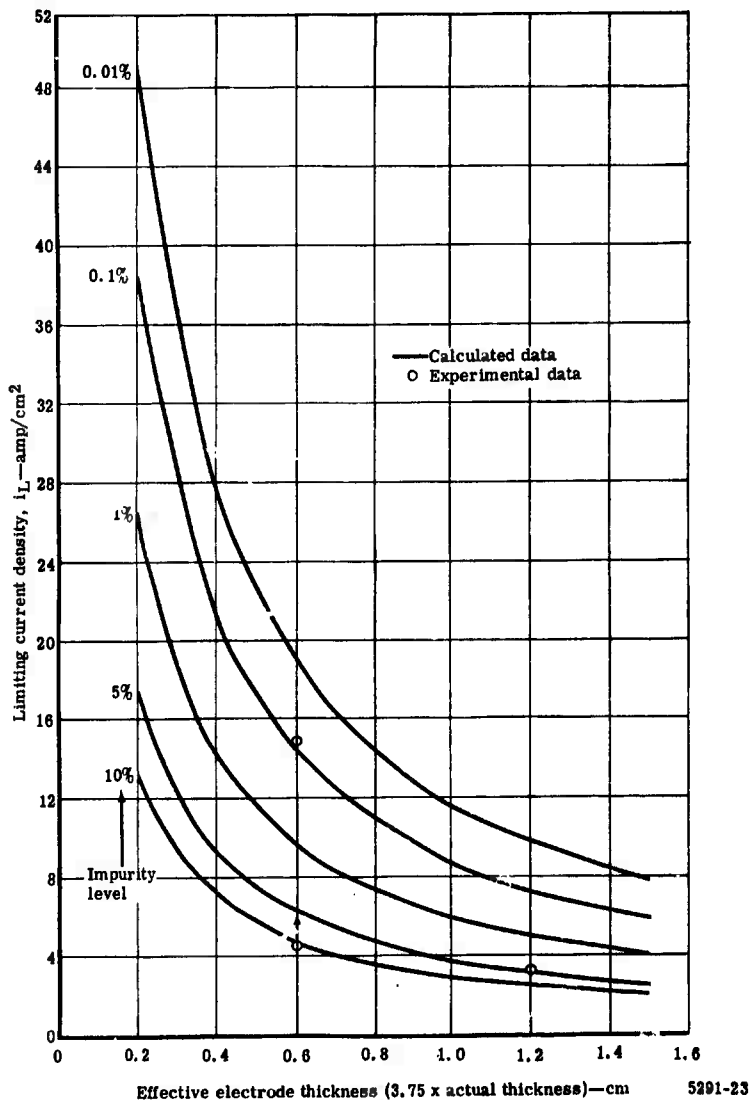
Figure 23. Limiting current density for Poc-Ax at 5 atm.
