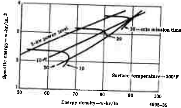
Figure 83. System characteristics of A-2 battery design at 20 w/cm 2 power density.
