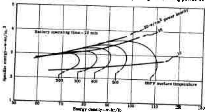
Figure 82. System characteristics of A-2 battery design at 10-kw e power level.
