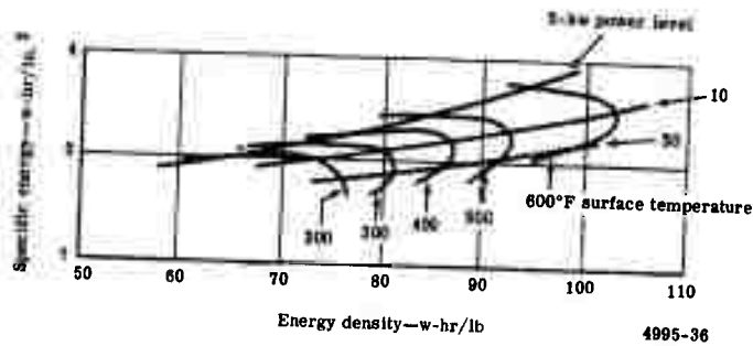
Figure 84. System characteristics of A-2 battery design at 20 w/cm 2 power density.
