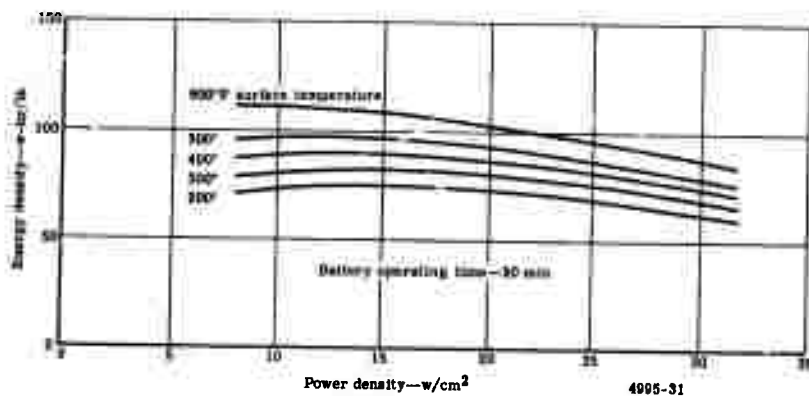
Figure 79. Weight energy density versus power density at a 10- \text{kW}_c power level for the A-2 battery design.
