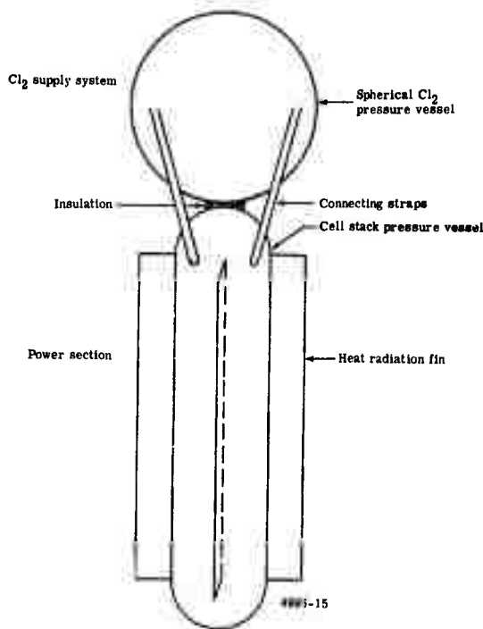
Figure 58. A-1 battery configuration.
