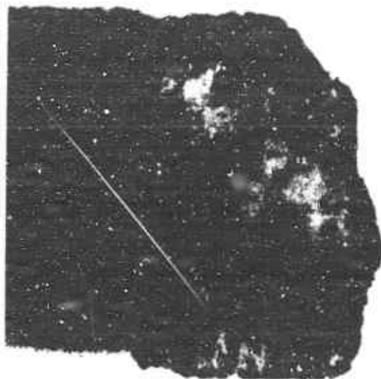
X104 Propellant 1014G Magnification: 15X
