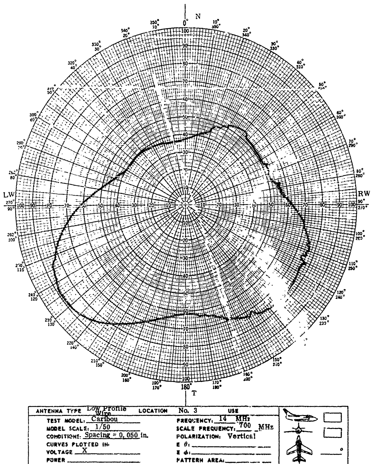
Fig. 39. Patterns of Low Profile Wire Antenna, 1/50 Caribou
