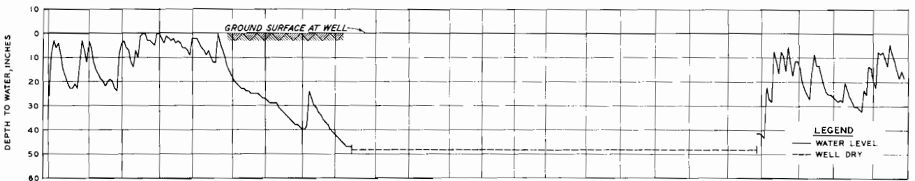
WATER TABLE OBSERVATION WELLS (4 FT)
