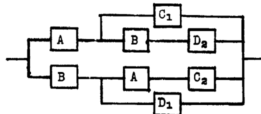
BOOLEAN OR LOGIC DIAGRAM
