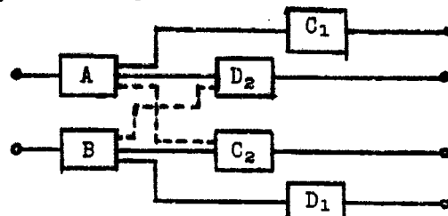
FUNCTIONAL DIAGRAM
