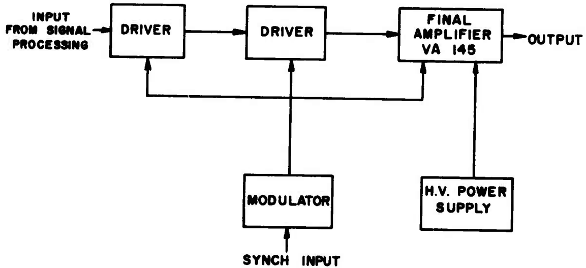
Figure 11. Interim Transmit System
