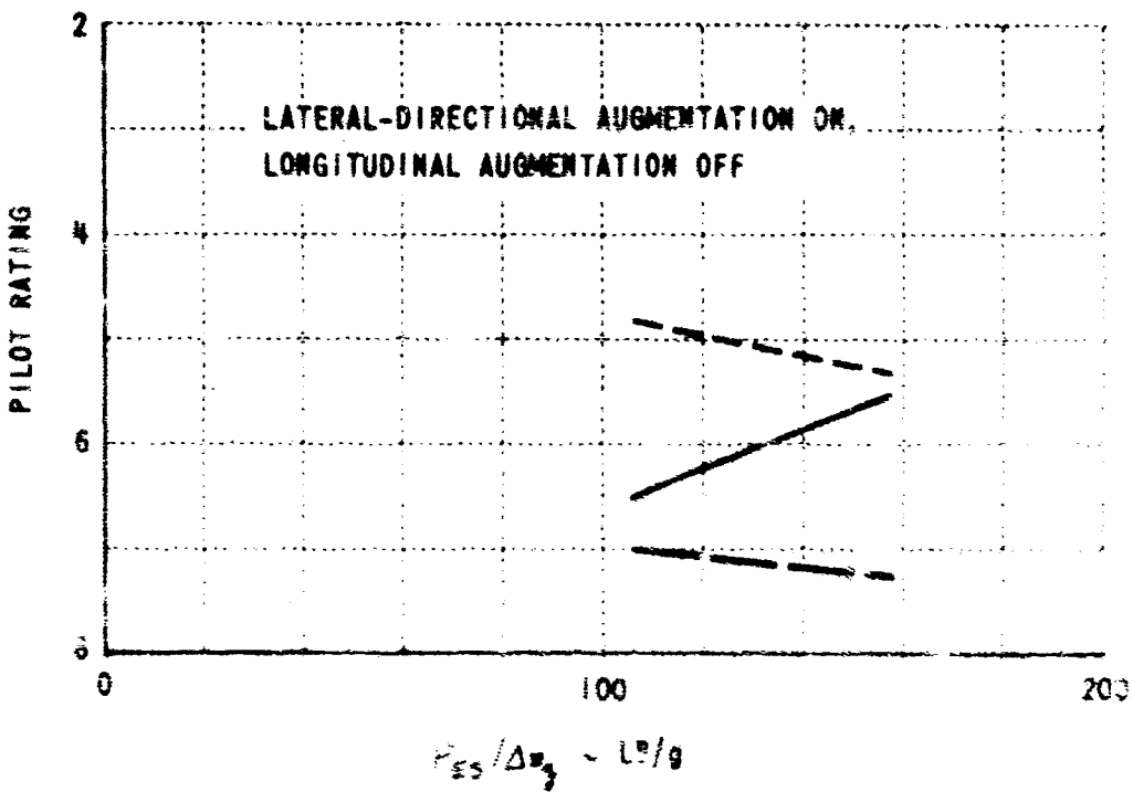
Figure 27 LONGITUDINAL EVALUATION -- COMPARISON OF INDIVIDUAL AVERAGED PILOT DATA
