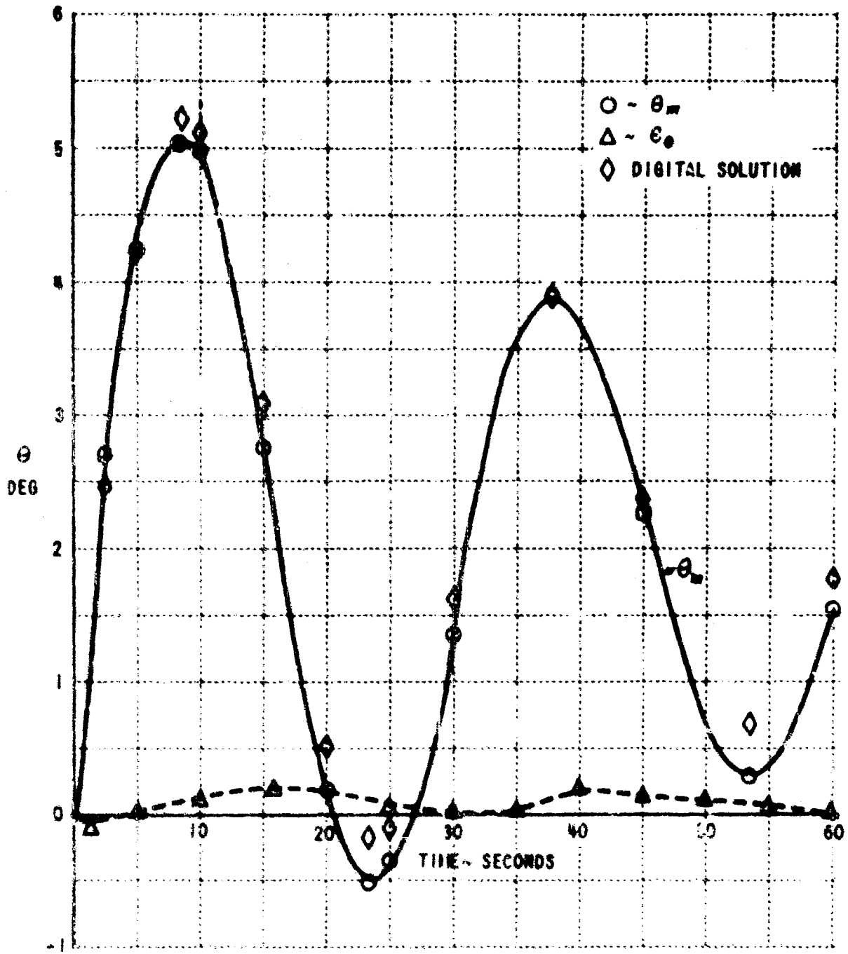
Figure 13 MODEL PITCH RESPONSE AND AIRPLANE PITCH RESPONSE ERROR TO 3^\circ \delta_e STEP COMMAND TO MODEL -- AUGMENTED CASE
