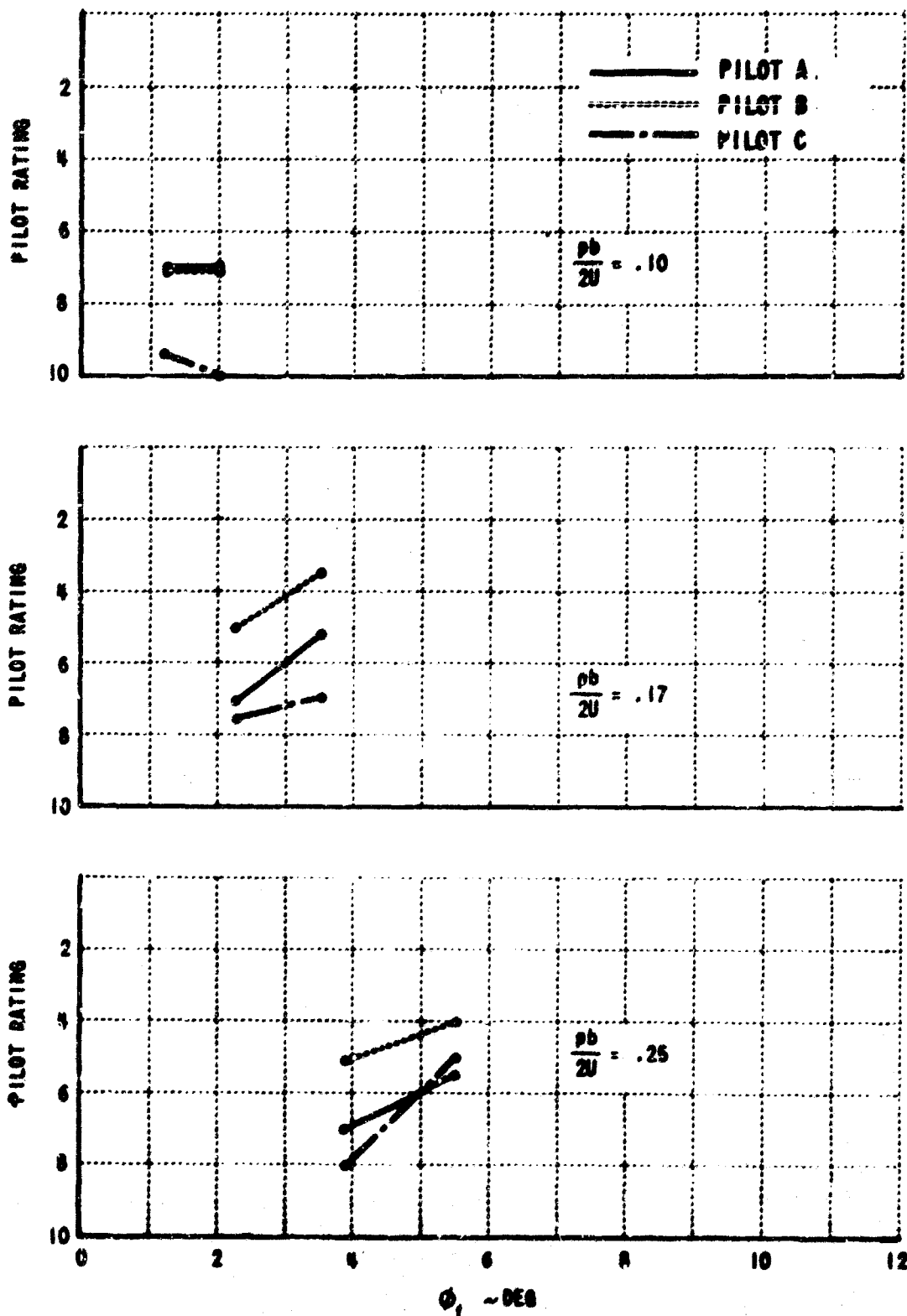
Figure 24 PILOT COMPARISON OF LATERAL-DIRECTIONAL EVALUATION UNAugMENTED CONFIGURATION
