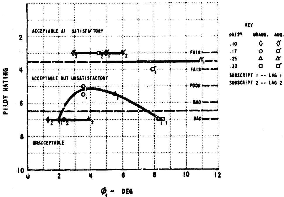
Figure 29 LATERAL-DIRECTIONAL EVALUATION -- PILOT A, EFFECT OF \phi_1 RATINGS INCLUDE LONGITUDINAL CHARACTERISTICS
