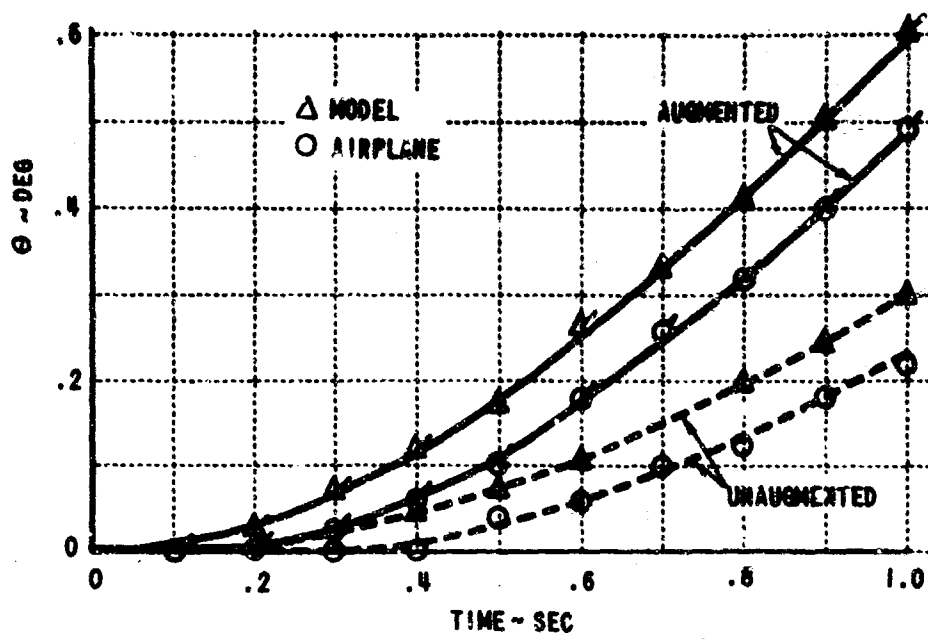
Figure 16 INITIAL \Theta RESPONSE COMPARISON TO 3^\circ \delta_e STEP COMMAND
