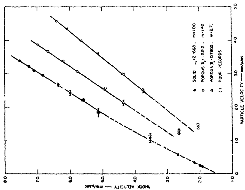
FIG. 5 SHOCK VELOCITY vs PARTICLE VELOCITY FOR TEFLON
