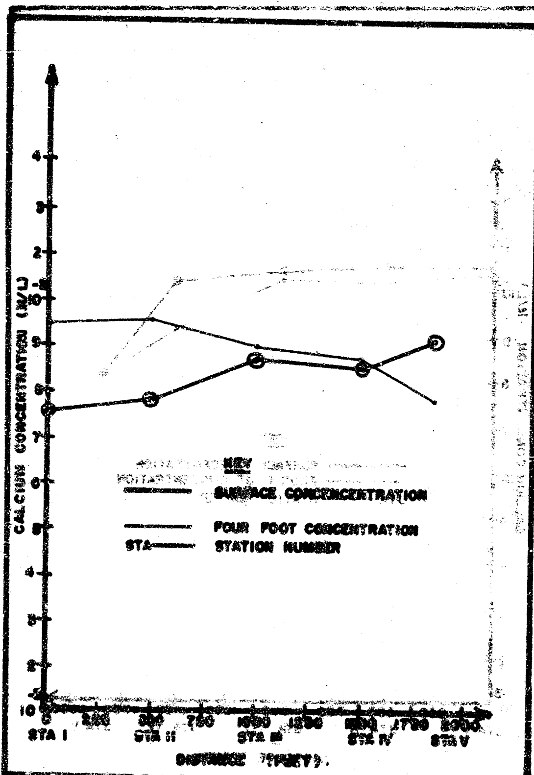
PLATE 10. CALCIUM DISTRIBUTION IN TERRACE A, FIELD TRIP 2, AT FIVE POINTS INTO THE RED STRATA
