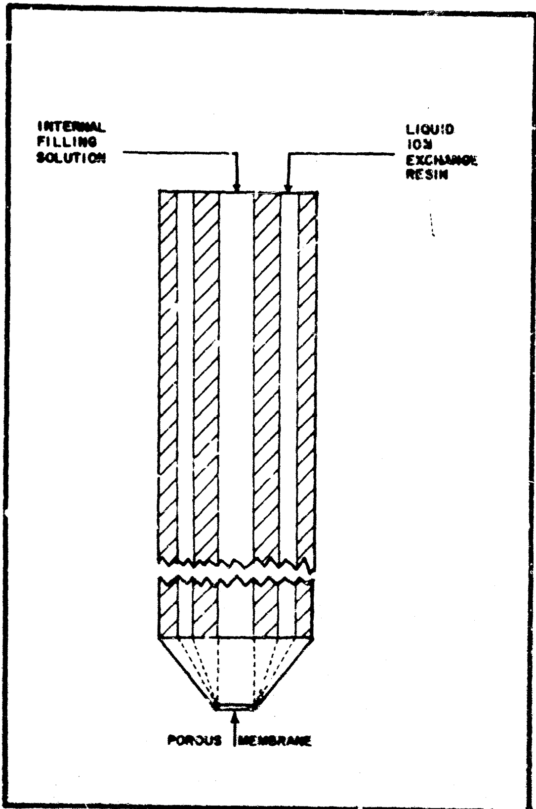
PLATE 3. CROSS SECTION OF CALCIUM ELECTRODE.
