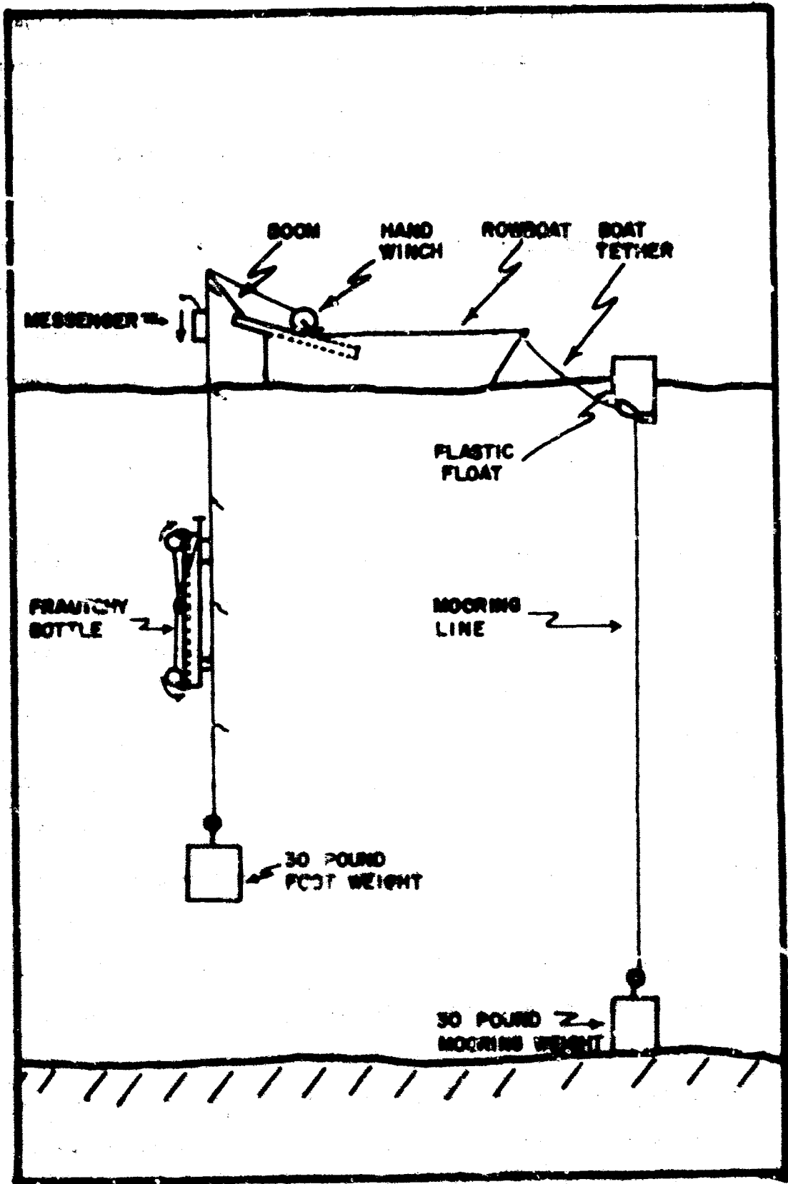
PLATE 2. SAMPLING SYSTEM.
