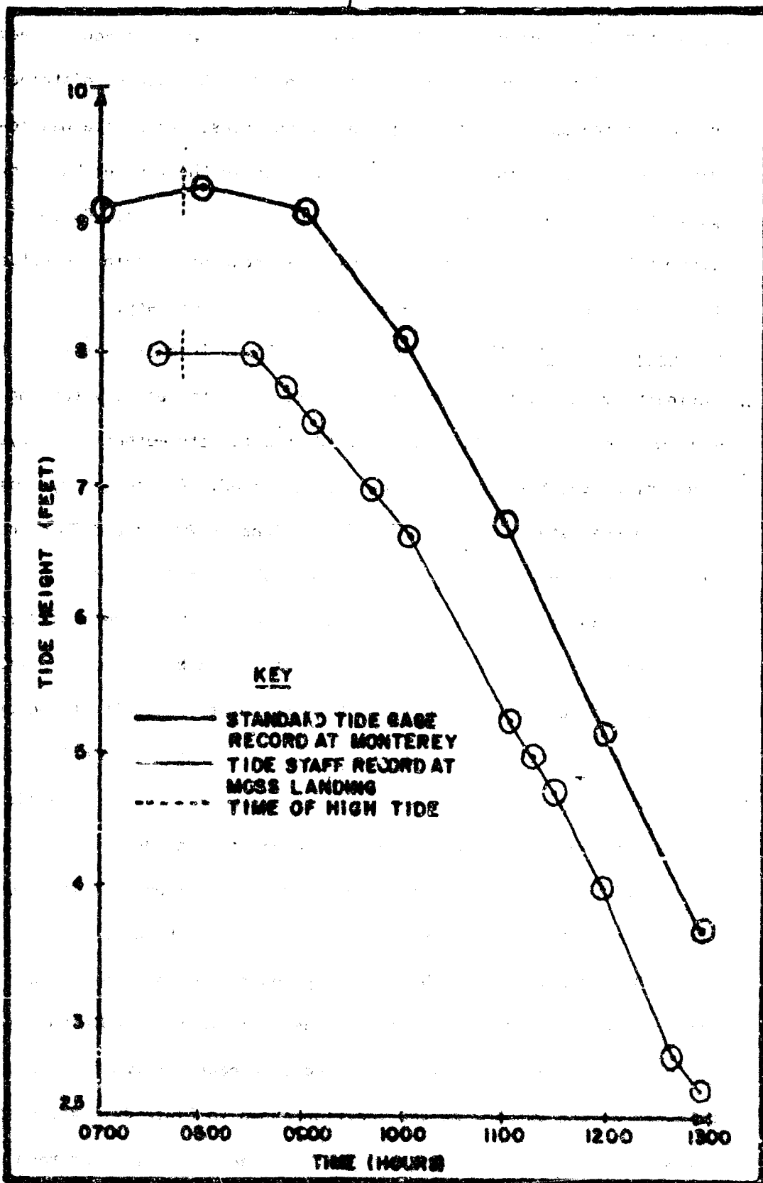
PLATE 2A. COMPARISON OF EBB TIDAL STAGE MOVEMENT RATES BETWEEN MONTEREY AND MOSS LANDING.
