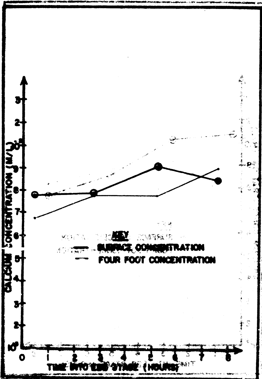
PLATE 8. CONCENTRATION VARIATION, STATION V, FIELD TRIP II.
