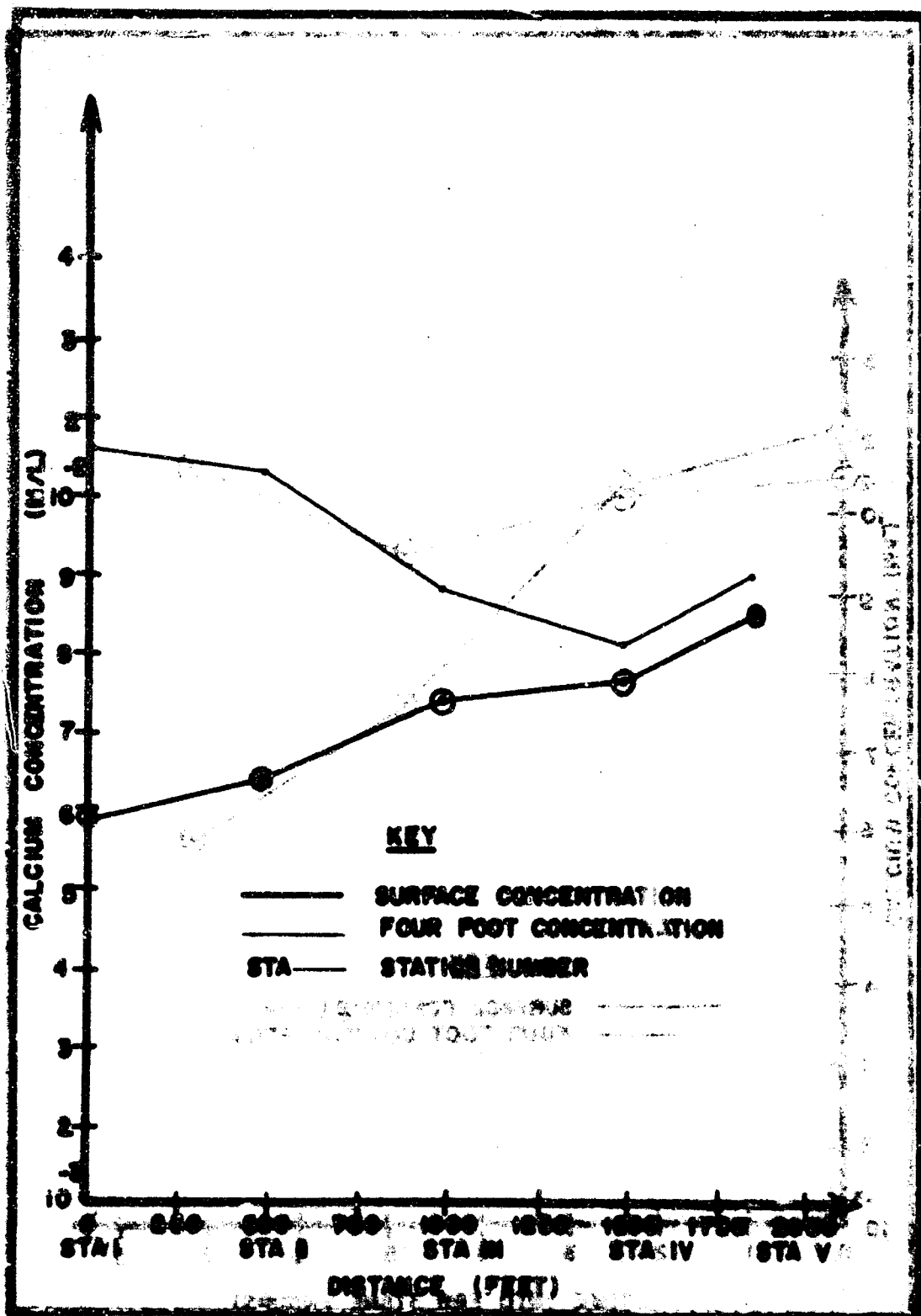
PLATE II. CALCIUM DISTRIBUTION IN TRIBUTARY A, FIELD TRIP II, AT SEVEN HOURS INTO THE EGG STAGE.
