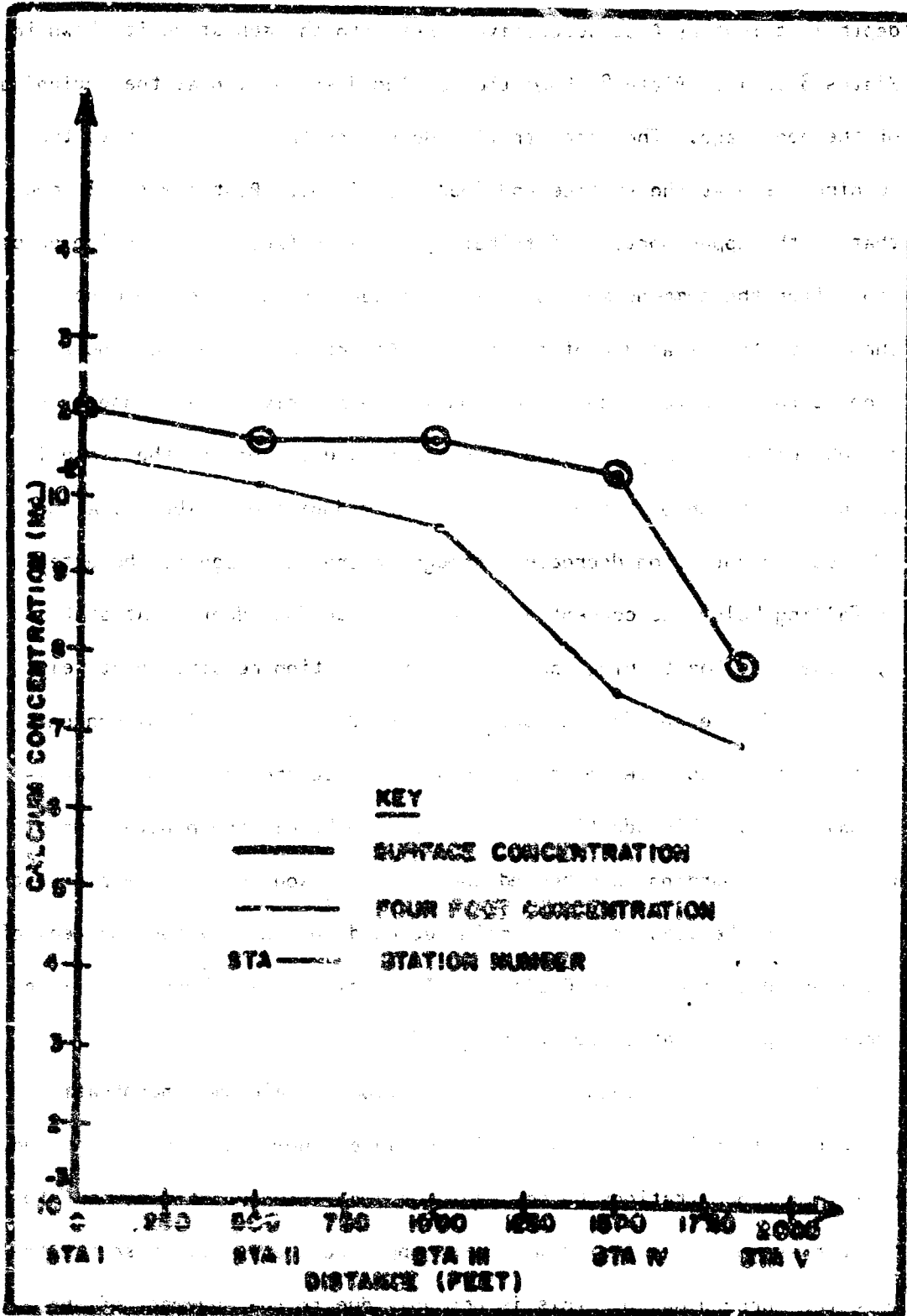
PLATE B. CALCIUM DISTRIBUTION IN TRIBUTARY A, FIELD TRIP N, AT COMMENCEMENT OF EGG STAGE.
