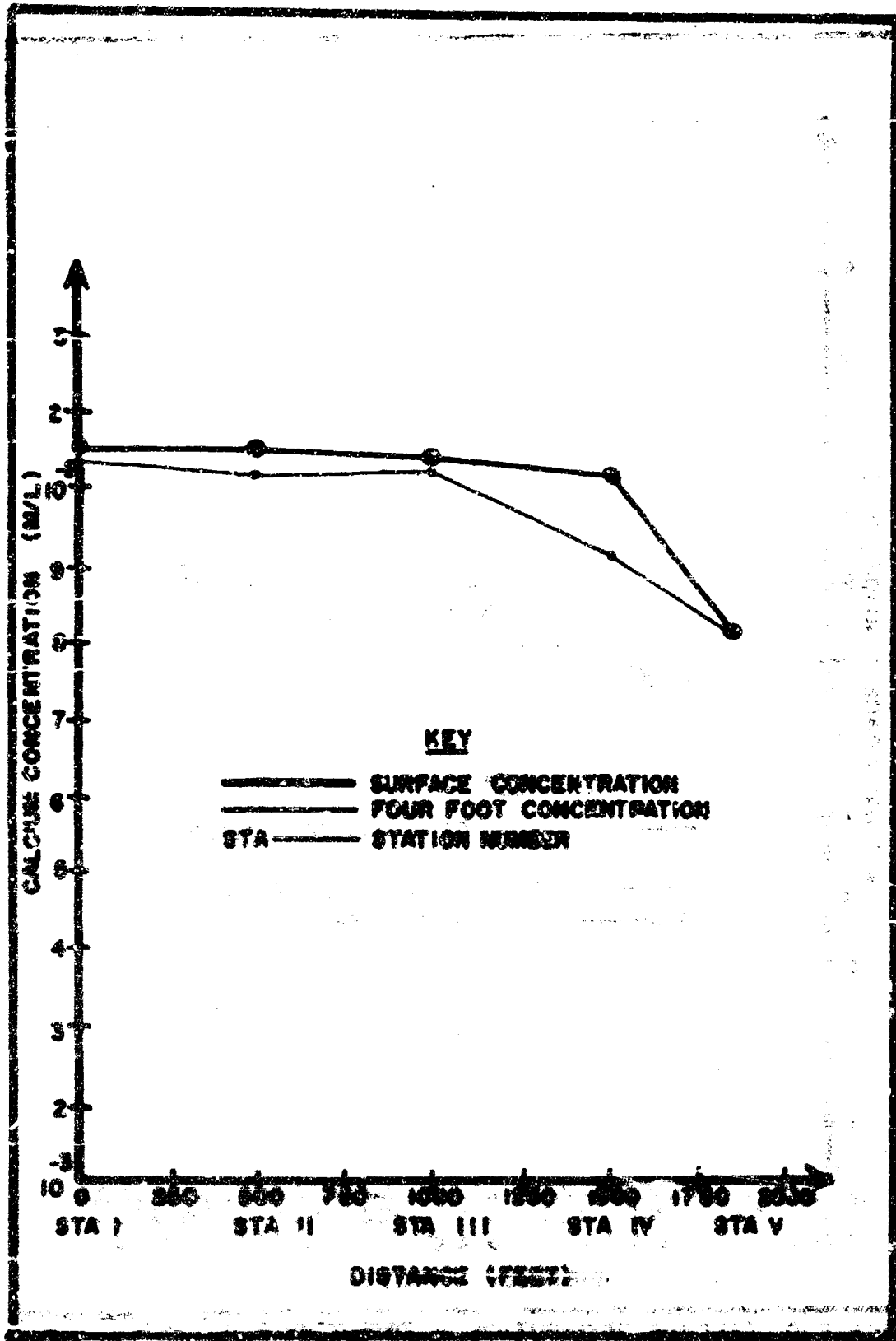
PLATE 9. CALCIUM DISTRIBUTION IN TRIBUTARY A AT 2.5 HOURS INTO THE ESB STAGE, FIELD TRIP II.
