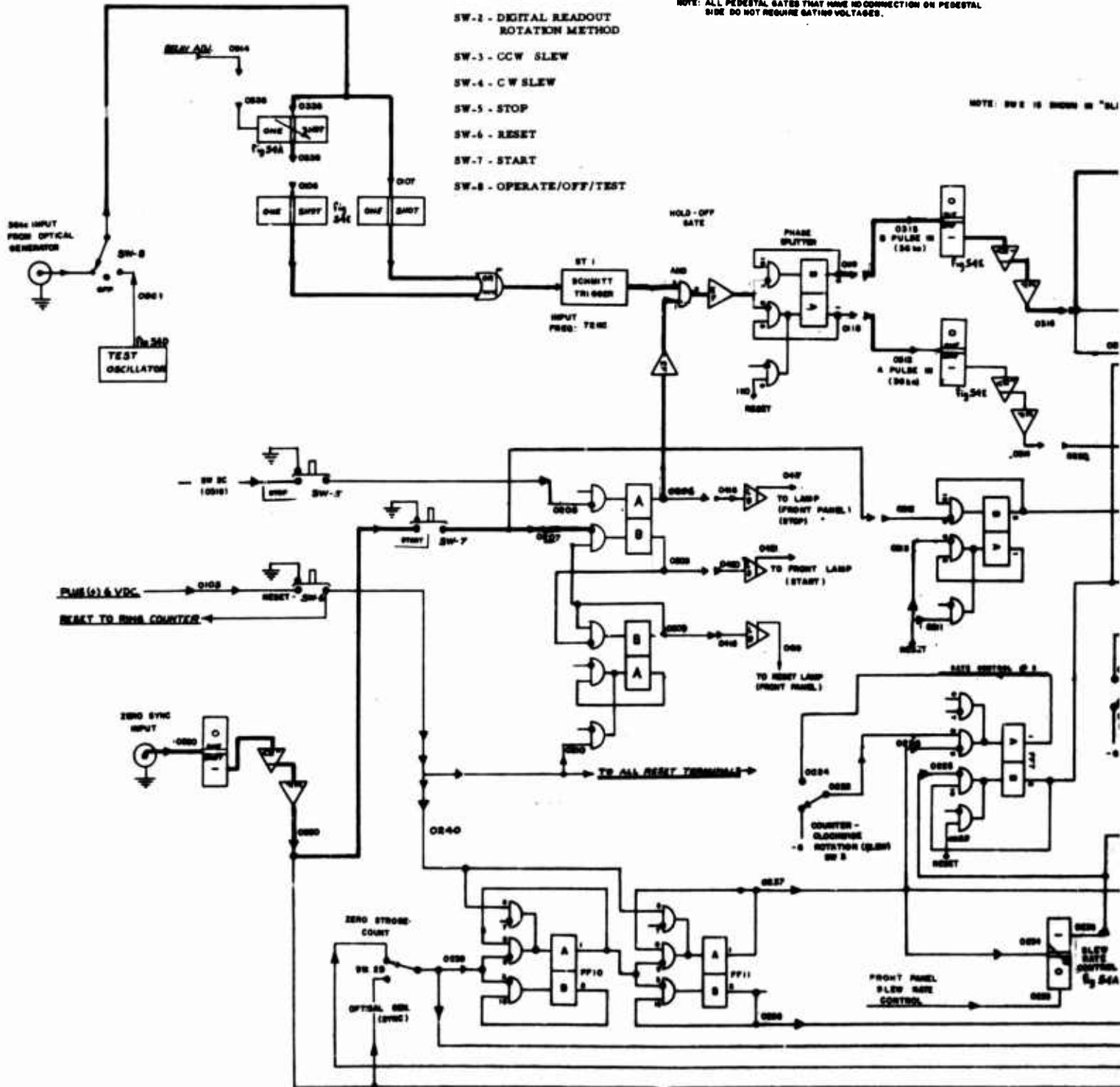
FIGURE 23. BLOCK DIAGRAM OF MASTER CONTROL SYSTEM
