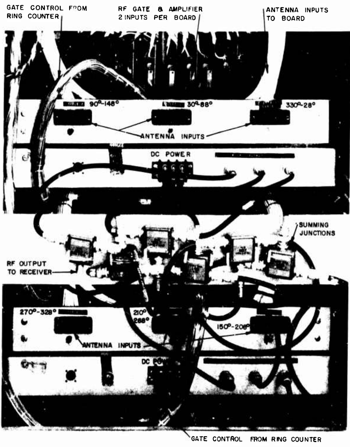
FIGURE 27. R. F. CHASSISS - REAR VIEW
