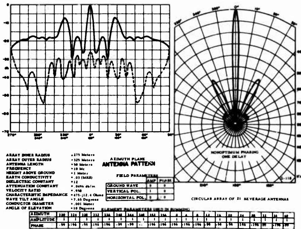
FIGURE 36. NONOPTIMALLY PHASED ARRAY PATTERN WITH ONE DELAY AT 10 MHz - 21 ANTENNAS
