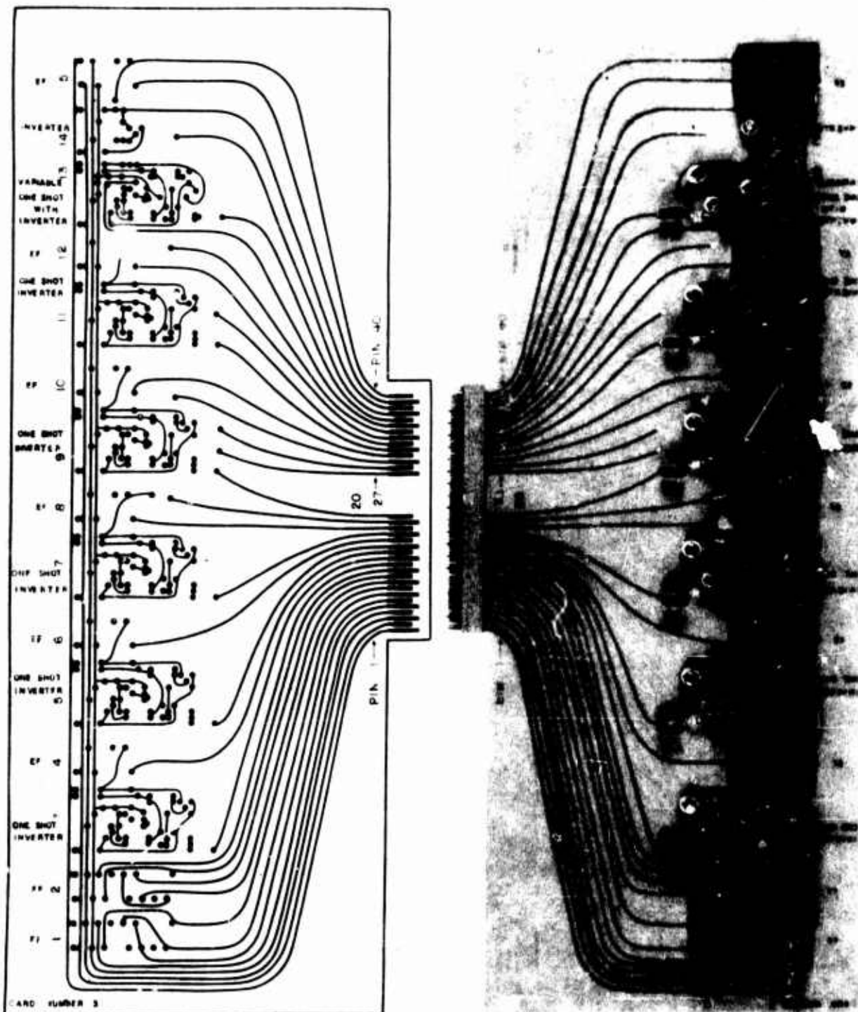
FIGURE 47. LOGIC BOARD NO. 3 - MASTER CONTROL CHASSIS
