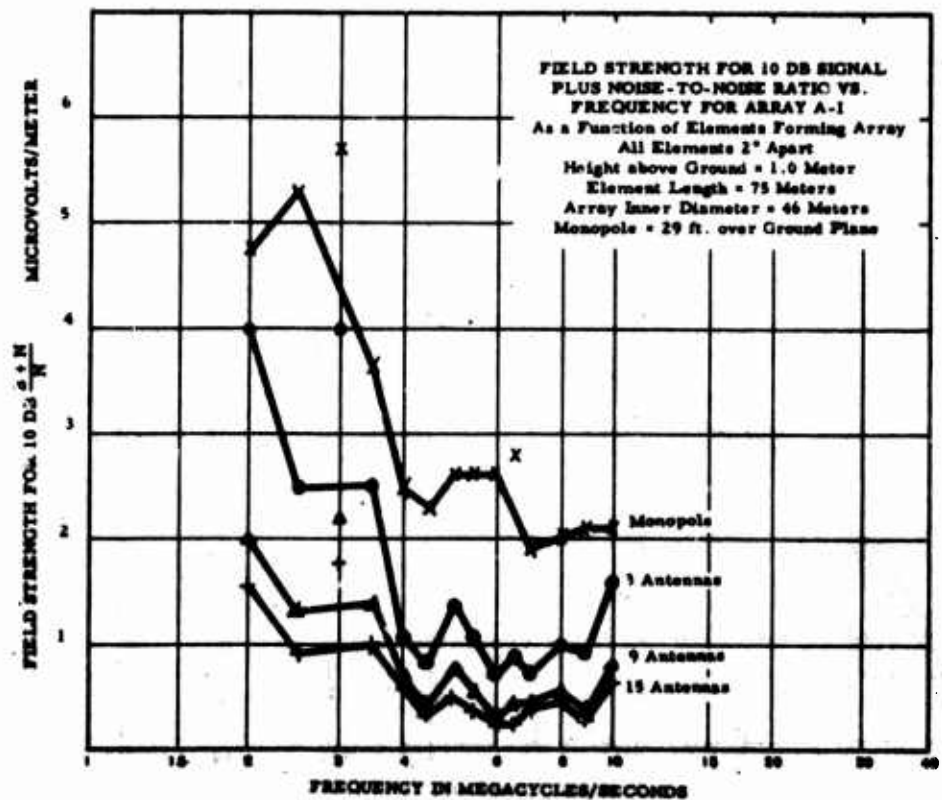
FIGURE 25. ARRAY SENSITIVITY
