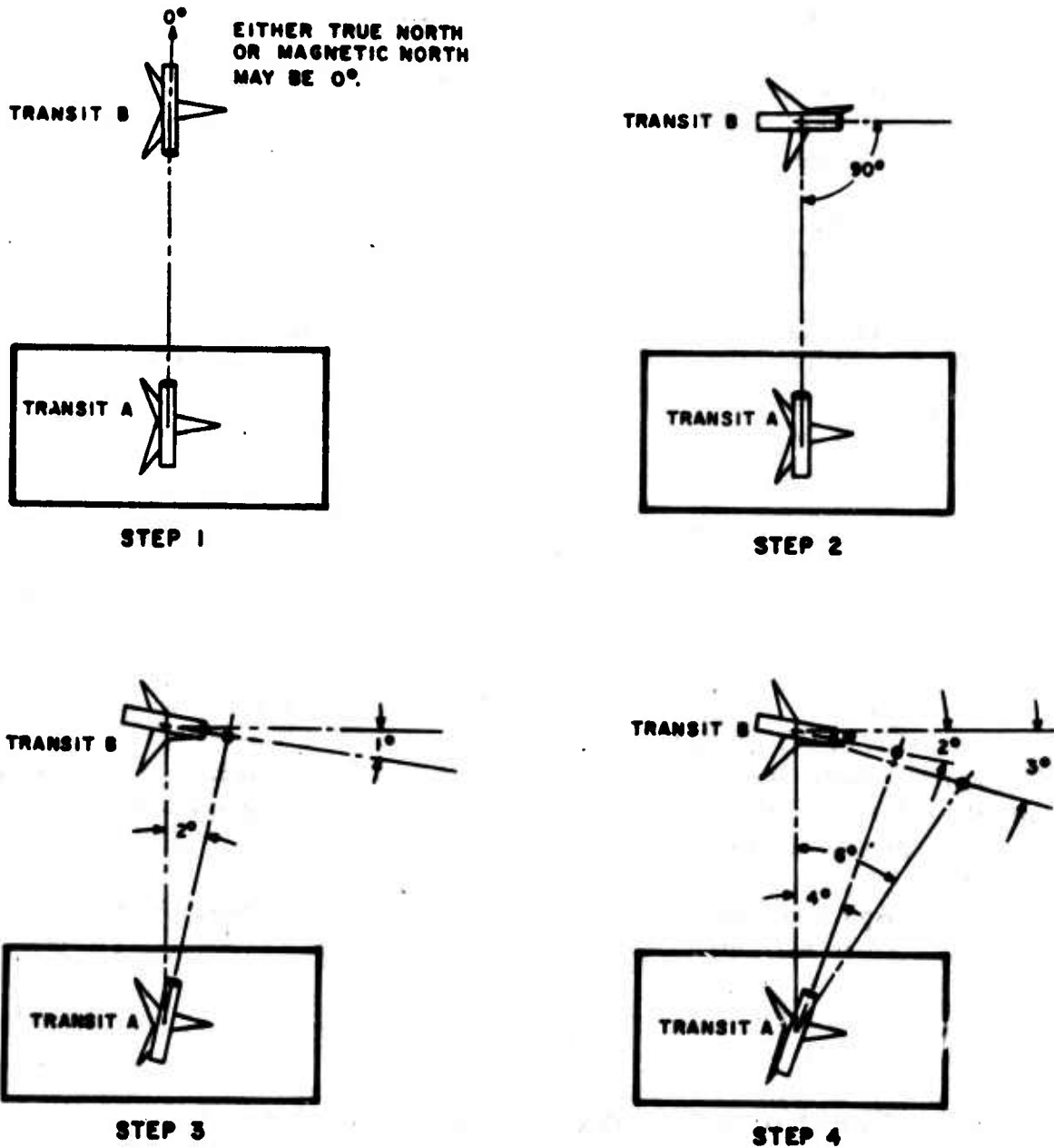
FIGURE 21. ALIGNMENT PROCEDURES FOR TWO-TRANSIT TECHNIQUE
