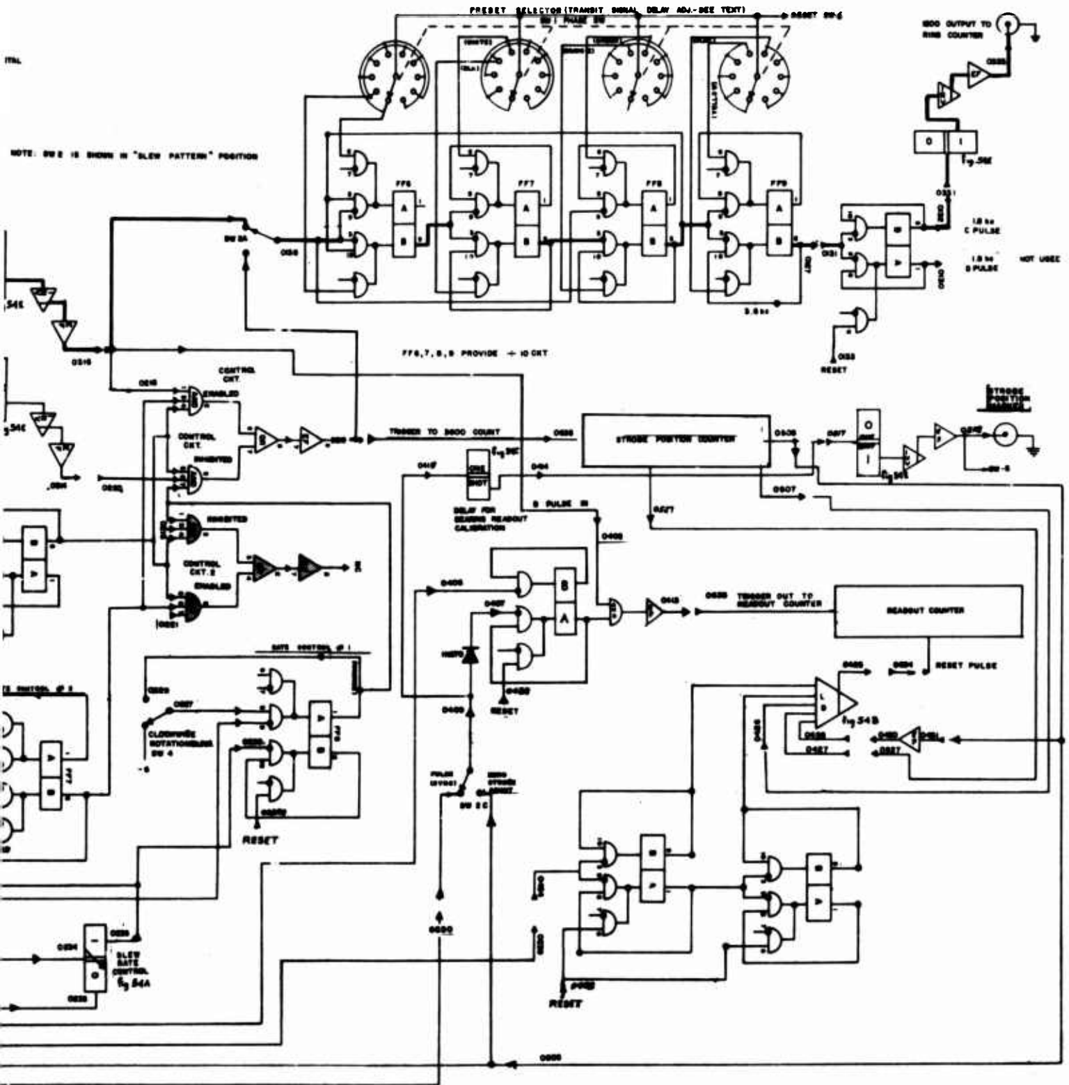
GRAM OF MASTER CONTROL CHASSIS
