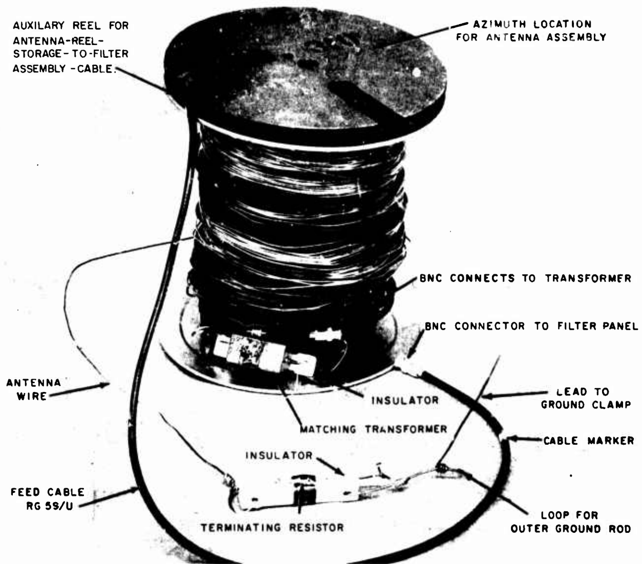
FIGURE 13. COMPLETE ANTENNA ASSEMBLY
