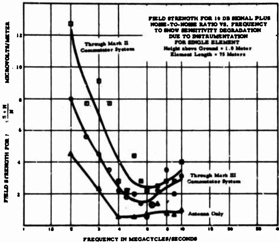
FIGURE 26. SENSITIVITY DEGRADATION DUE TO COMMUTATOR
