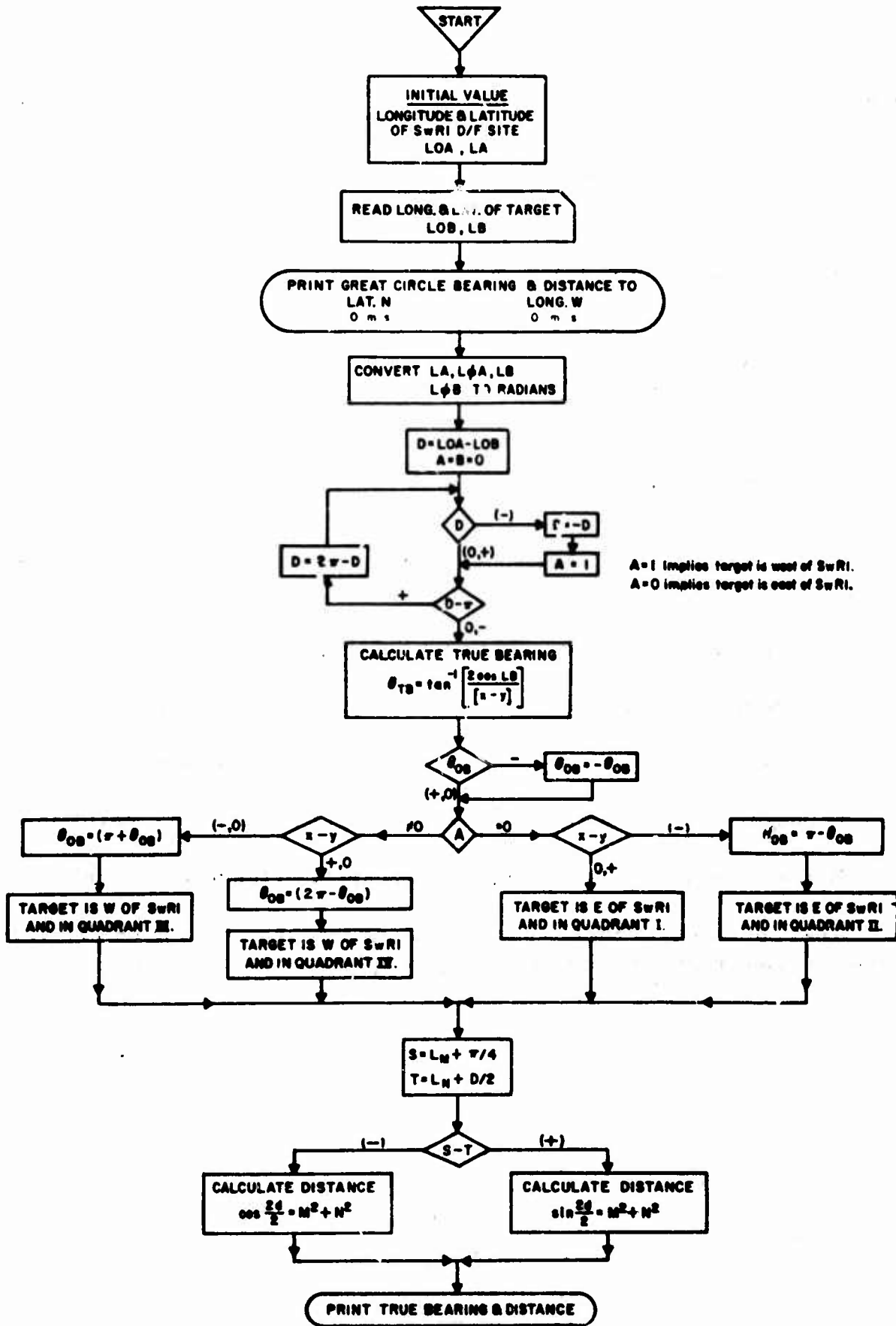
COMPUTER PROGRAM FOR TRUE BEARING CALCULATIONS
