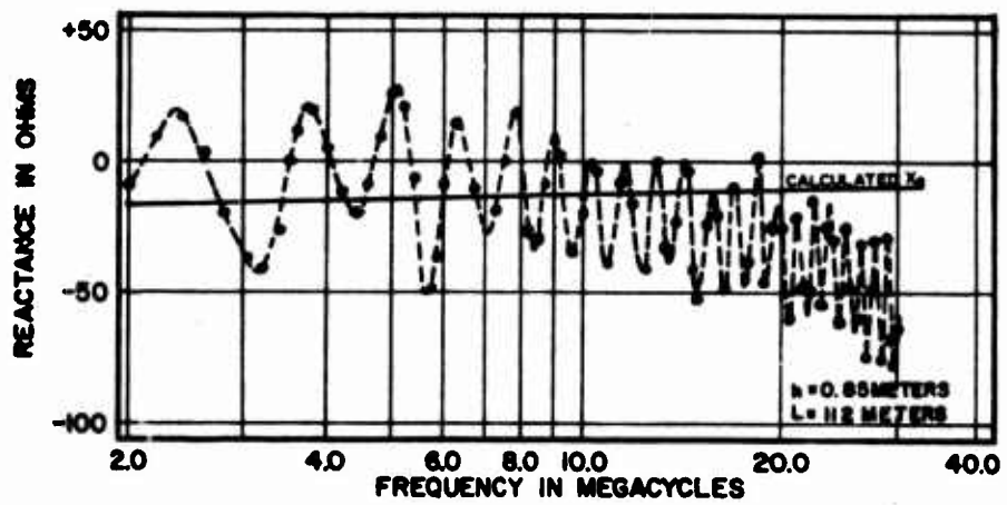
FIGURE 4. IMPEDANCE VS FREQUENCY OF SINGLE BEVERAGE ANTENNA
