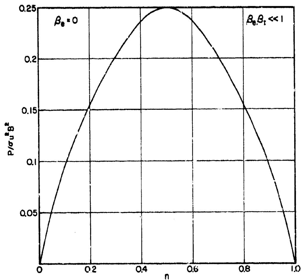
FIGURE 5. Power and Efficiency for Segmented Electrode Generator
