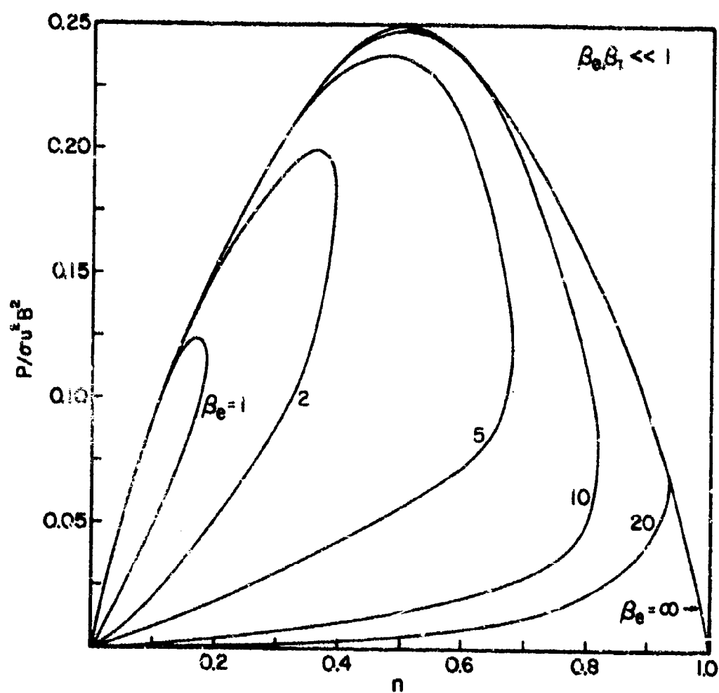
FIGURE 6. Power and Efficiency for Hall Generator
