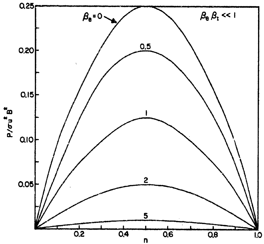
FIGURE 4. Power and Efficiency for Continuous Electrode Generator
